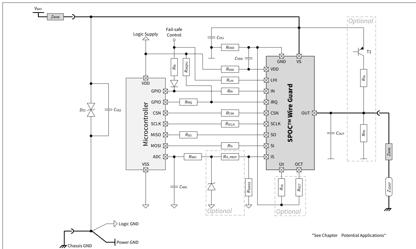
Figure 4 Application diagram
