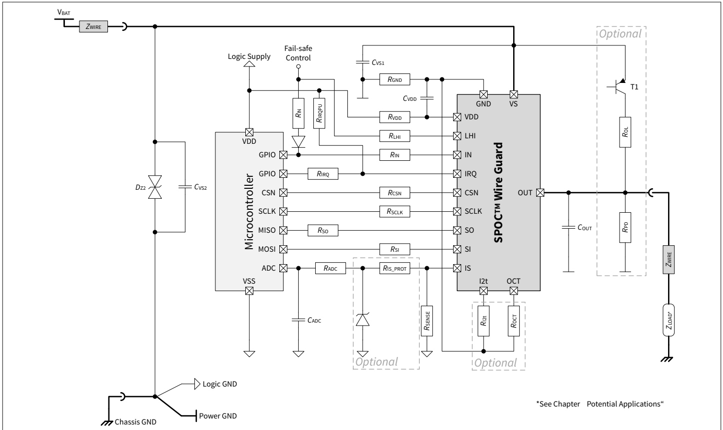
Figure 4 Application diagram
