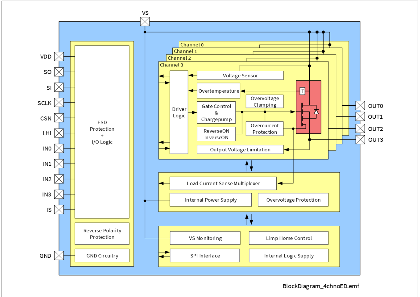
Figure 2 Block Diagram of BTS72220-4ESP
