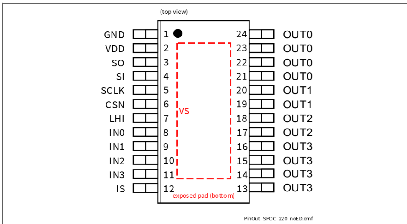
Figure 4 Pin Configuration
