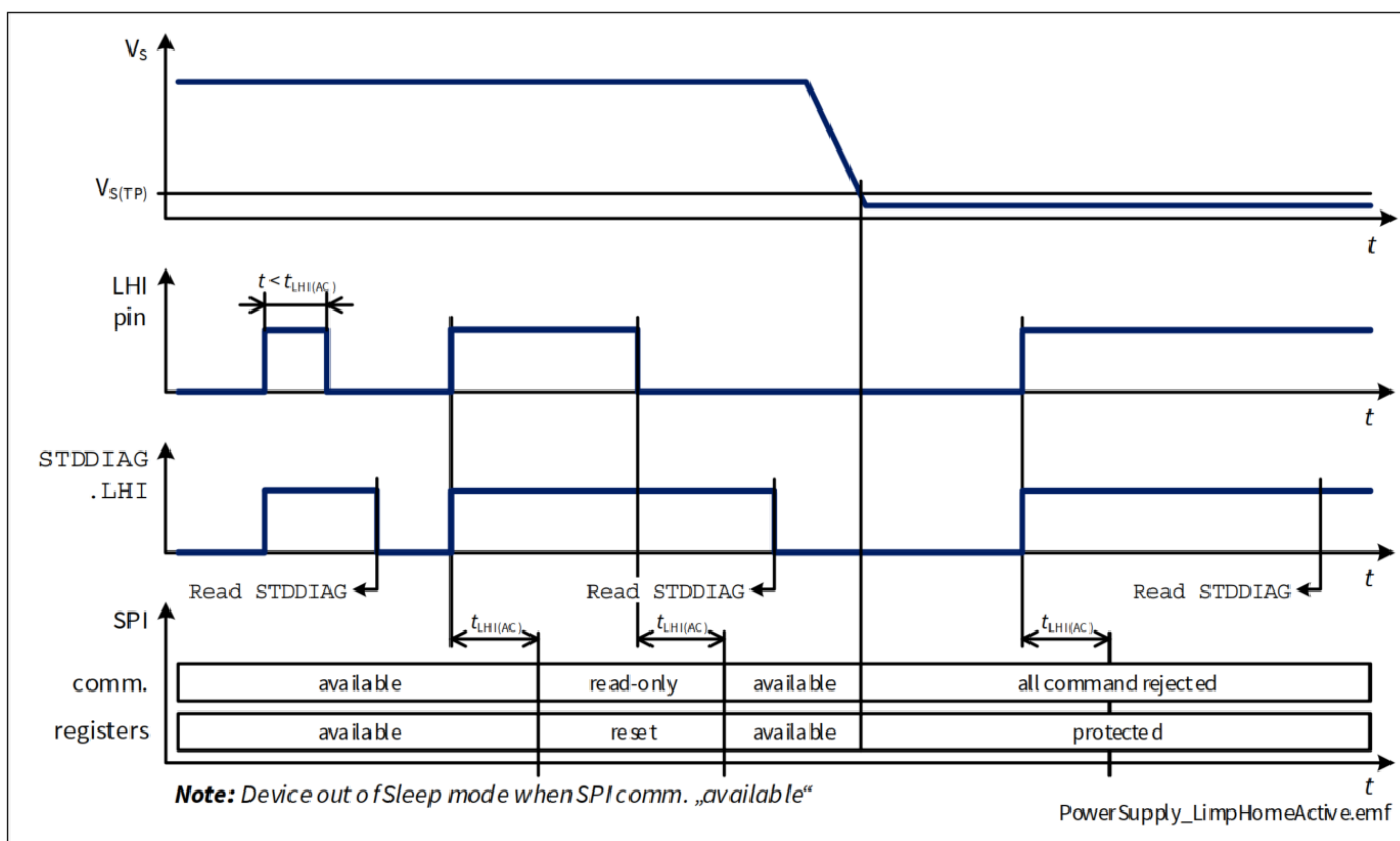
Figure 15 Limp Home Activation as function of V s
