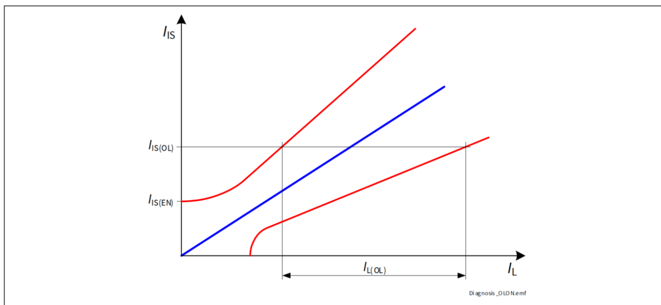
Figure 33 Current Sense Ratio in Open Load at ON condition
