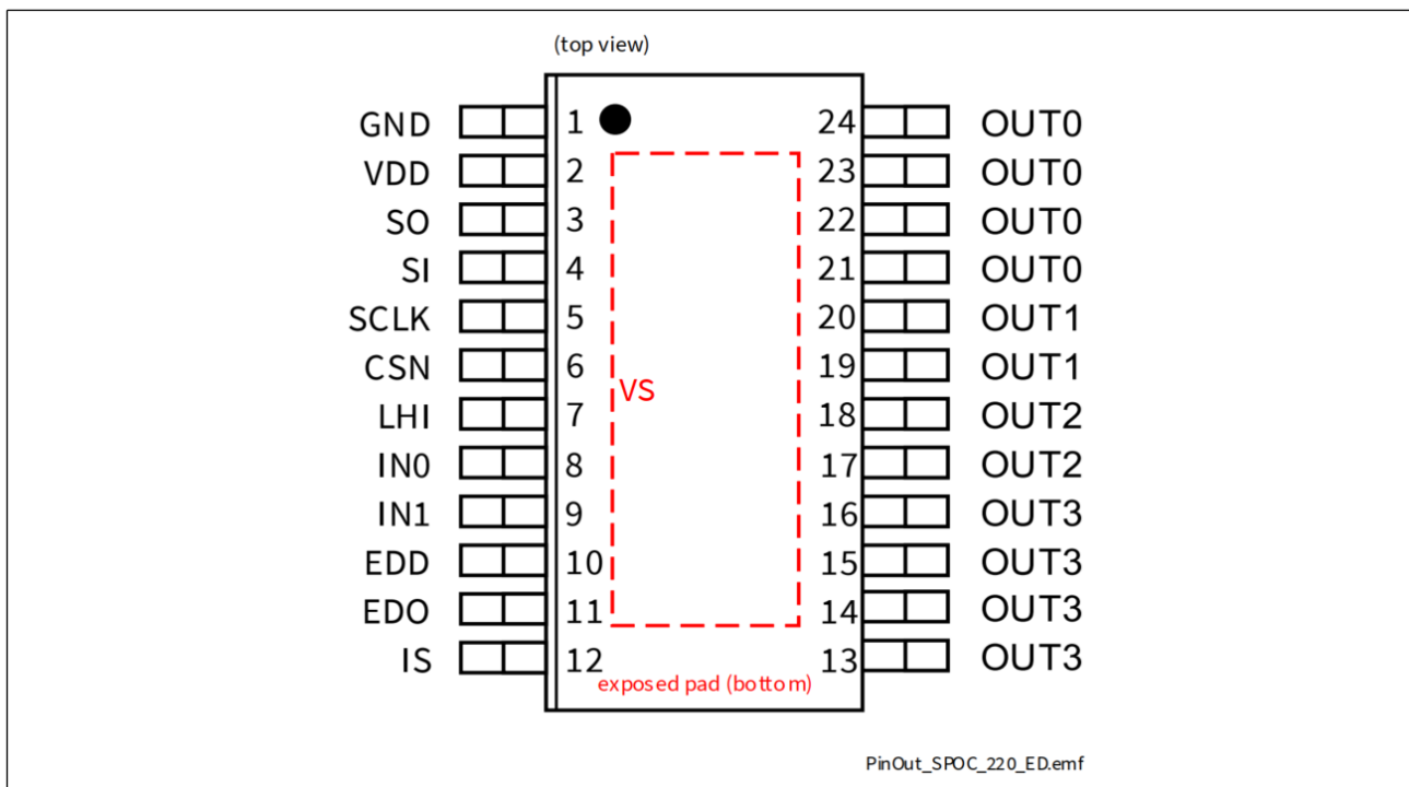
Figure 4 Pin Configuration
