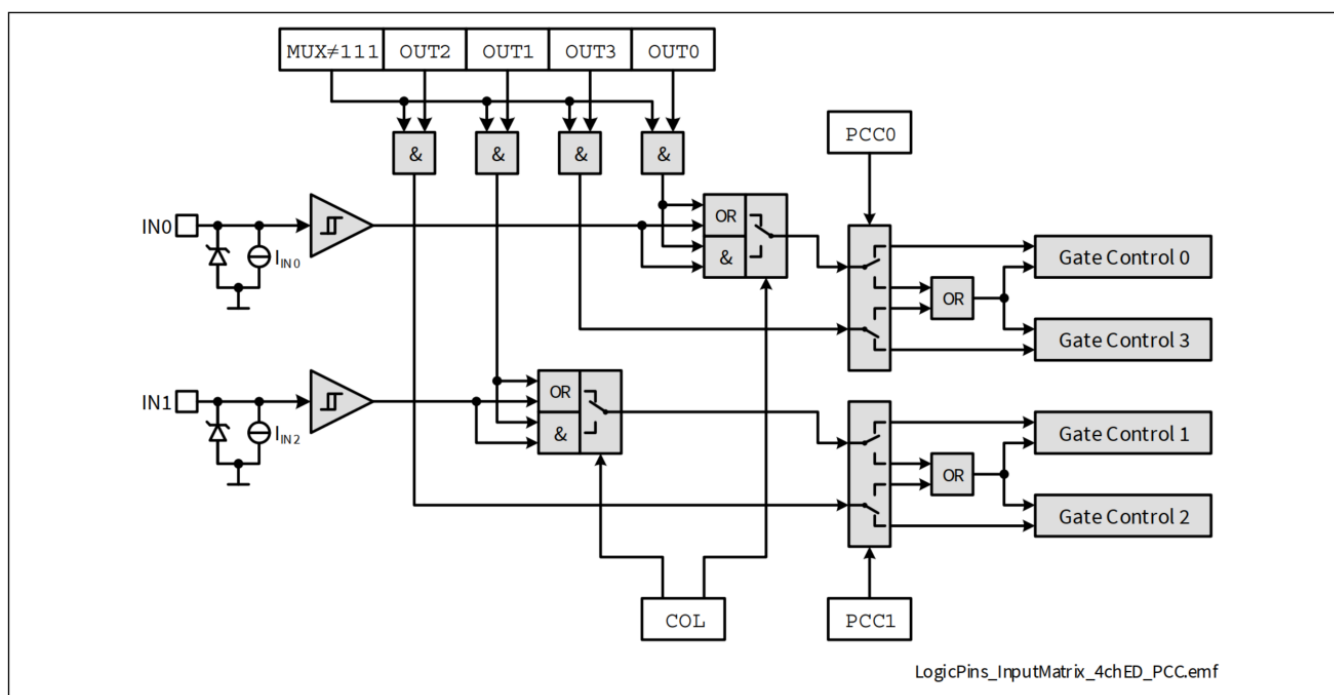
Figure 13 Input Switch Matrix
