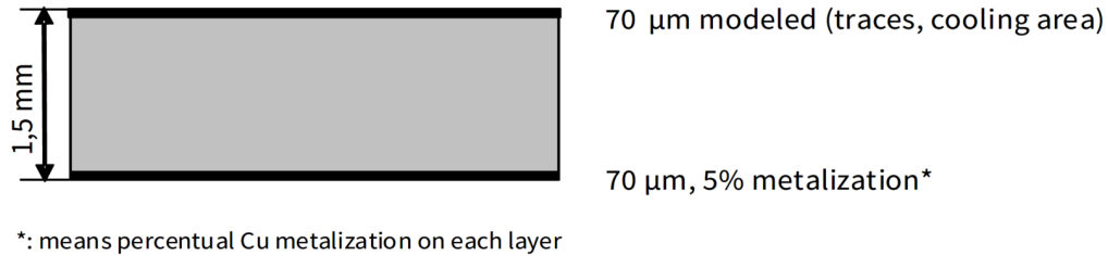
Figure 5 1s0p PCB Cross Section
