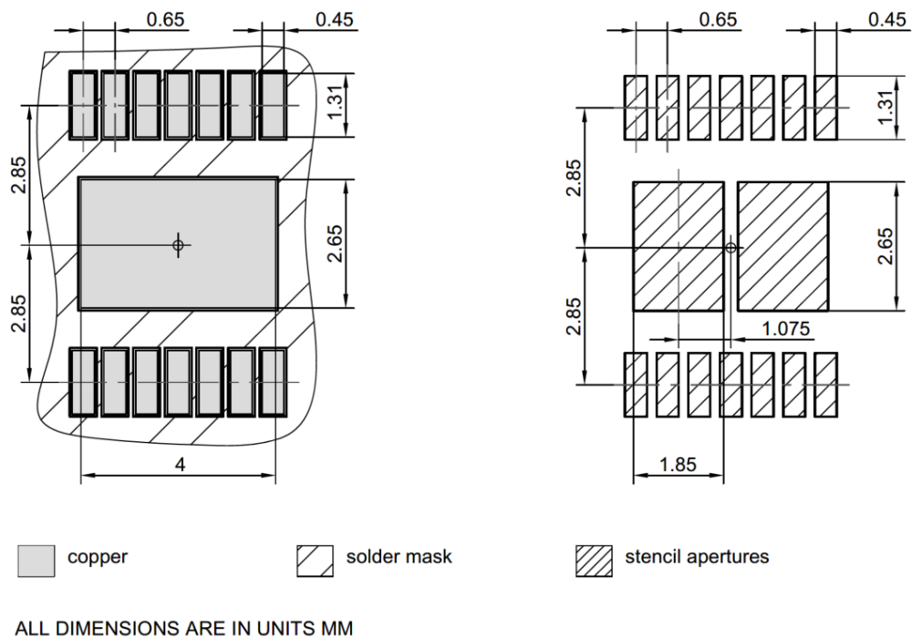
Figure 44 PG-TSDSO-14 (Thin (Slim) Dual Small Outline 14 pins) Package pads and stencil
