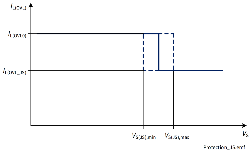
Figure 26 Overload Detection Current variation with V_S voltage
