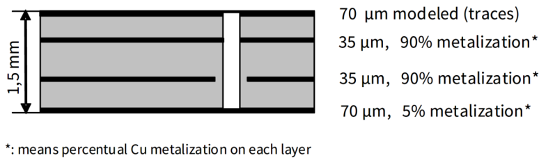
Figure 6 2s2p PCB Cross Section
