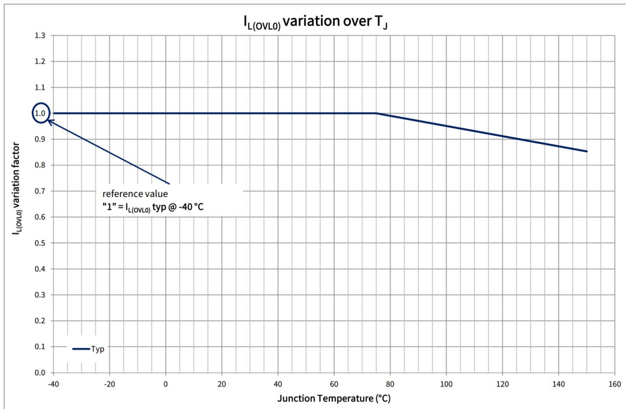
Figure 25 Overload Current Thresholds variation with T_J
