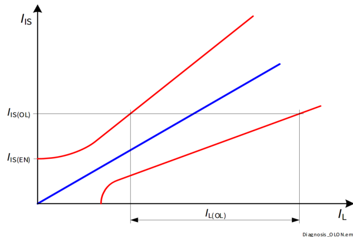
Figure 33 Current Sense Ratio in Open Load at ON condition
