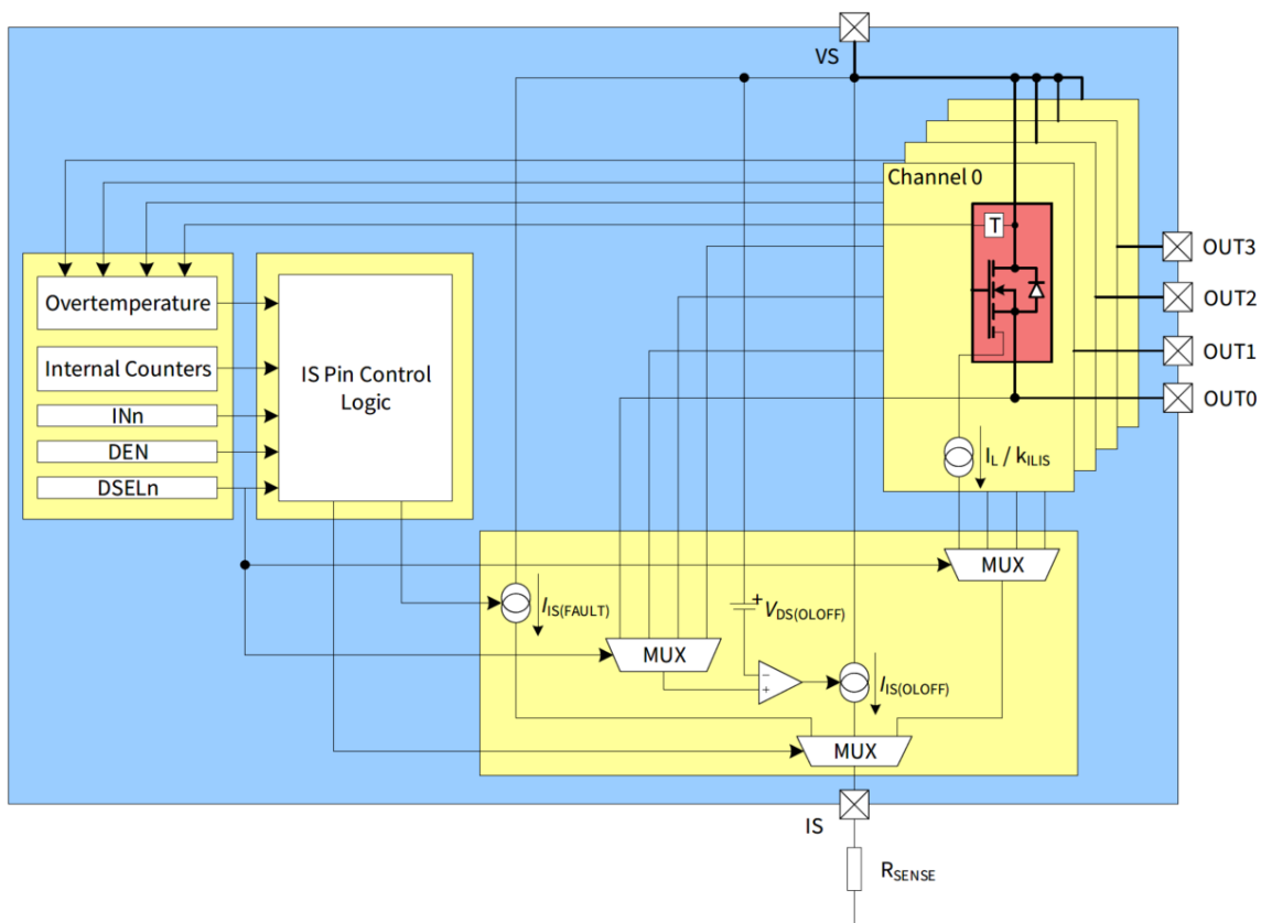
Figure 31 Diagnosis block diagram
