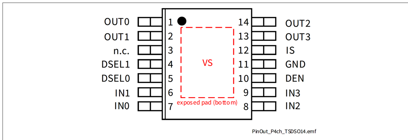
Figure 4 Pin Configuration
