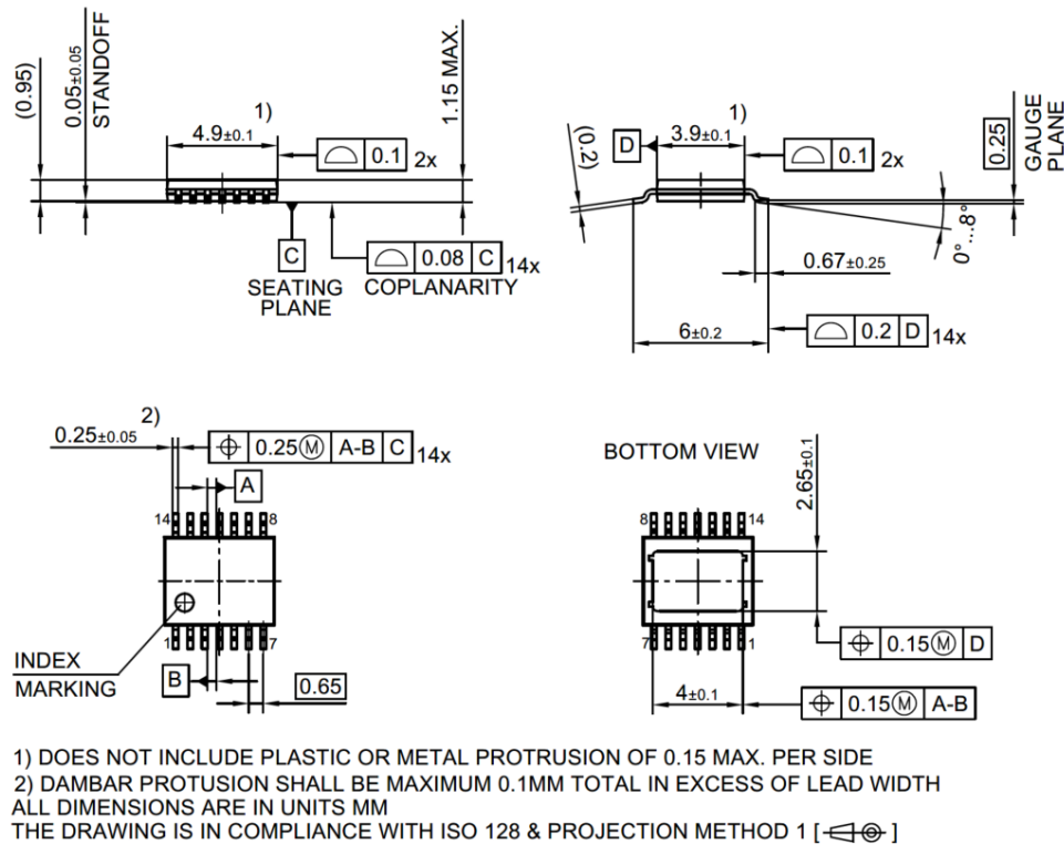
Figure 43 PG-TSDSO-14 (Thin (Slim) Dual Small Outline 14 pins) Package Outline
