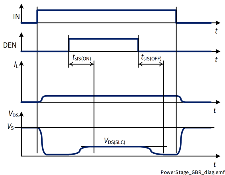
Figure 18 Output Voltage Limitation activation during diagnosis
