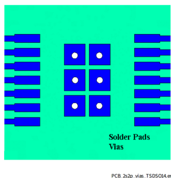
Figure 8 Thermal vias on PCB for 2s2p PCB setup
