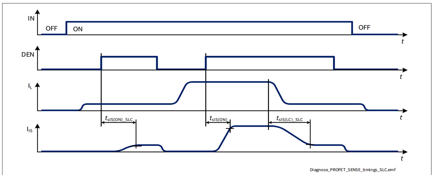
Figure 40 SENSE Timing with Small Load Current
