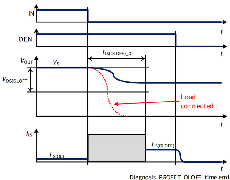
Figure 38 Open Load in OFF Timings - load disconnected
