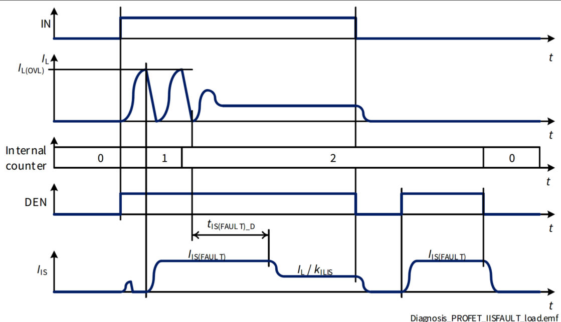
Figure 34 I_{IS(FAULT)} at Load Switching
