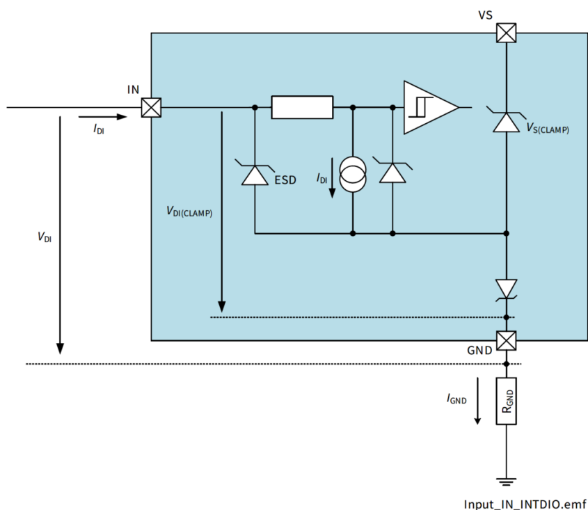
Figure 11 Input circuitry
