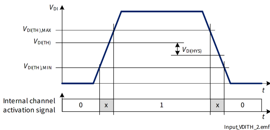
Figure 12 Input Threshold voltages and hysteresis
