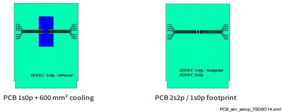
Figure 7 PCB setup for thermal simulations
