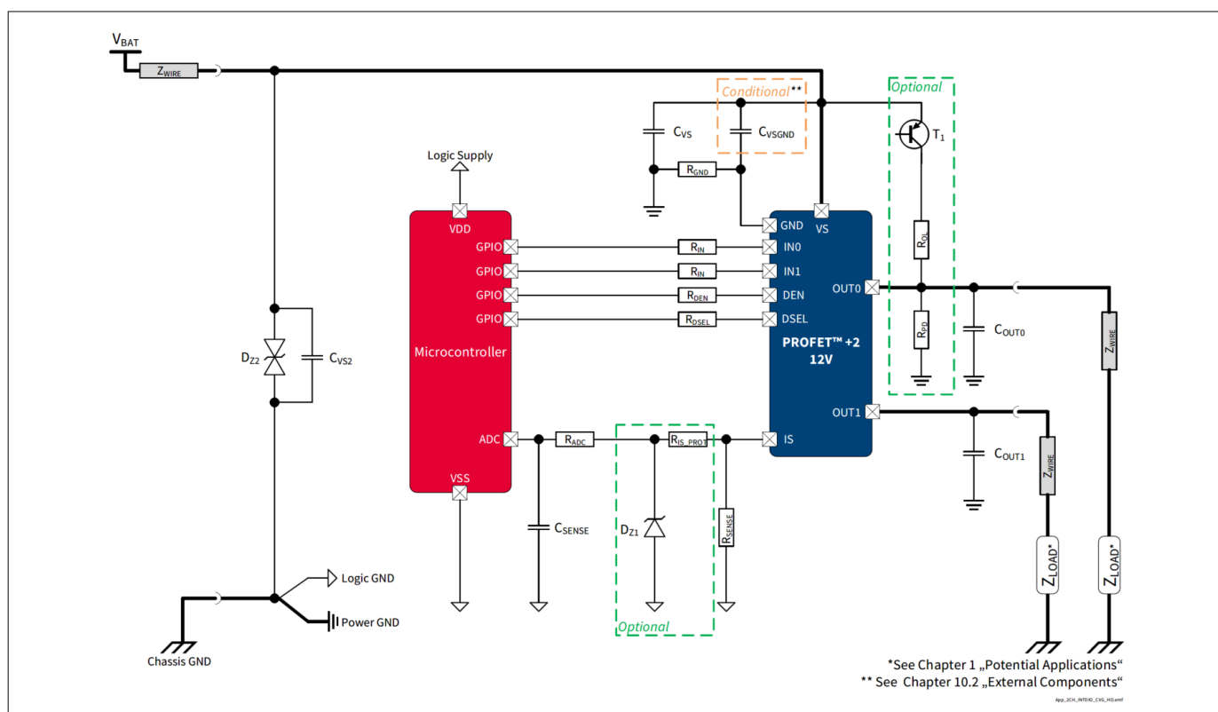
Figure 1 BTS7120-2EPG Application Diagram. Further information in Chapter 10
