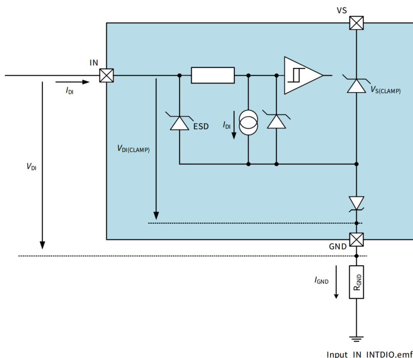
Figure 11 Input circuitry
