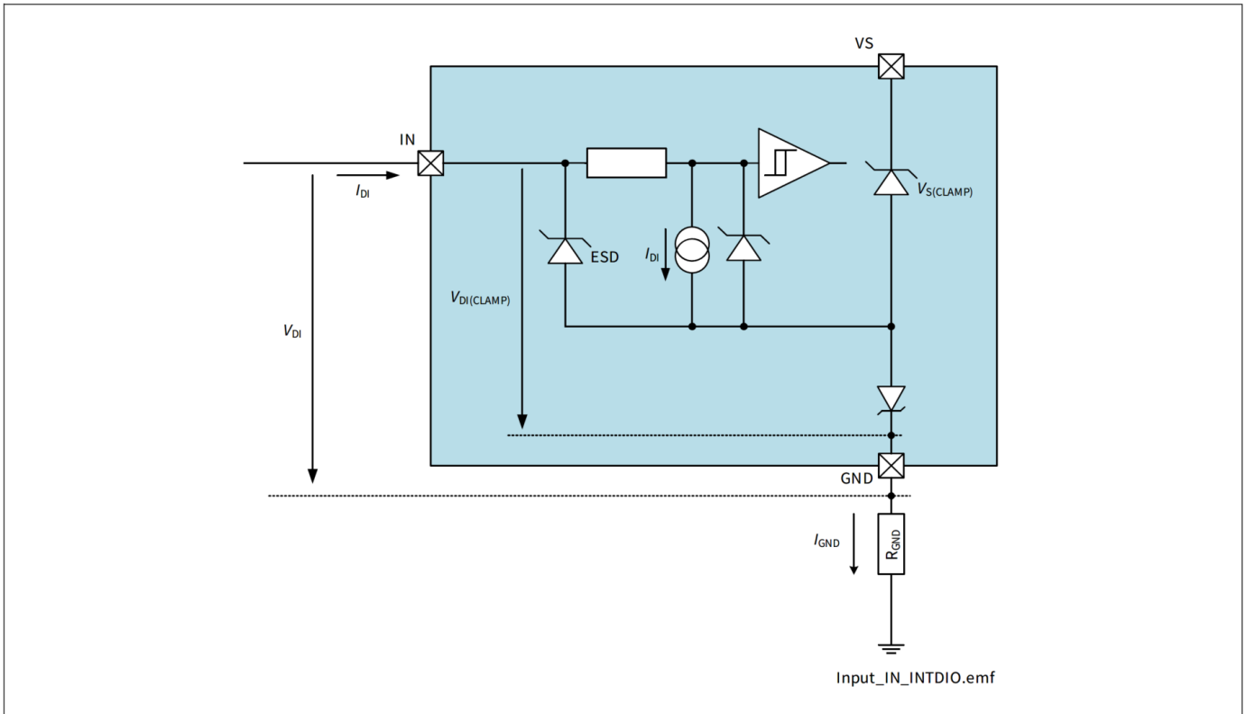
Figure 11 Input circuitry
