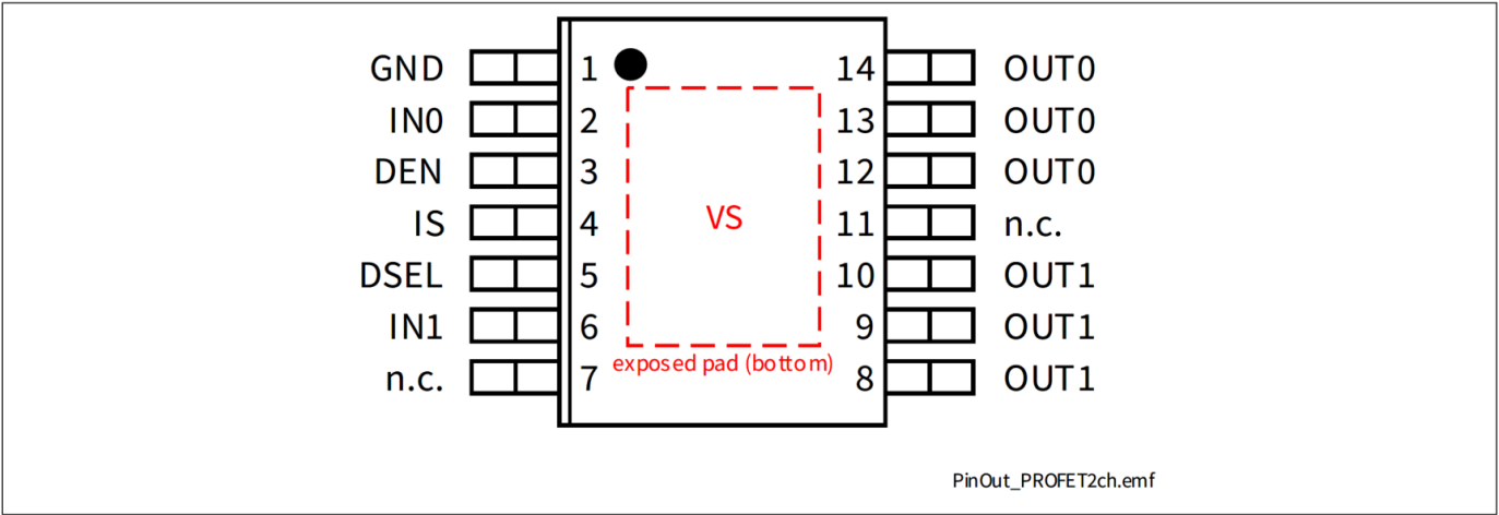
Figure 4 Pin Configuration
