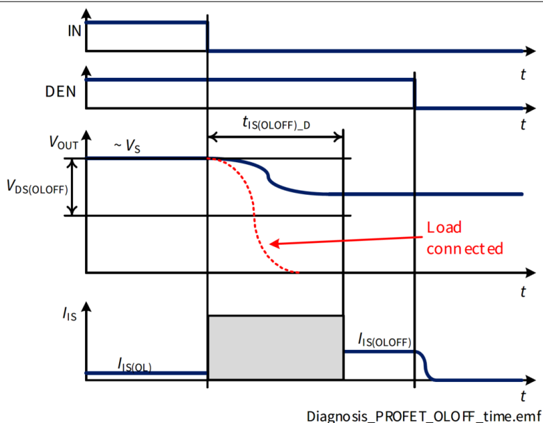
Figure 39 Open Load in OFF Timings - load disconnected
