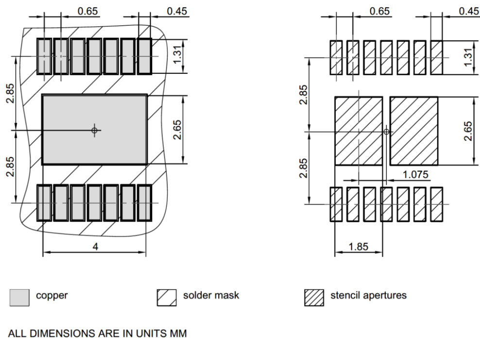
Figure 45 PG-TSDSO-14 (Thin (Slim) Dual Small Outline 14 pins) Package pads and stencil
