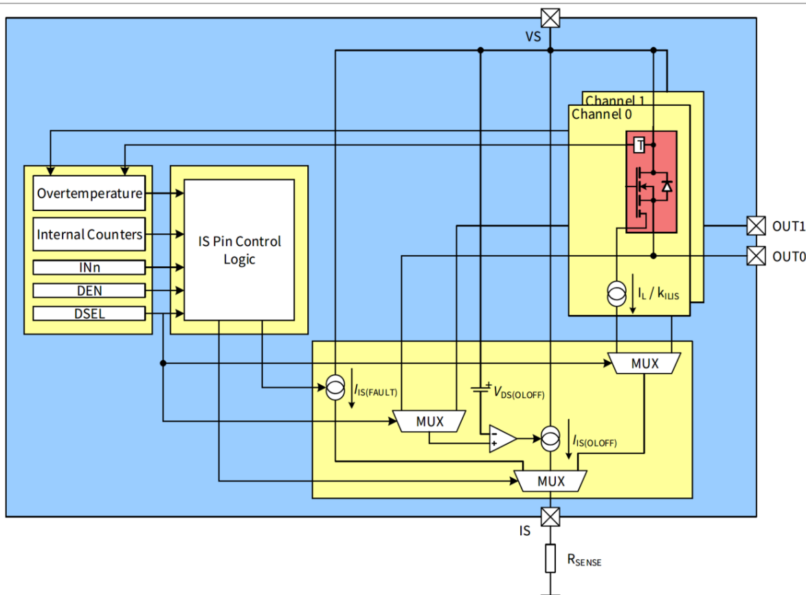
Figure 32 Diagnosis Block Diagram
