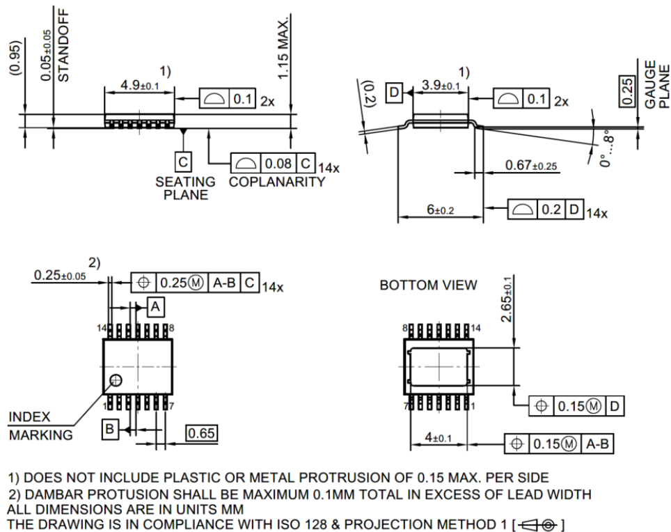
Figure 44 PG-TSDSO-14 (Thin (Slim) Dual Small Outline 14 pins) Package Outline
