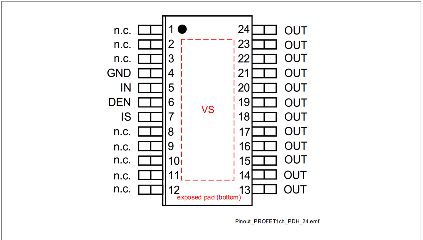
Figure 4 Pin Configuration
