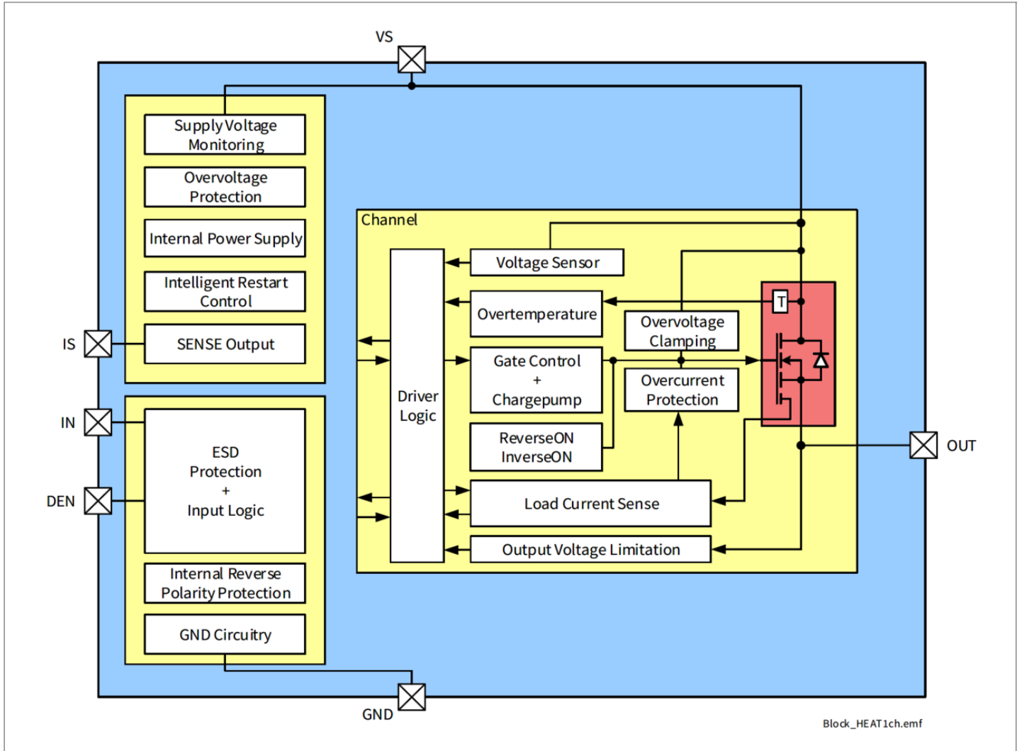
Figure 2 Block Diagram of BTS70012-1ESP
