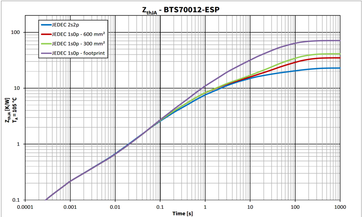
Figure 9 Typical Thermal Impedance. PCB setup according to Chapter 4.4.1
