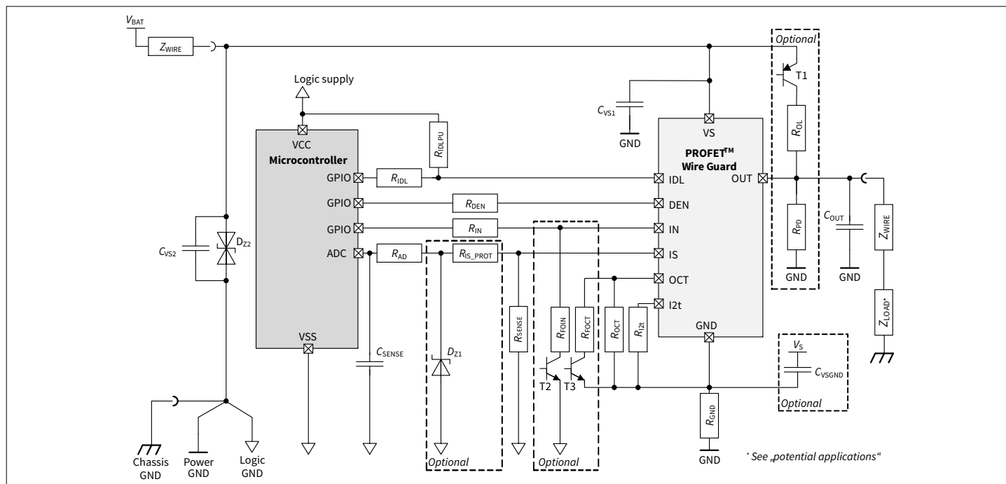
Figure 54 PROFET™ Wire Guard - application diagram
