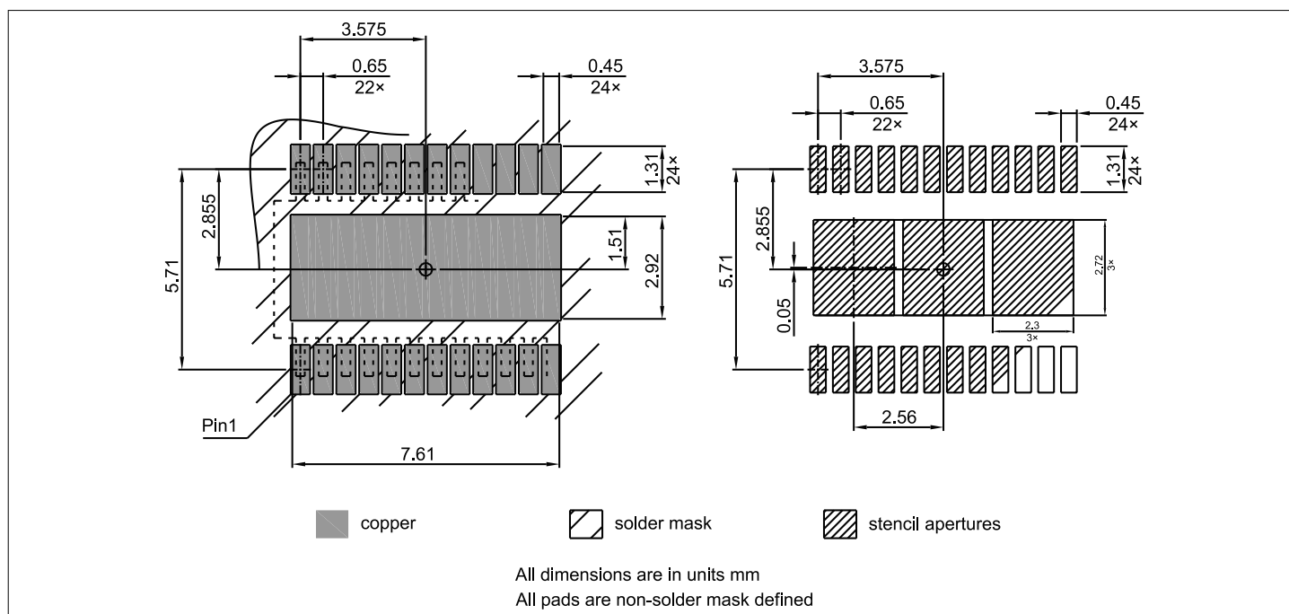
Figure 56 PG-TSDSO-24 (thin (slim) dual small outline 24 pins) package pads and stencil
