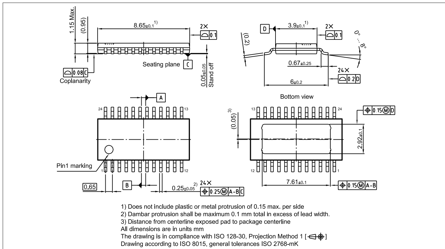
Figure 55 PG-TSDSO-24 (thin (slim) dual small outline 24 pins) package outline
