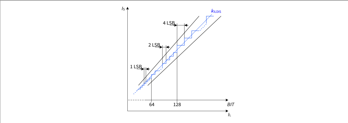
Figure 52 Digital current sense behavior - overview
