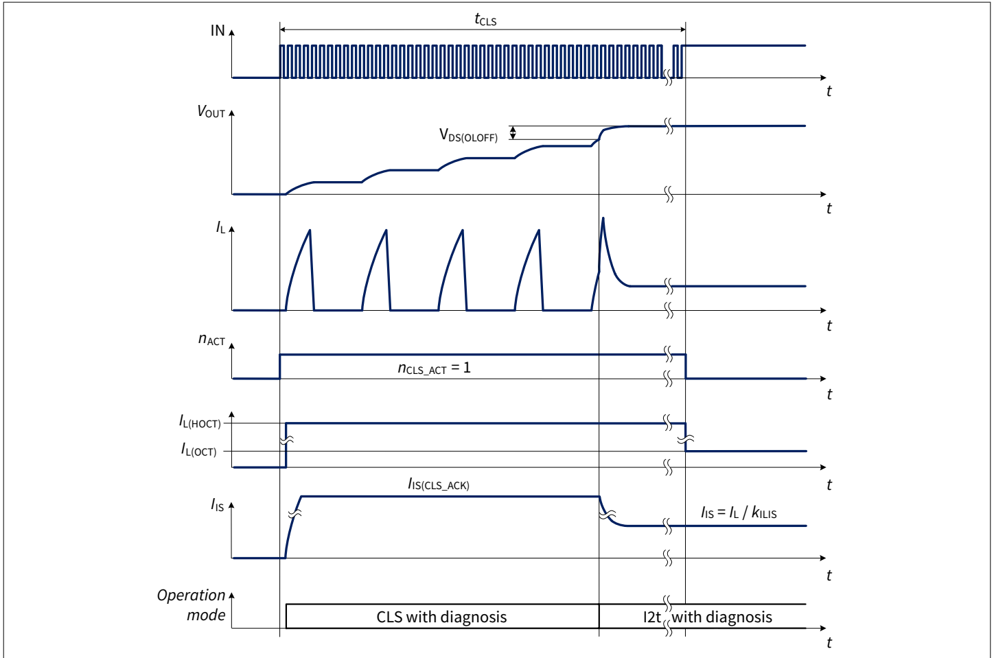
Figure 22 Capacitive load switching activations
