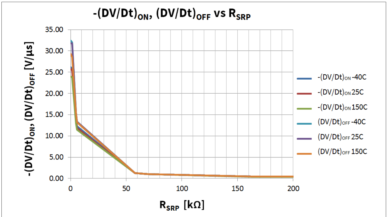
图 33 -(\Delta V/\Delta t)_{ON}, (\Delta V/\Delta t)_{OFF} vs. R_{SRP} ; V_{IN} = V_{ENABLE} = V_{DD} = 5V ; V_{BAT} = 13.5V ; R_L = 10\Omega ; T_J = -40, 25, 150^\circ C
