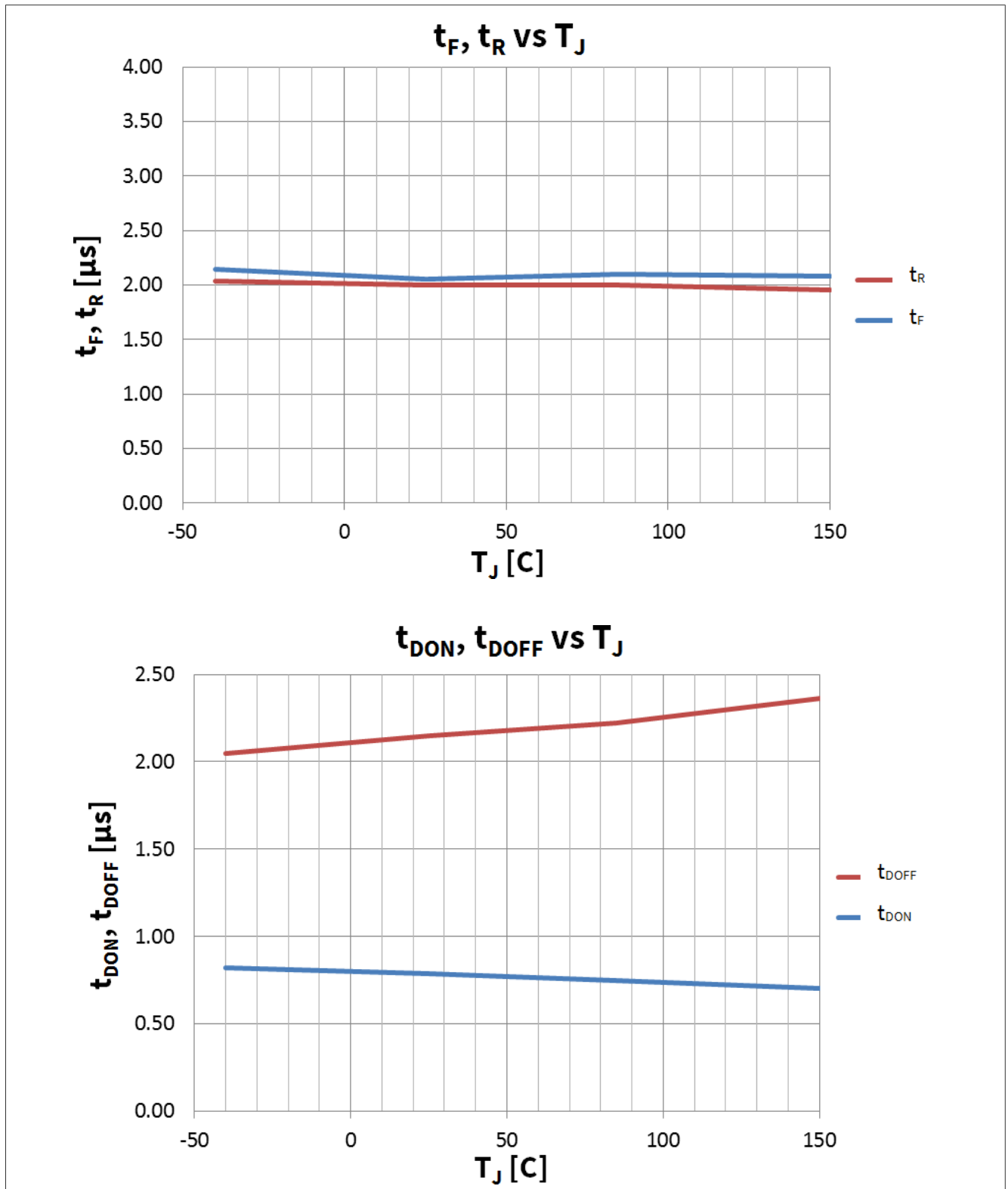
图 37 t_F, t_R, t_{DON}, t_{DOFF} vs. T_J = -40; 25; 150^\circ\text{C} @ R_{SRP} = 5.8\text{k}\Omega; V_{IN} = V_{ENABLE} = V_{DD} = 5\text{V}; V_{BAT} = 13.5\text{V}; R_L = 10\Omega
