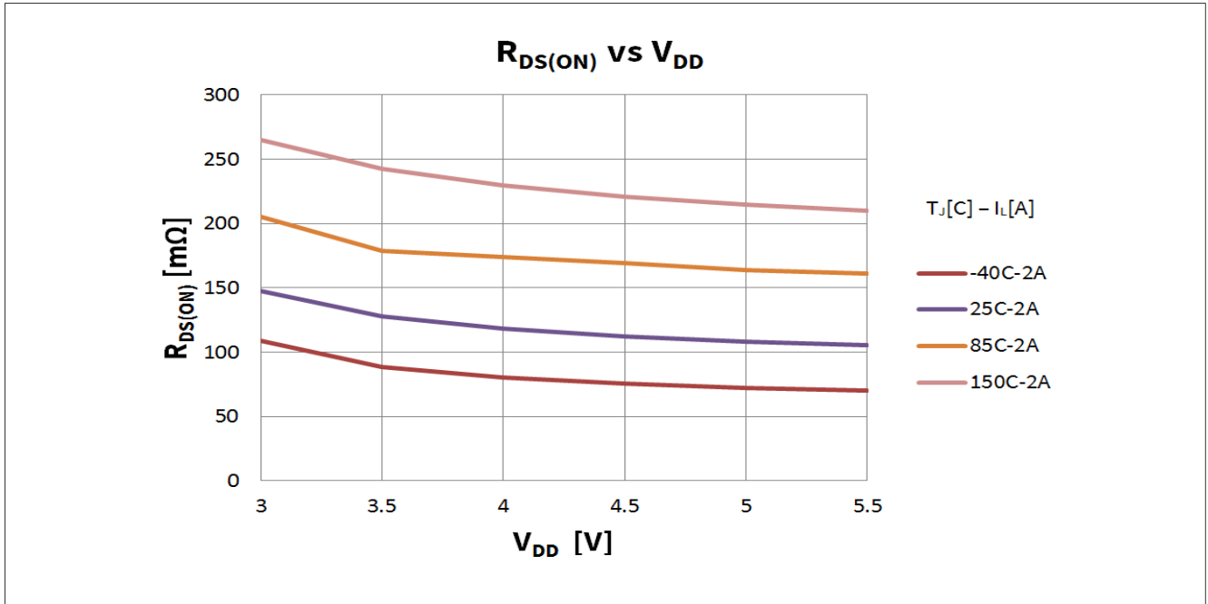
图 24 R_{DS(ON)} vs. V_{DD} @ T_J = -40, 25, 150^\circ\text{C} , I_L = I_{L(NOM)} ; V_{IN} = V_{ENABLE} = 5\text{V} ; V_{DD} = 3 \dots 5.5\text{V} ; R_{SRP} = 0\Omega
