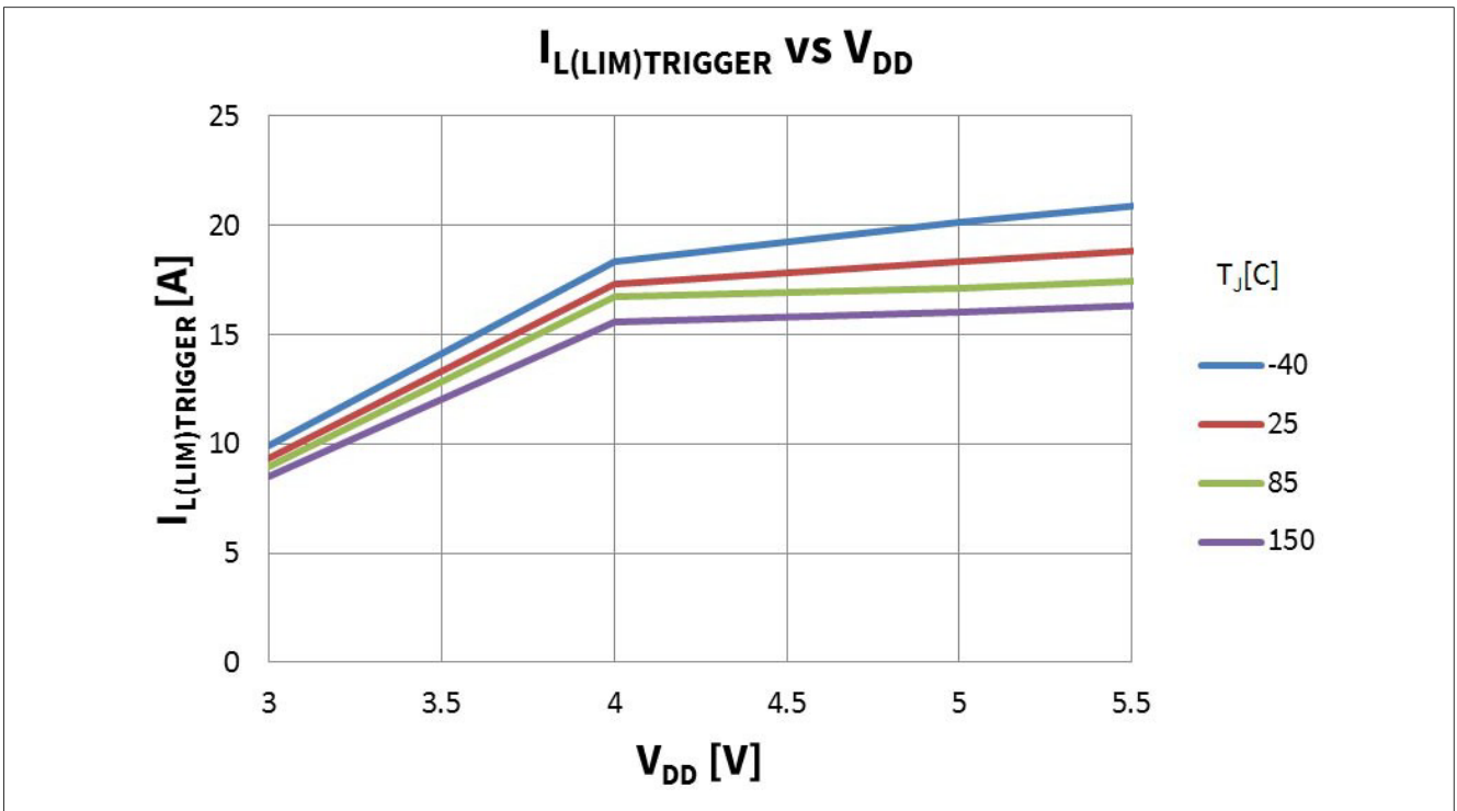
图 41 I_{L(LIM)TRIGGER} peak vs. V_{DD}=3. \dots 5.5V @ T_J=-40, 25, 85, 150^\circ C; V_{IN}= PWM 5V in SOA; V_{ENABLE}= 5V; V_{BAT}= 13.5V; R_L= 10\Omega
