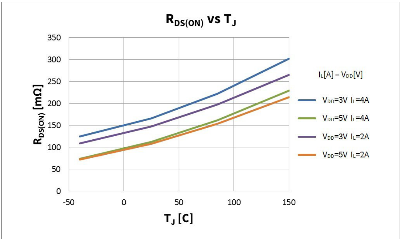
图26 R_{DS(ON)} 与 T_J @ V_{DD}=5V ; V_{IN} = V_{ENABLE} = 5V ; T_J = -40, 25, 85, 150^\circ C ;
