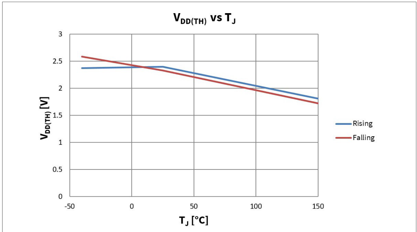
图45 V DD(TH) vs. T J = -40, 25, 150°C; V IN =V ENABLE = 5V; R L = 10Ω; V BAT = 13.5V; R SRP = 0Ω
