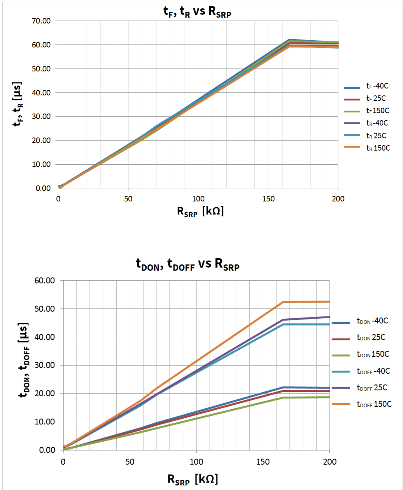
图 32 t_F, t_R, t_{DON}, t_{DOFF} vs. R_{SRP} ; V_{IN} = V_{ENABLE} = V_{DD} = 5V ; V_{BAT} = 13.5V ; R_L = 10\Omega ; T_J = -40, 25, 150^\circ C
