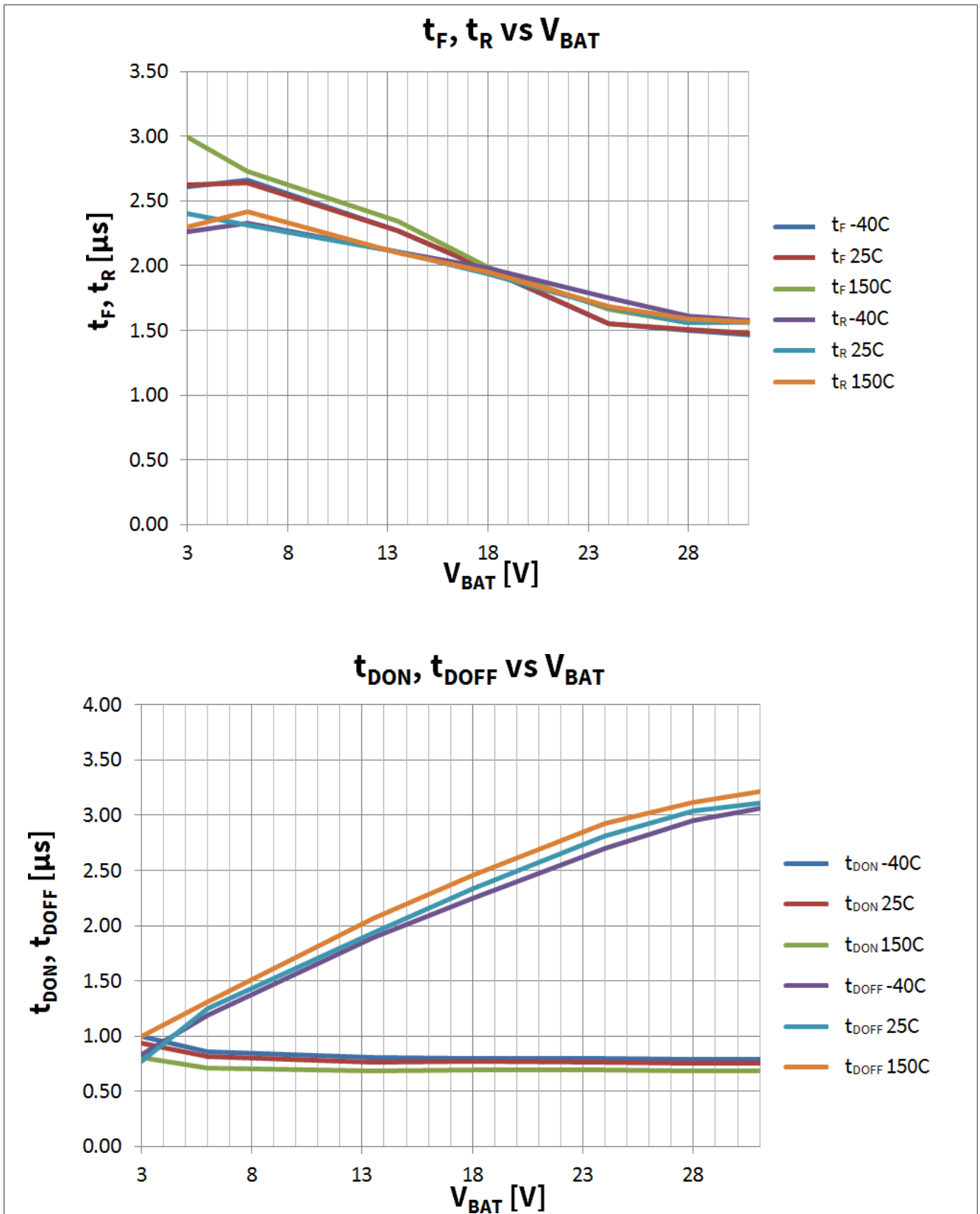
图 35 t_F, t_R, t_{DON}, t_{DOFF} vs. V_{BAT}=3..31V @ V_{DD}=5V; V_{IN} = V_{ENABLE} = V_{DD} = 5V; R_L = 10\Omega; R_{SRP}=5.8k\Omega , 开路; T_J = -40, 25, 150^\circ C
