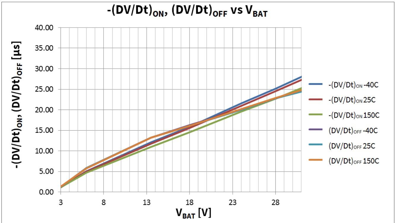
图 36 转化率 -(\Delta V/\Delta t)_{ON}, (\Delta V/\Delta t)_{OFF} vs. V_{BAT} @ T_J = -40, 25, 150^\circ\text{C} ; R_L = 10\Omega ; R_{SRP} = 5.8\text{k}\Omega ; V_{IN} = V_{DD} = V_{ENABLE} = 5\text{V} ; V_{BAT} = 3..31\text{V}
