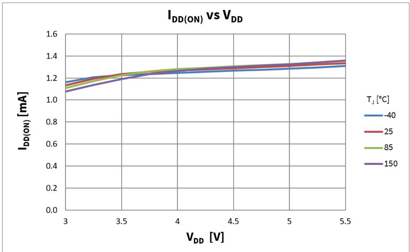
图 46 I DD(ON) vs. V DD = 3V...5.5V@ T J = -40, 25, 85, 150°C; V IN = V ENABLE = 5V; R SRP = 0Ω; V BAT = 13.5V;
