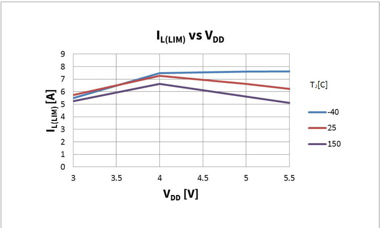
图 42 I_{L(LIM)} vs. V_{DD}= 3V. \dots V @ T_J= -40, 25, 150^\circ C; V_{ENABLE}=V_{IN}= 5V; V_{BAT}= 13.5V
