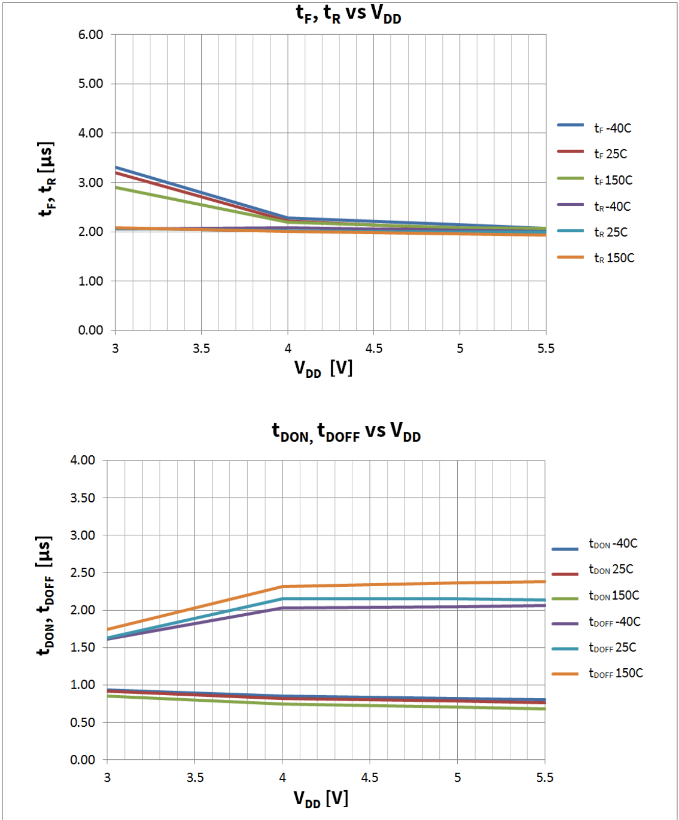
图 34 t_F, t_R, t_{DON}, t_{DOFF} vs. V_{DD}=3..5.5V @ V_{BAT}=13.5V; T_J = -40, 25, 150^\circ C; R_{SRP} = 5.8k\Omega; V_{IN} = V_{ENABLE} = 5V; R_L=10\Omega;
