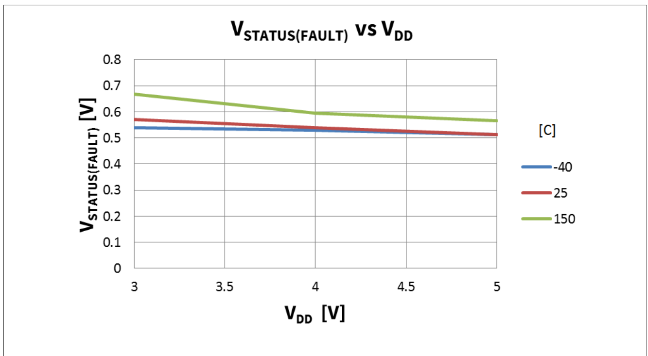
图 44 V_{STATUS} in fault mode vs. V_{DD} = 3V..5V @ T_J = -40, 25, 150^{\circ}C ; V_{IN} = V_{ENABLE} = 5V ; V_{BAT} = 13.5V ;
