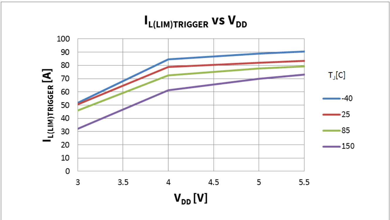
图 41 I_{L(LIM)TRIGGER} peak vs. V_{DD}=3. \dots 5.5V @ T_J = -40, 25, 85, 150^\circ C ; V_{IN} = PWM 5V in SOA; V_{ENABLE} = 5V ; V_{BAT} = 13.5V ; R_L = 4.7\Omega
