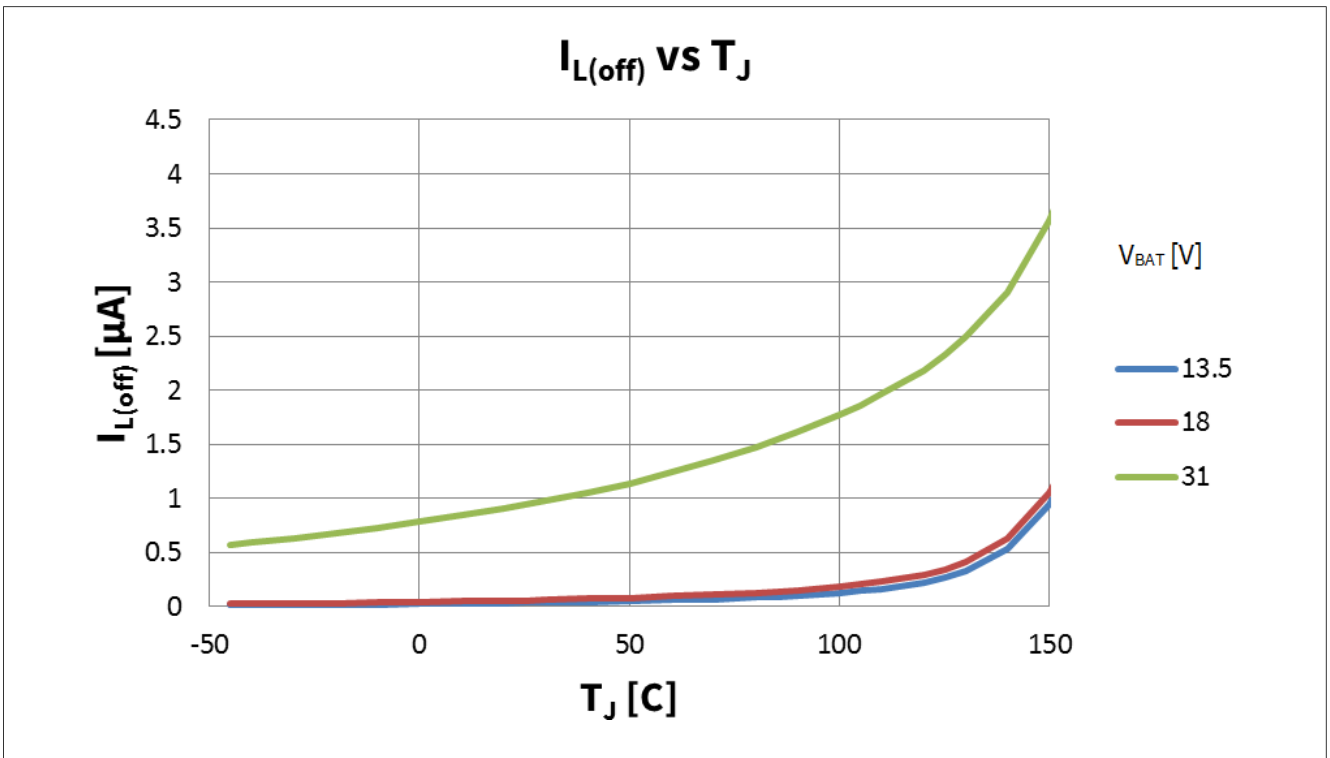
图 27 I_{L(OFF)} 与 T_J @ V_{IN} = 0V ; V_{ENABLE} = V_{DD} = 5V ; T_J = -40, -20, 0, 25, 50, 85, 105, 125, 150^{\circ}C ; V_{BAT} = 13.5V, 18V, 31V
