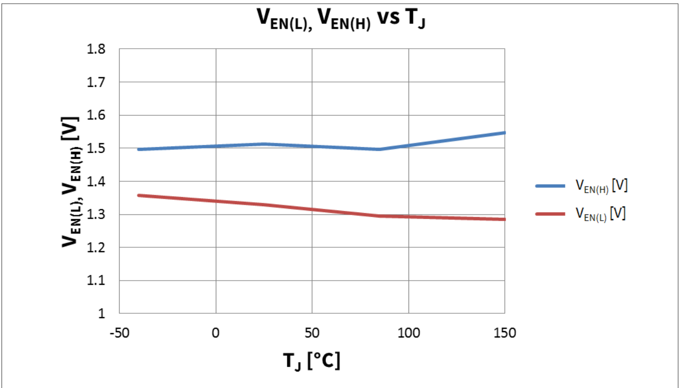
图 50 V_{EN(L)}, V_{EN(H)} vs. T_J @ V_{DD} = 5V ; V_{BAT} = 13.5V ; I_L = 1.4mA ; R_{SRP} = 0\Omega ; V_{EN} = 0V..5.5V ; V_{BAT} = 13.5V ;
