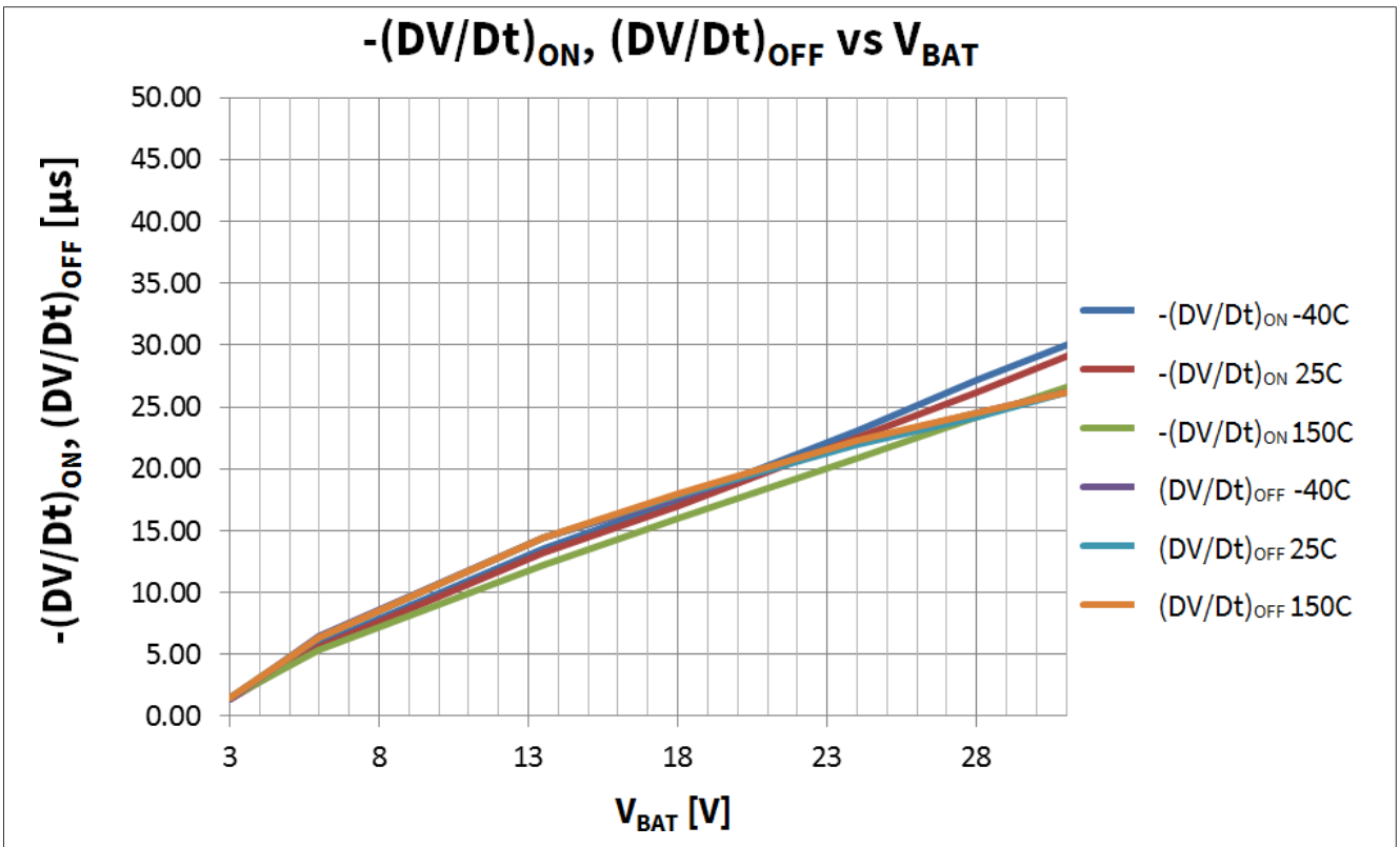
图 36 转换率 -(\Delta V/\Delta t)_{ON} , (\Delta V/\Delta t)_{OFF} vs. V_{BAT} @ T_J = -40, 25, 150^\circ C ; R_L = 4.7\Omega ; R_{SRP} = 5.8k\Omega ; V_{IN} = V_{DD} = V_{ENABLE} = 5V ; V_{BAT} = 3..31V
