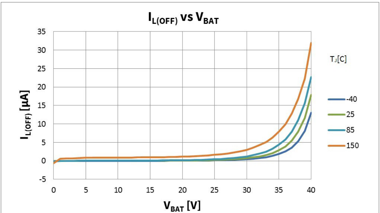
图 28 I_{L(OFF)} 与 V_{BAT} = 0..40V @ T_J = -40, 25, 85, 150^{\circ}C ; V_{IN} = 0V ; V_{ENABLE} = V_{DD} = 5V
