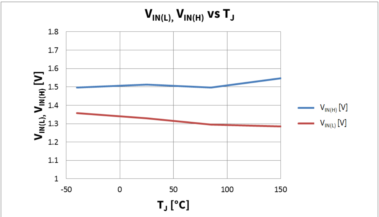
图 49 V_{IN(L)}, V_{IN(H)} vs. T_J @ V_{DD} = 5V ; V_{ENABLE} = 5V ; I_L = 1.4 mA ; R_{SRP} = 0\Omega ; V_{IN} = 0V..5.5V ; V_{BAT} = 13.5V ;
