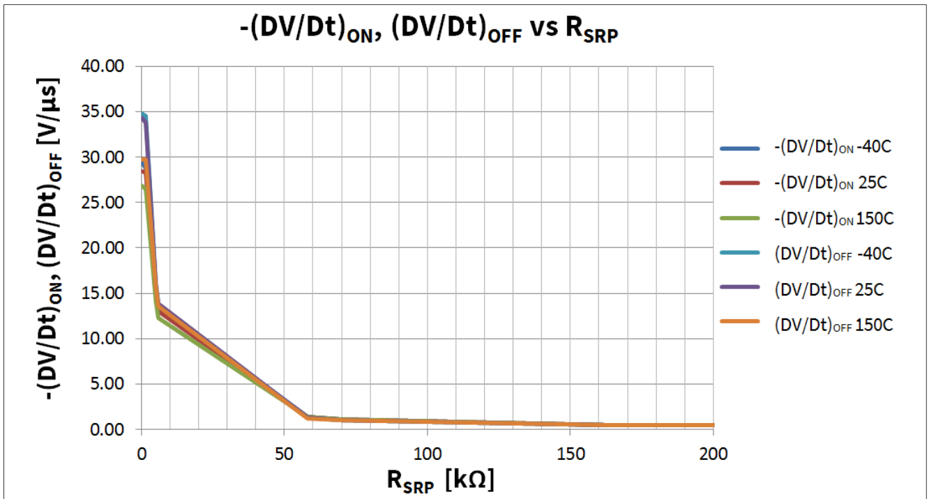
图 33 -(\Delta V/\Delta t)_{ON}, (\Delta V/\Delta t)_{OFF} vs. R_{SRP} ; V_{IN} = V_{ENABLE} = V_{DD} = 5V ; V_{BAT} = 13.5V ; R_L = 4.7\Omega ; T_J = -40, 25, 150^\circ C
