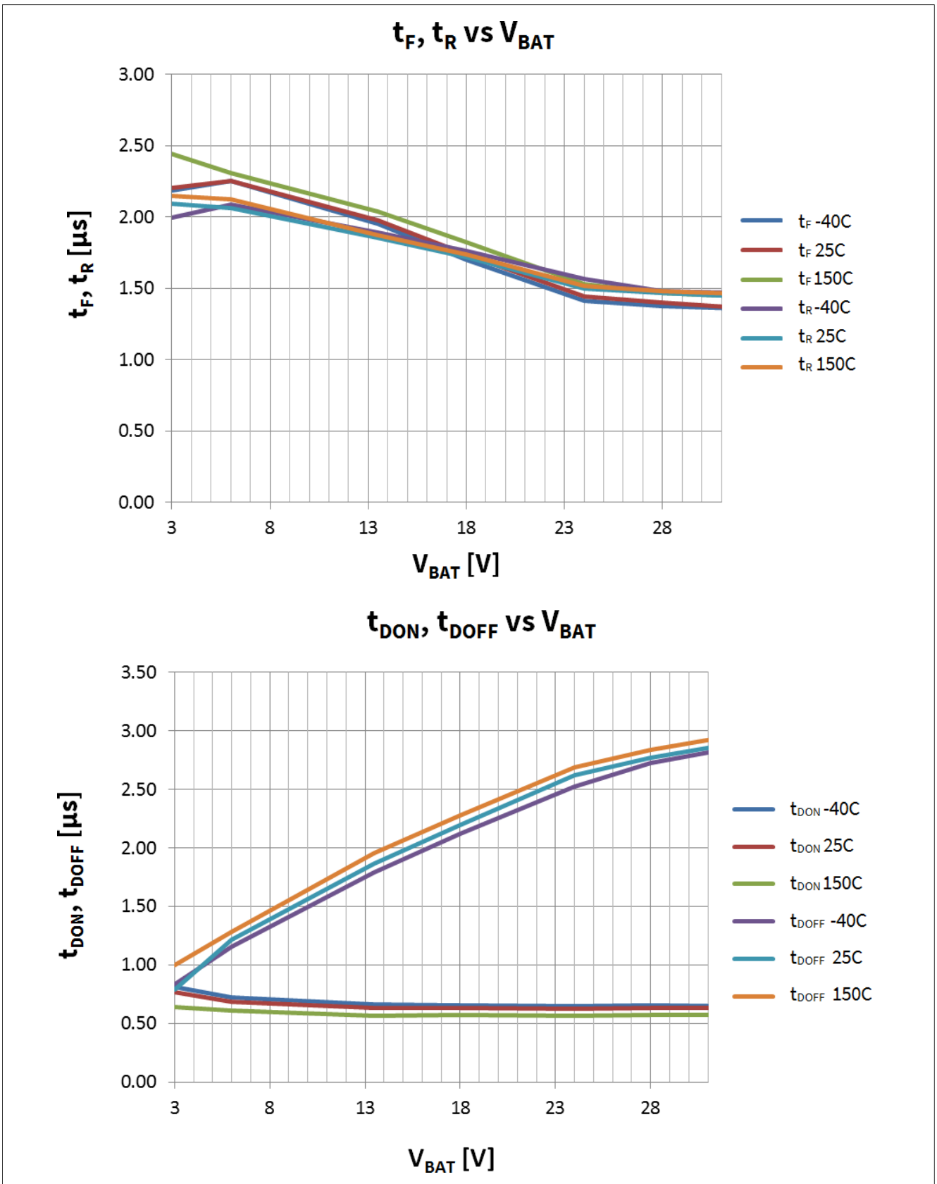
图 35 t_F, t_R, t_{DON}, t_{DOFF} vs. V_{BAT}=3..31V @ V_{DD}=5V; V_{IN} = V_{ENABLE} = V_{DD} = 5V; R_L = 4.7\Omega; R_{SRP}=5.8k\Omega , 开路; T_J = -40, 25, 150^\circ C
