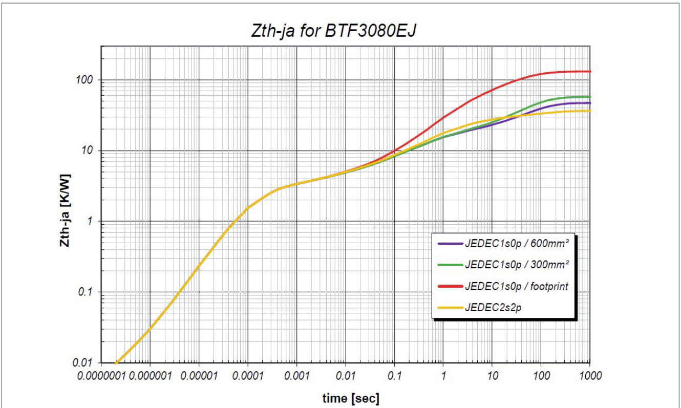
图 7 典型瞬态热阻抗 Z_{thJA} = f(t_p) , T_a = 85^\circ\text{C}
