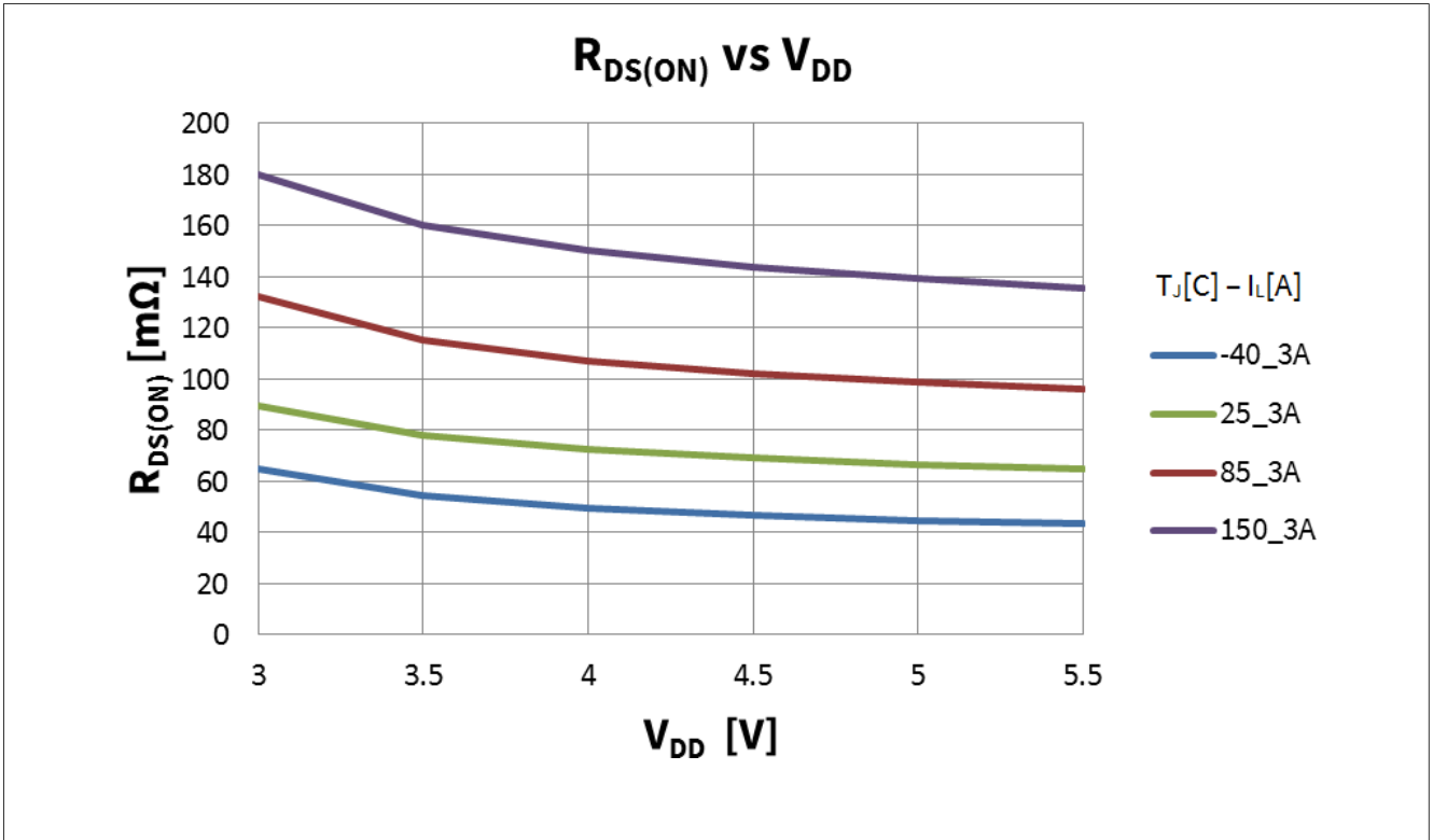
图 24 R_{DS(ON)} vs. V_{DD} @ T_J = -40, 25, 85, 150^\circ\text{C} , I_L = I_{L(NOM)} ; V_{IN} = V_{ENABLE} = 5\text{V} ; V_{DD} = 3.. 5.5\text{V} ; R_{SRP} = 0\Omega
