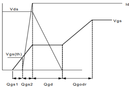
Fig 13a. Gate Charge Waveform
