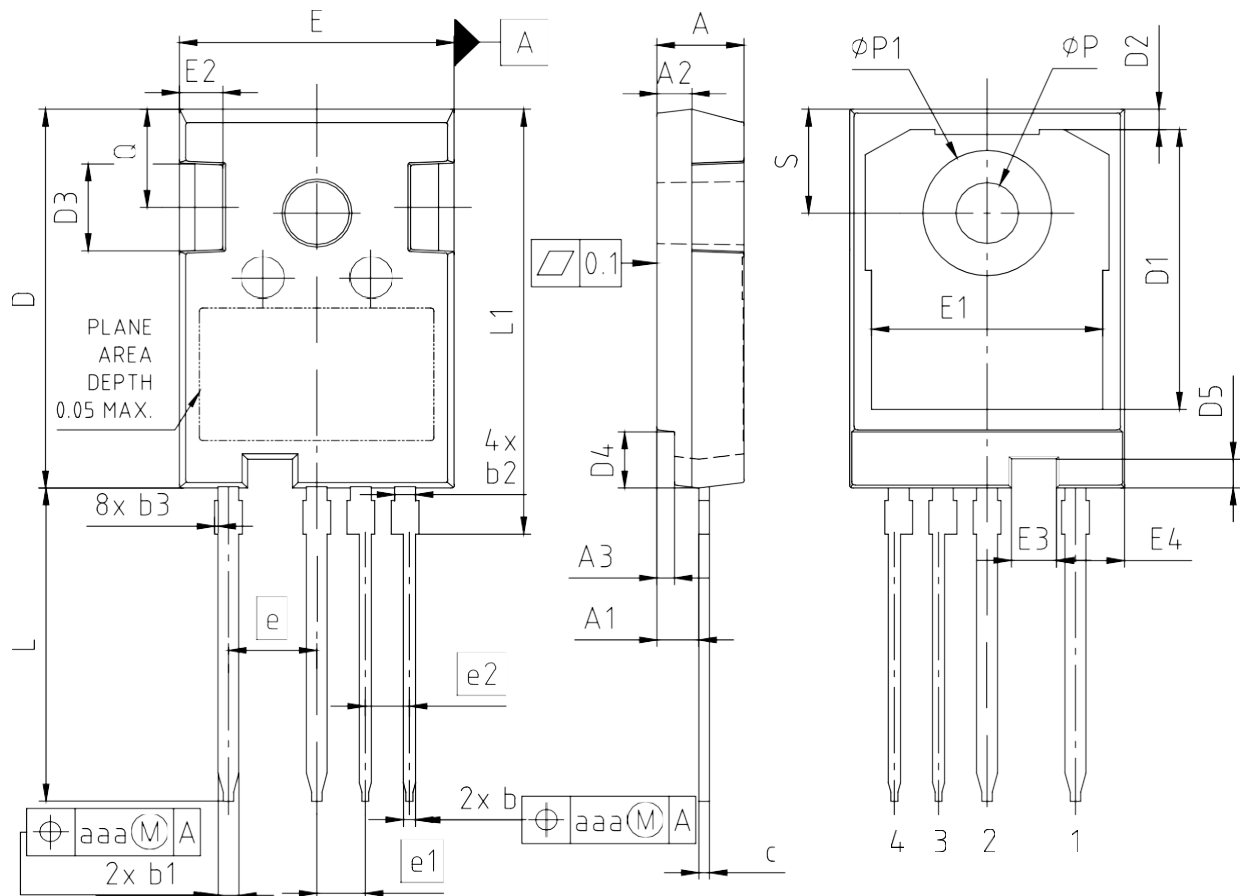
PACKAGE - GROUP NUMBER: PG-TO247-4-U03
