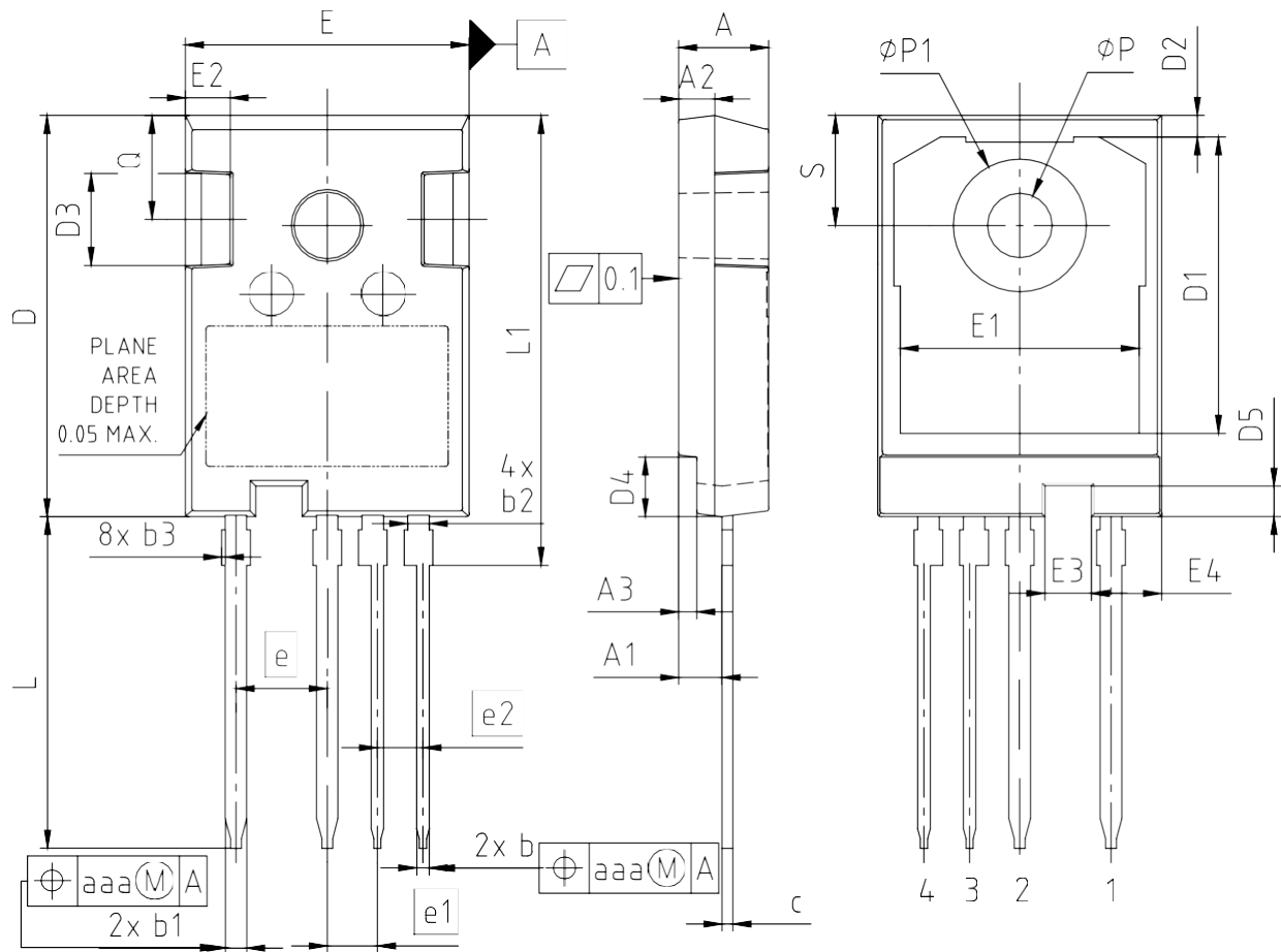
PACKAGE - GROUP NUMBER: PG-TO247-4-U03
