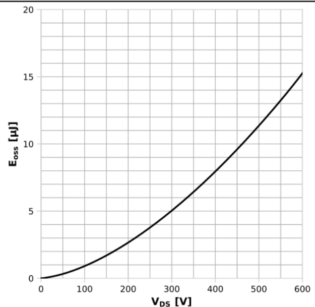
Diagram 16: Typ. Coss stored energy
