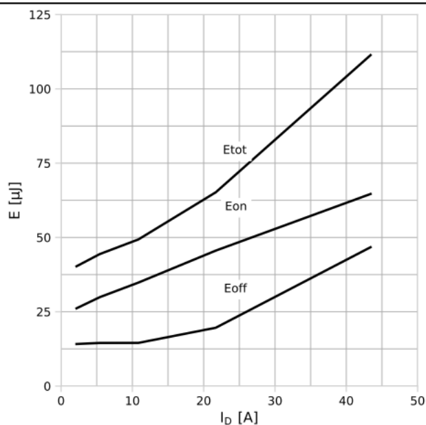
Diagram 20: Typ. Switching Losses vs switching current
