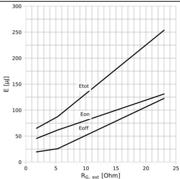
Diagram 19: Typ. Switching Losses vs RGeXt
