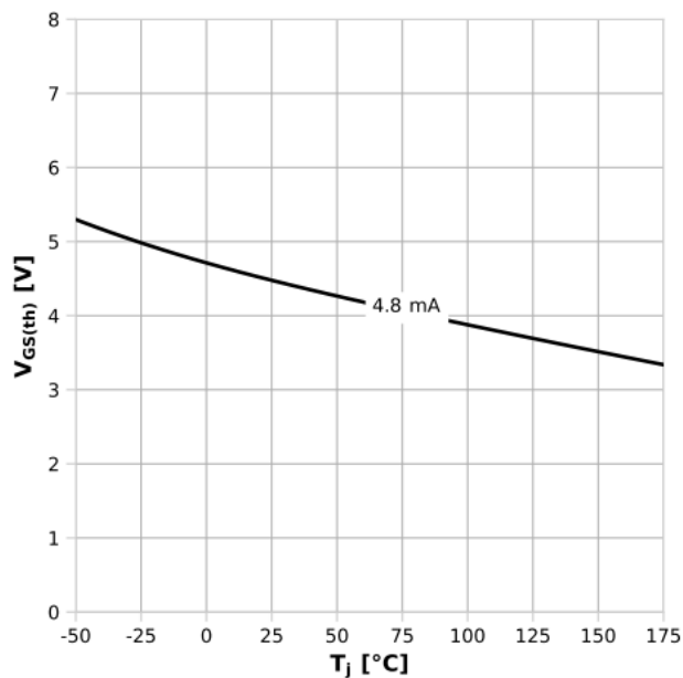
Diagram 18: Typ. gate threshold voltage
