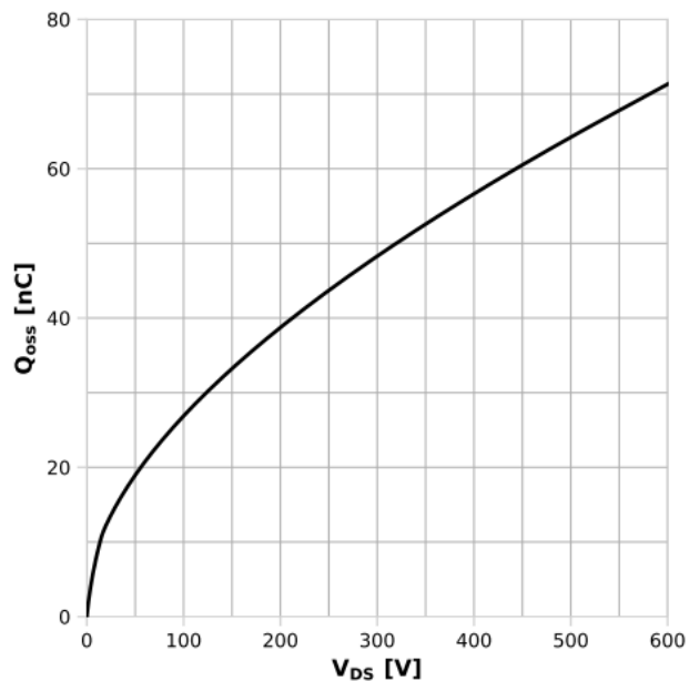
Diagram 17: Typ. Qoss output charge
