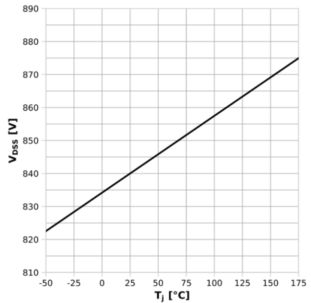
Diagram 14: Drain-source breakdown voltage
