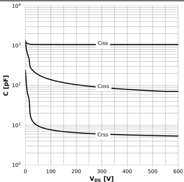
Diagram 15: Typ. capacitances
