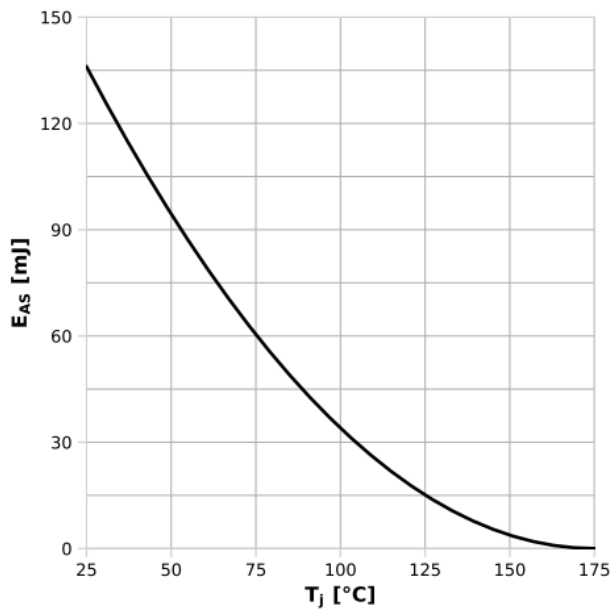
Diagram 13: Avalanche energy
