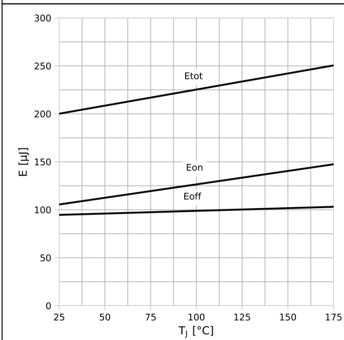
Diagram 21: Typ. Switching Losses vs T_J
