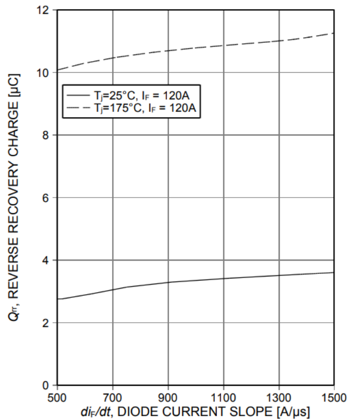
Figure 22. Typical reverse recovery charge as a function of diode current slope ( V_R=400\text{V} , Dynamic test circuit in Figure E)
