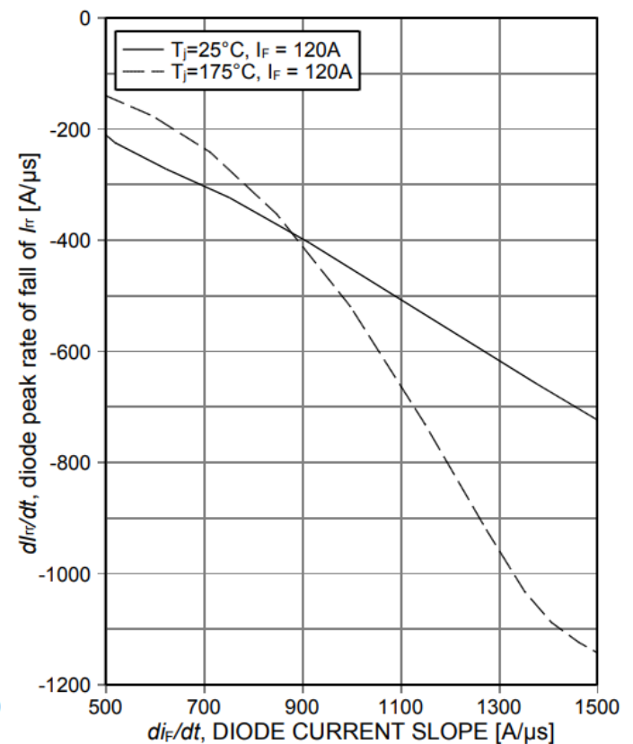
Figure 24. Typical diode peak rate of fall of reverse recovery current as a function of diode current slope ( V_R=400\text{V} , Dynamic test circuit in Figure E)
