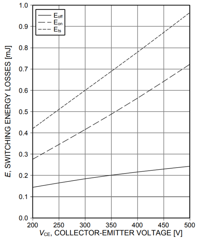
Figure 14. Typical switching energy losses as a function of collector emitter voltage (inductive load, T_{j1}=150^\circ C , V_{GE}=15/0V , I_C=20A , r_G=15\Omega , Dynamic test circuit in Figure E)
