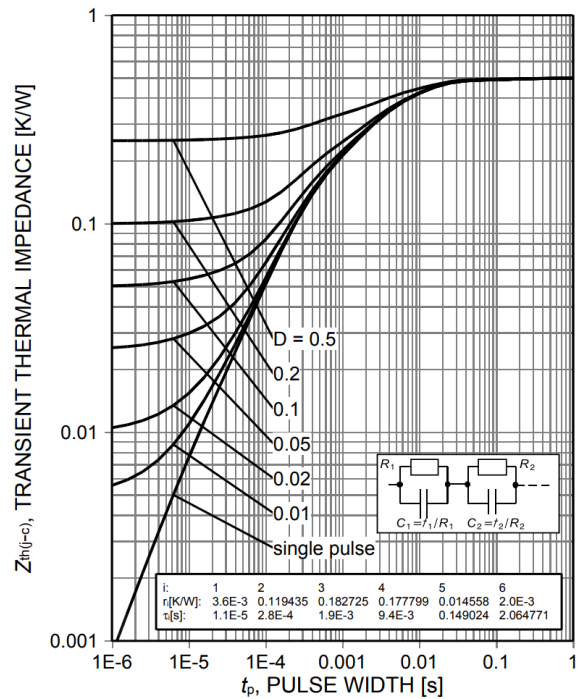
Figure 17. IGBT transient thermal impedance ( D=t_p/T )
