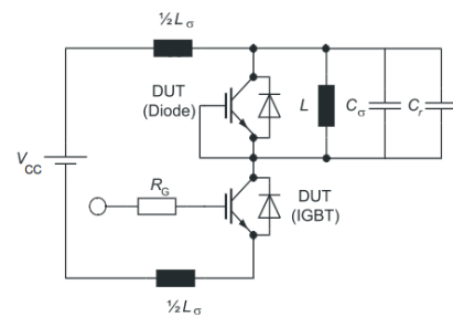
Figure E. Dynamic test circuit
