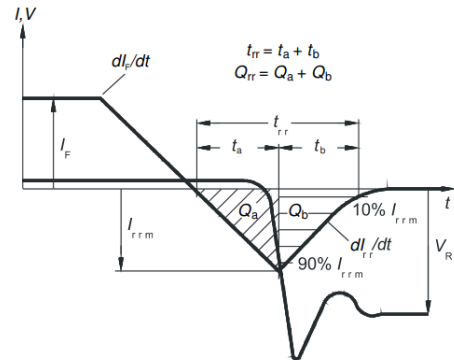
Figure C. Definition of diode switching characteristics
