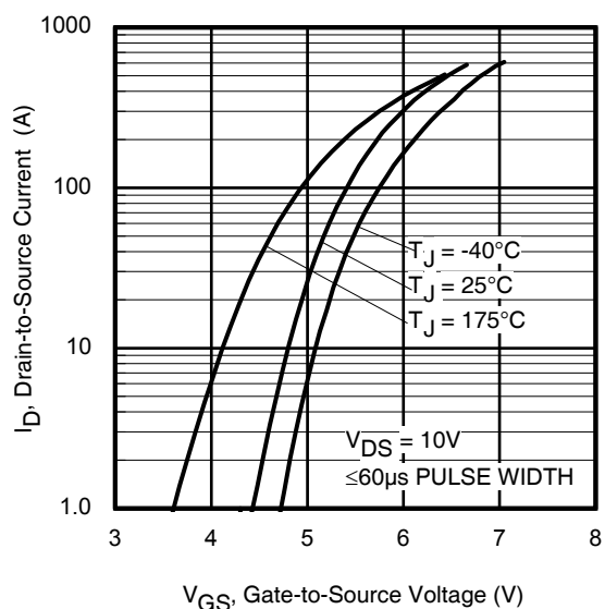
Fig 5. Transfer Characteristics
