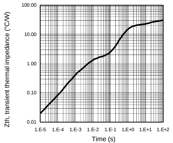
Figure 8 – Transient thermal impedance ( ^{\circ}C/W ) Vs time (s)
