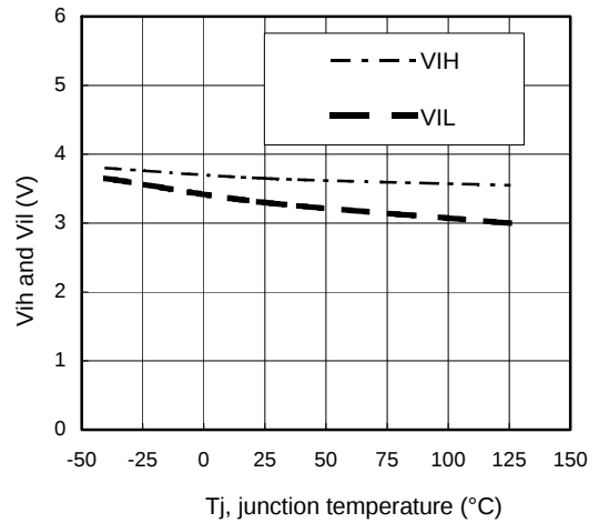
Figure 6 – V_{ih} and V_{il} (V) Vs T_j ( ^{\circ}C )
