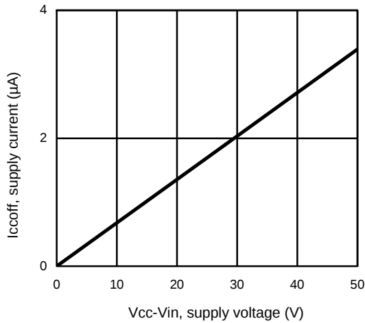
Figure 5 – I_{cc\ off}(\mu A) Vs V_{CC}-V_{in} (V)
