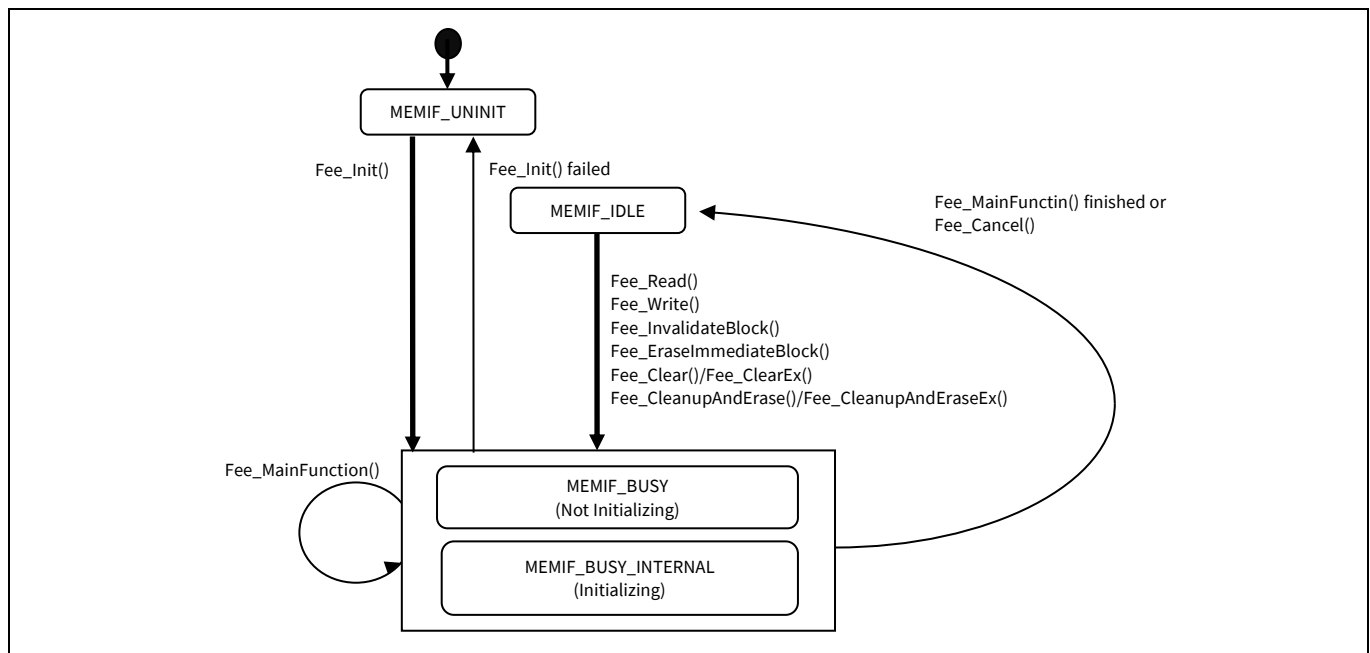
Figure 6 State machine of FEE
