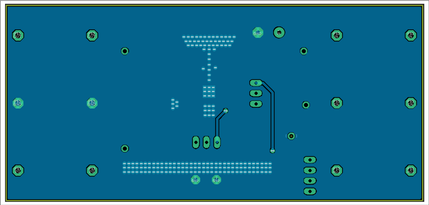
Figure 5 Bottom layer
