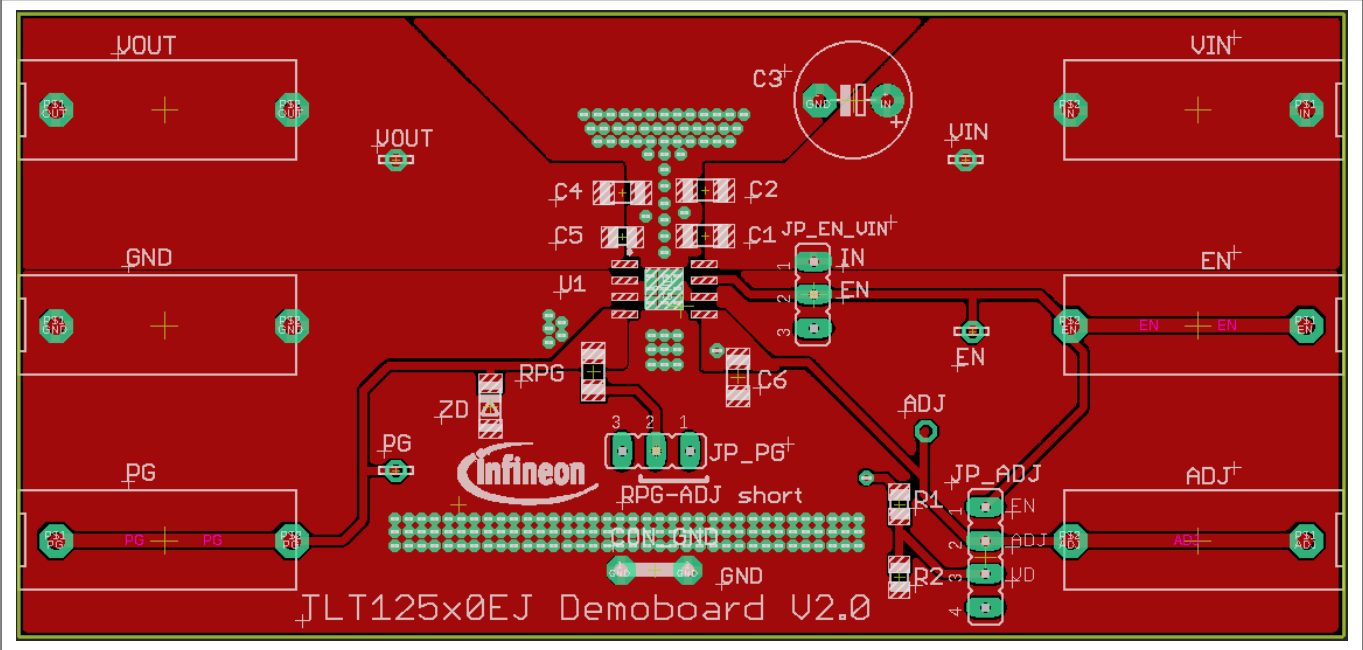
Figure 4 Top layer
