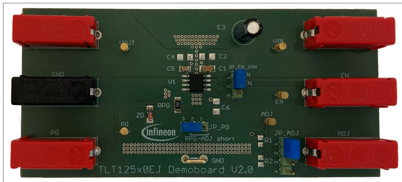
Figure 2 OPTIREG™ linear voltage regulator TLT125D0EJ demoboard
