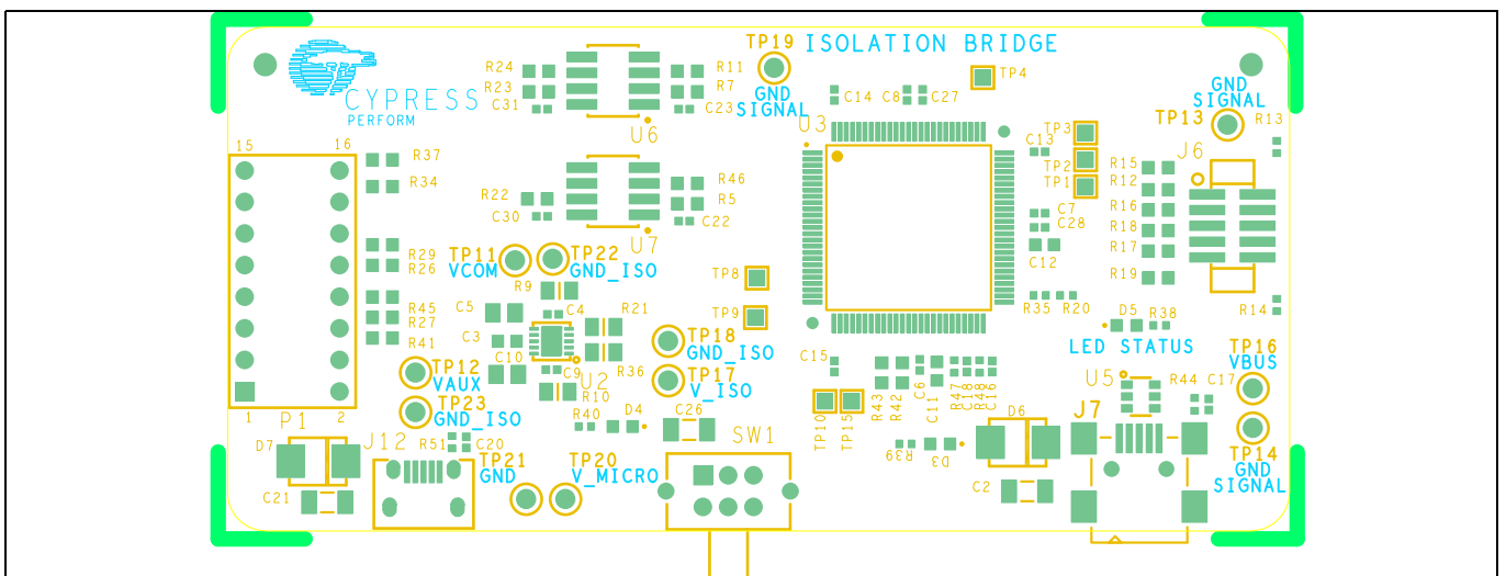
Figure 37 Primary silkscreen
