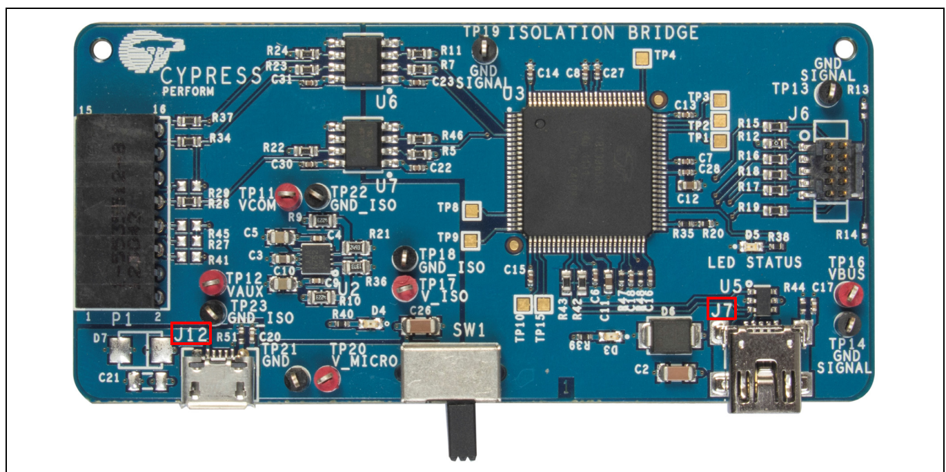
Figure 7 Isolation bridge
