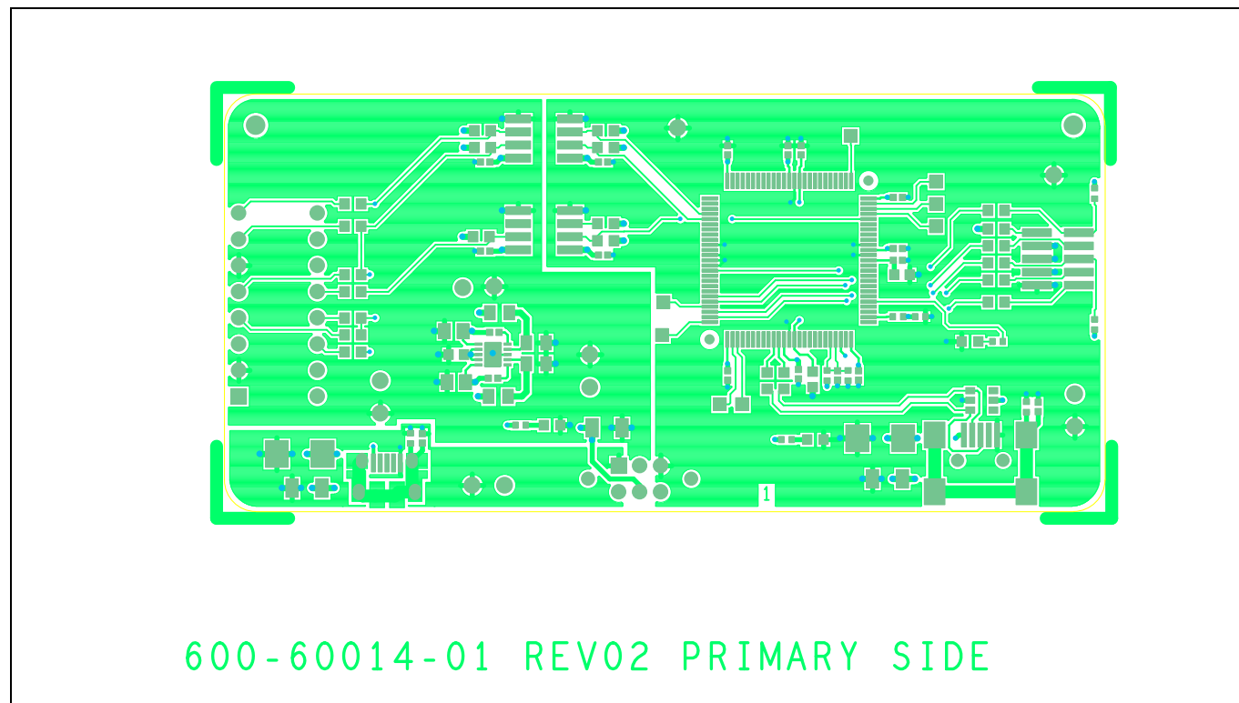
Figure 33 Primary side
