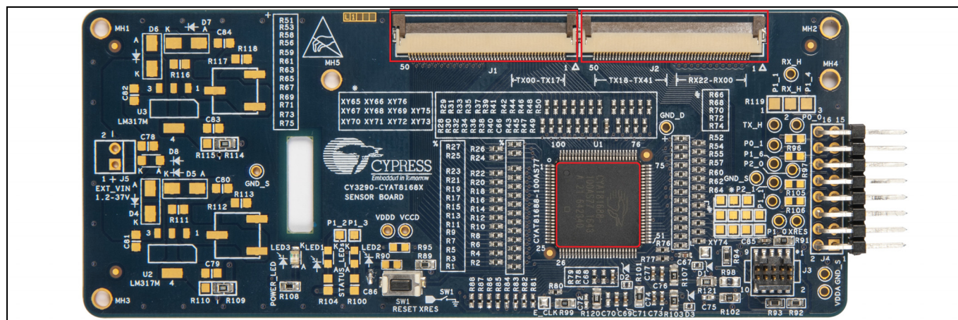
Figure 6 CYAT8168X EVK sensor board
