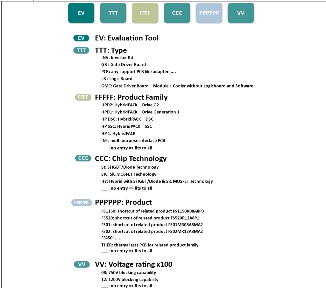
Figure 3 Type designation tree for the HybridPACK™ power module evaluation tools.
