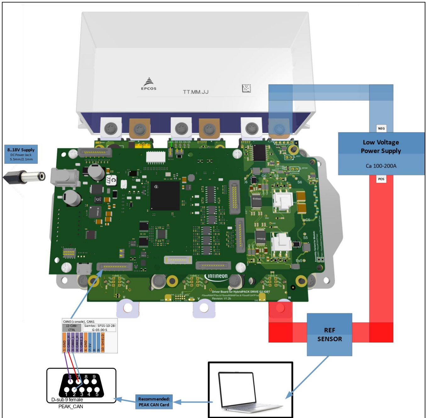
Figure 12 Setup for Gain Parameter Calibration of the Current Sensors (shown only example for phase W).
