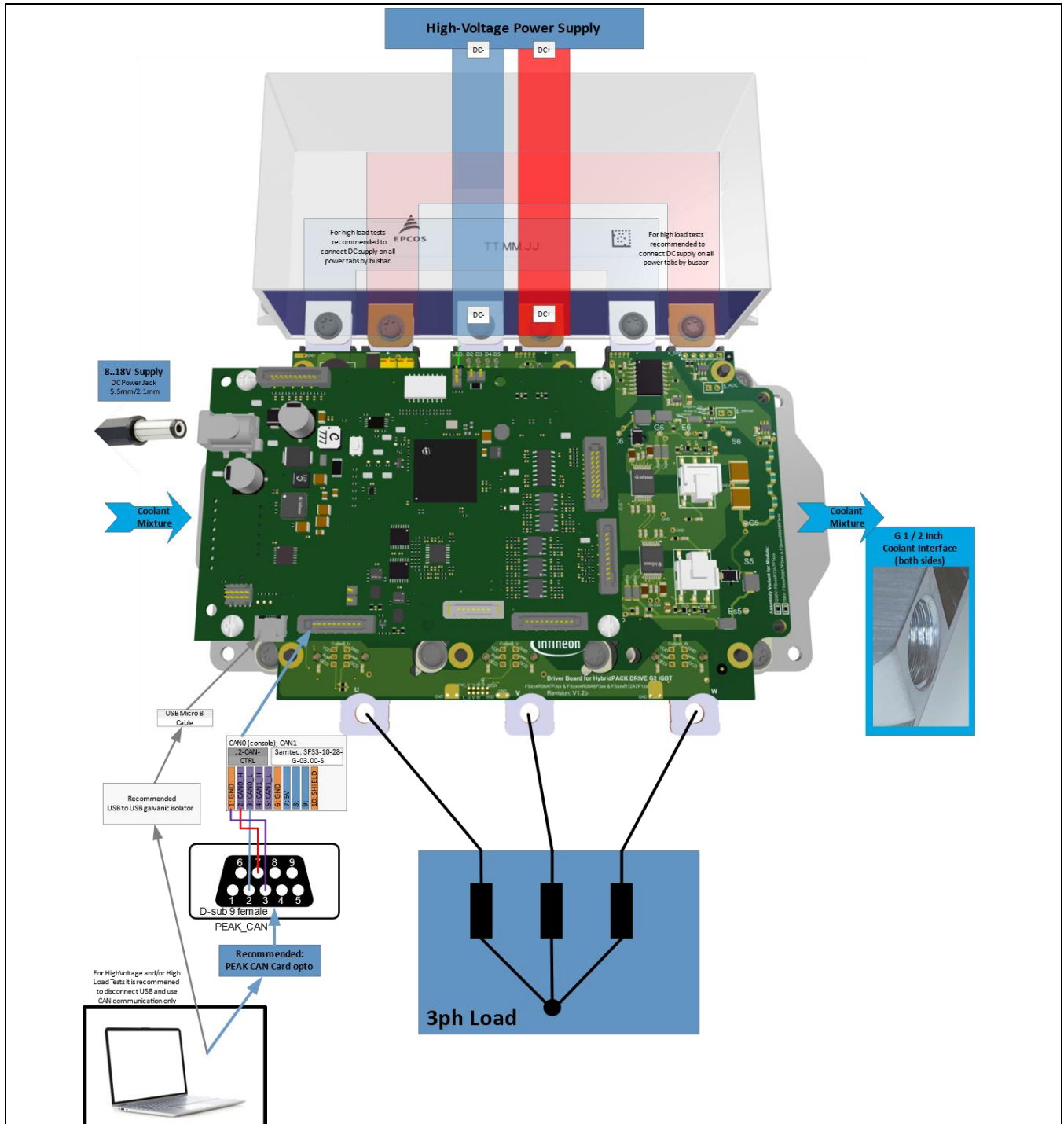
Figure 7 Typical setup for Inverter Load Tests.
