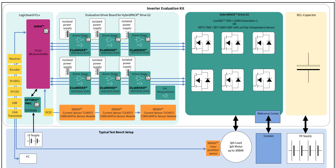
Figure 1 Block Diagram of the Inverter Evaluation Kits for HybridPACK™ Drive G2 power modules
