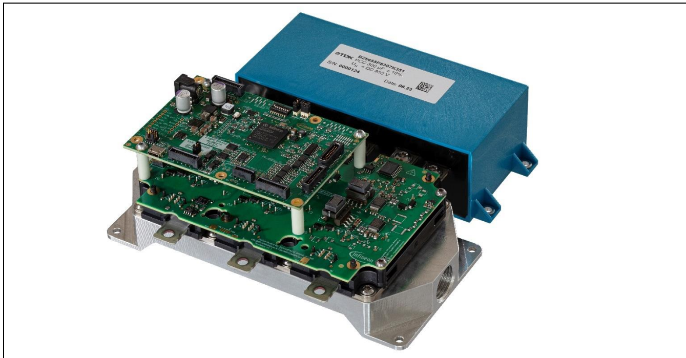
Figure 2 Inverter Evaluation Kits for HybridPACK™ Drive G2 power modules. Versions with latest IGBT and SIC MOSFET chipsets at 750V and 1200V blocking capability are available. See also Table 2.
