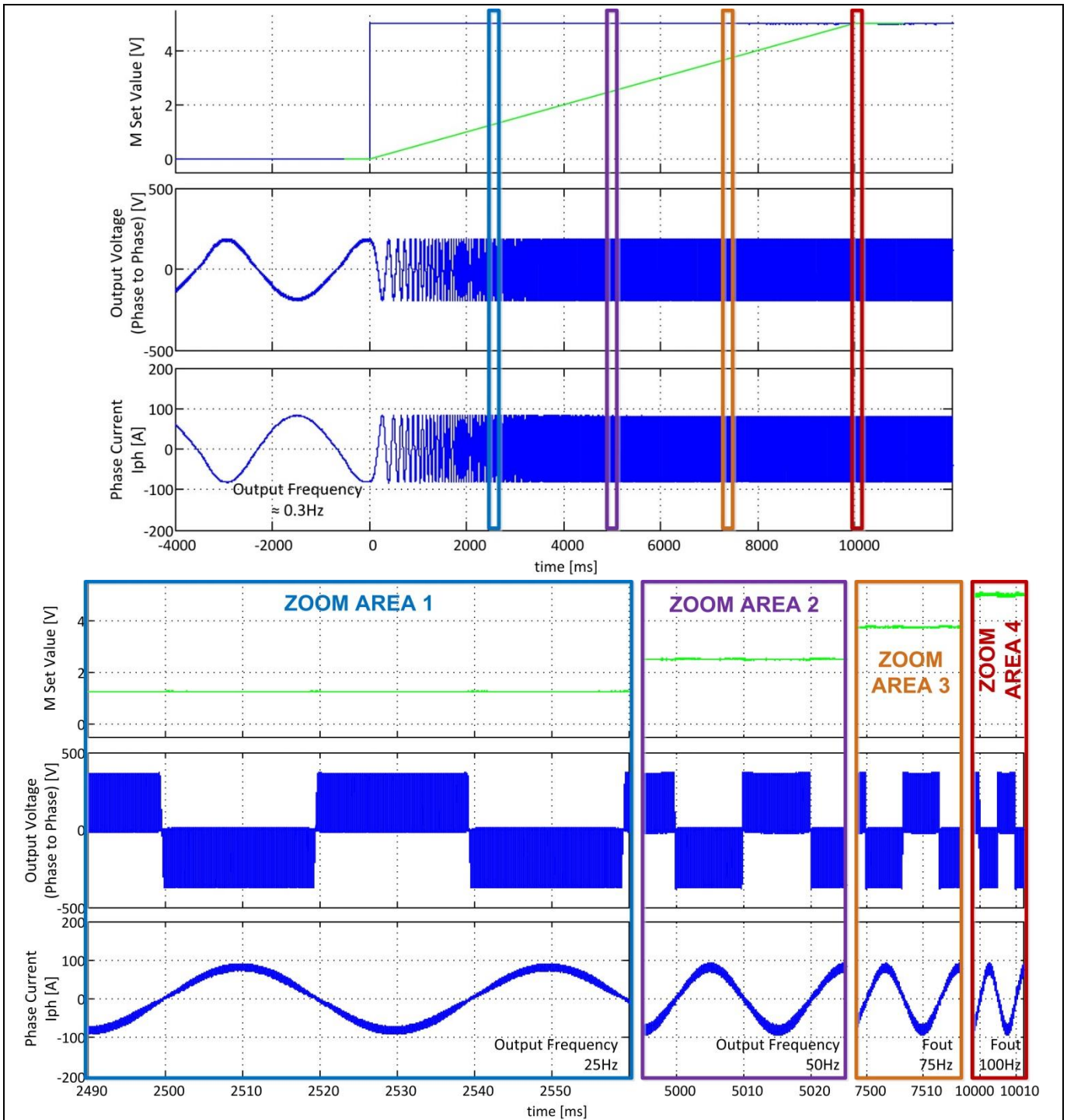
Figure 10 Measured event, where operator changes the output frequency set value rapidly from 0V to 5V. The internal ramp function ensures a smooth transition from nearly 0Hz to 100Hz output.
