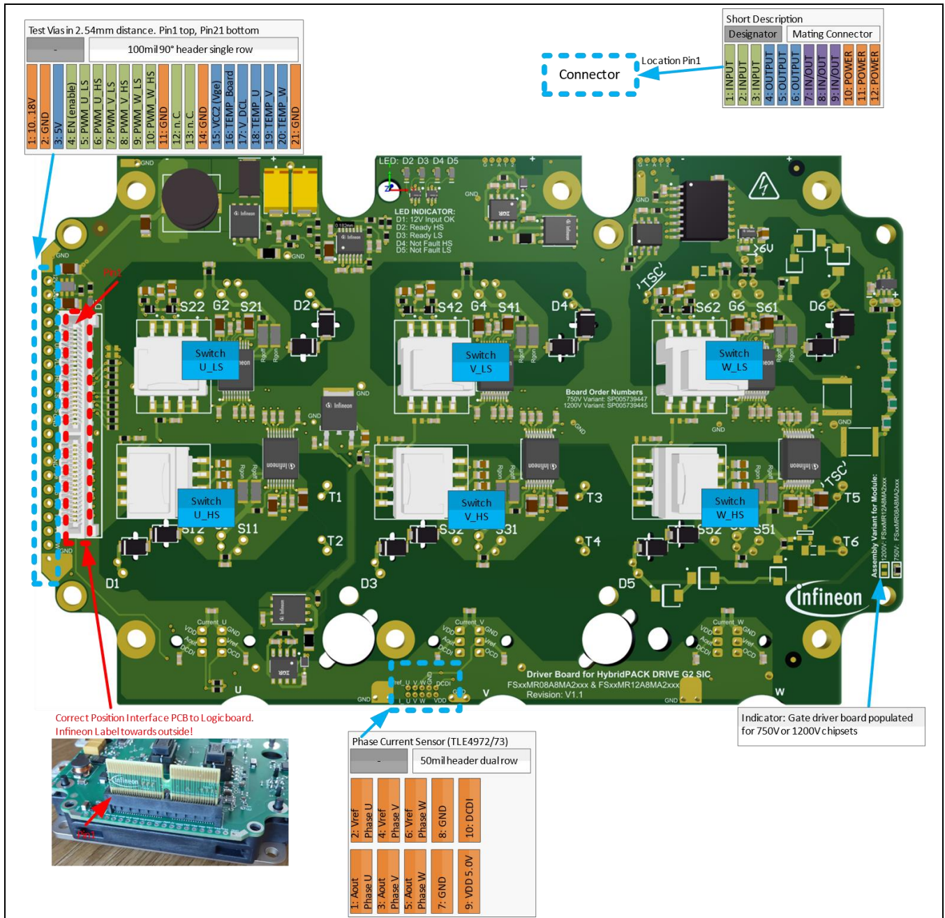
Figure 6 Connectors of Gate Driver Boards (SIC MOSFET Versions).
