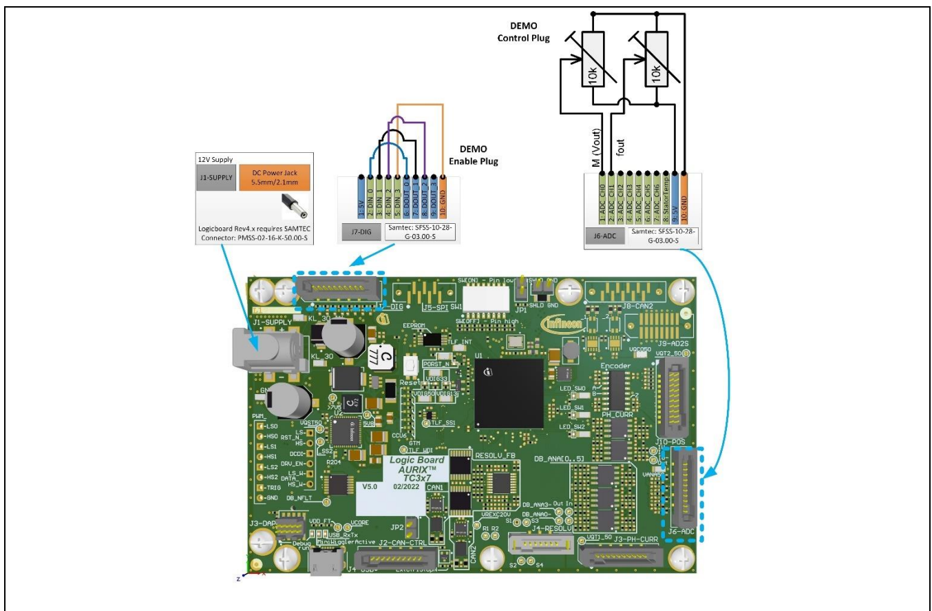
Figure 8 Connection to enable the DEMO-MODE in order to operate the inverter kit without communication in open loop operation.
