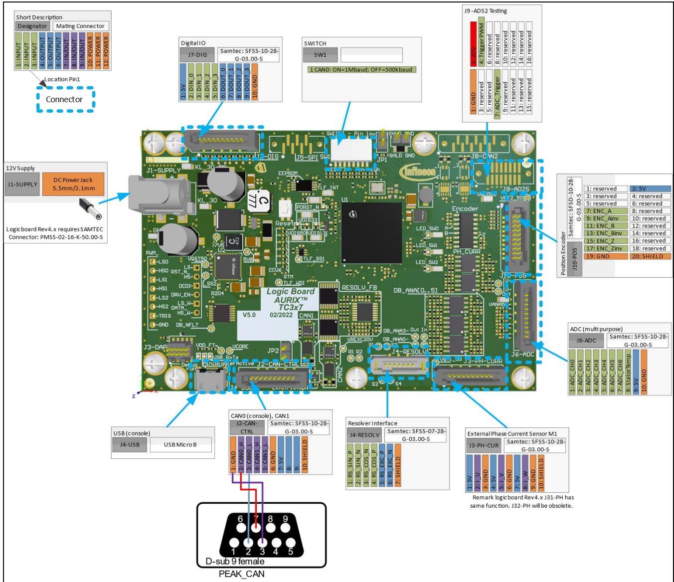
Figure 4 Connectors of Logicboard LB5.x.
