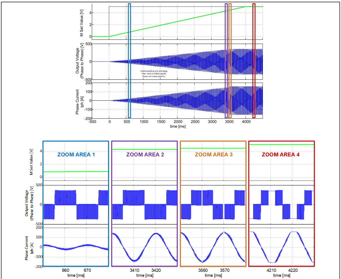
Figure 9 Measured event, where operator changes the modulation set value rapidly from 0V to 5V. The internal ramp function ensures a smooth transition from 0% to 100% modulation index. The modulated phase to phase output voltage is consequently increased within the limits of the applied system working voltage.
