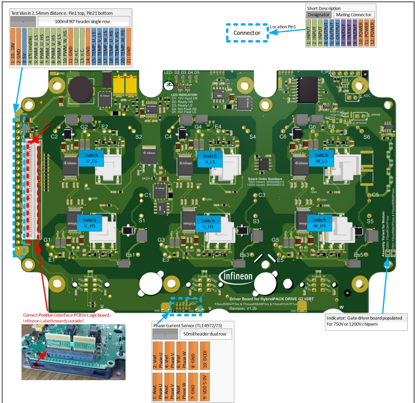
Figure 5 Connectors of Gate Driver Boards (IGBT Versions).
