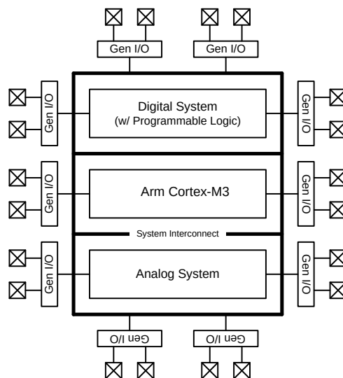
Figure 6. PSoC 5LP Block Diagram
