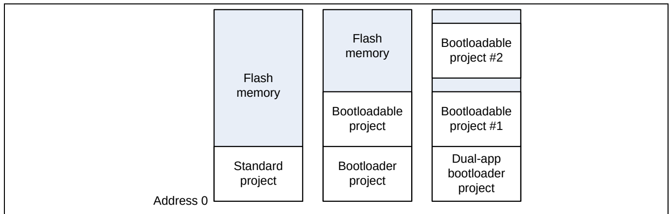
Figure 7 PSoC™ Creator projects and flash memory usage
