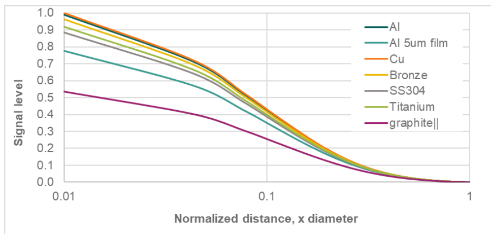
Figure 46 Electrical conductivity of metal as function of signal level and distance/diameter
