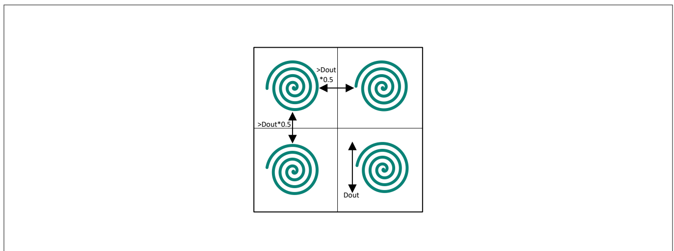
Figure 33 Coil-to-coil spacing for a four-button use case
