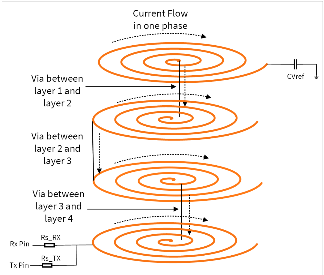
Figure 35 Different layers of the coil arranged to allow current flow to be in the same direction in each layer
