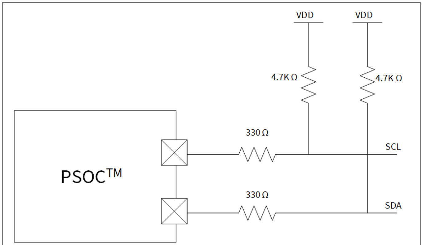
Figure 50 Series resistors on communication lines
