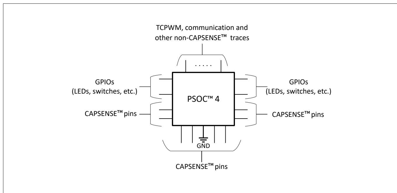
Figure 19 Recommended: Port isolation for communication, CAPSENSE™, and LEDs
