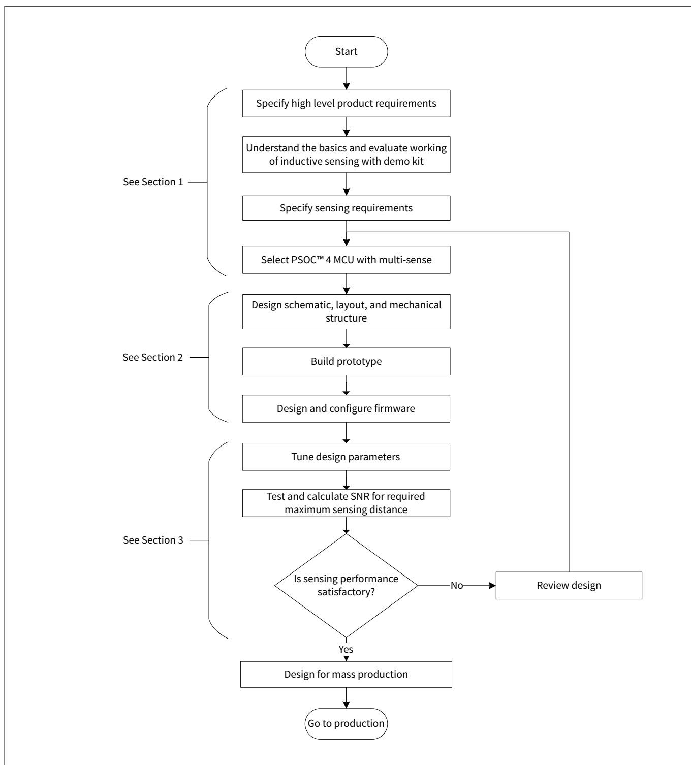
Figure 11 Recommended ISX system design flow
