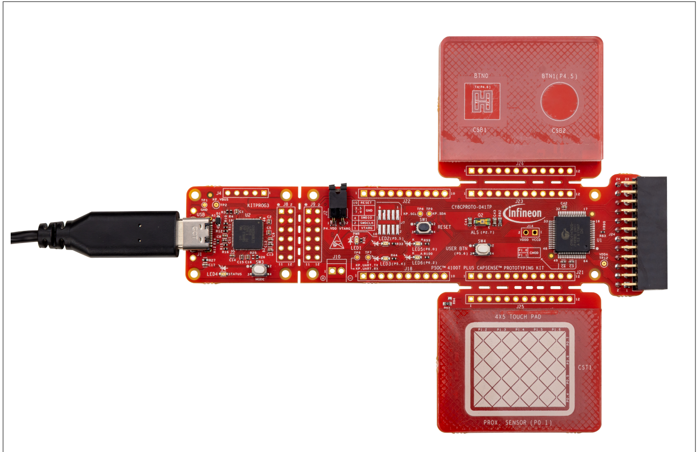
Figure 8 CY8CPROTO-041TP kit
