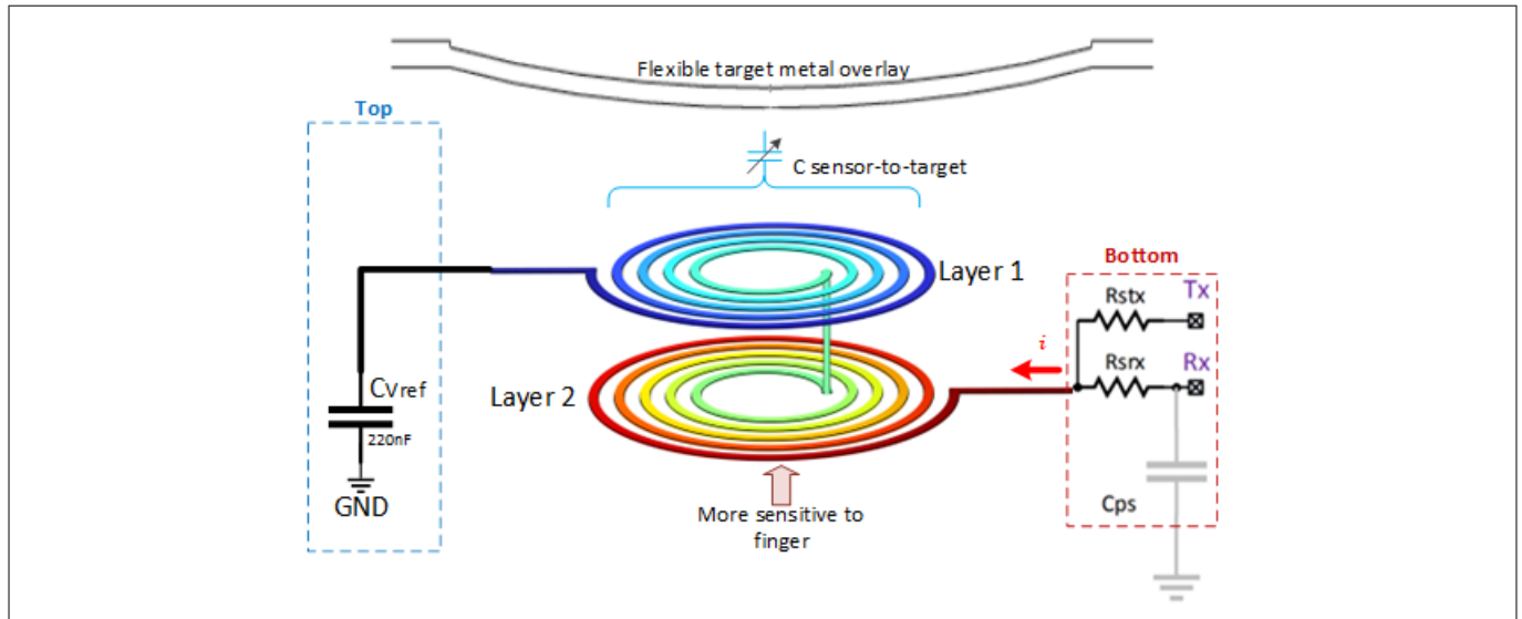
Figure 36 Two-layer inductors in a series configuration with a flexible metal target
