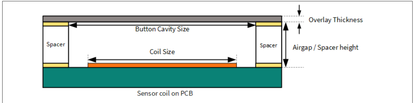
Figure 40 Mechanical construction of a touch-over-metal button
