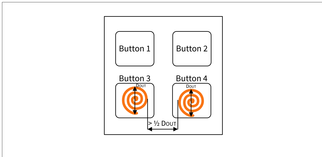
Figure 49 4-button system
