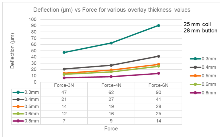
Figure 45 Deflection values ( in \mu\text{m} ) for different overlay thickness values and button (coil) sizes
