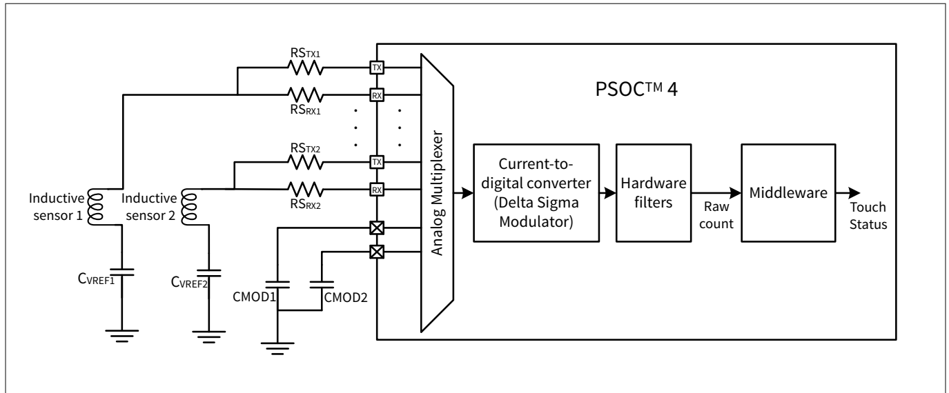
Figure 3 Simplified diagram of PSOC™ 4 MSCLP with flyback inductive sensor
