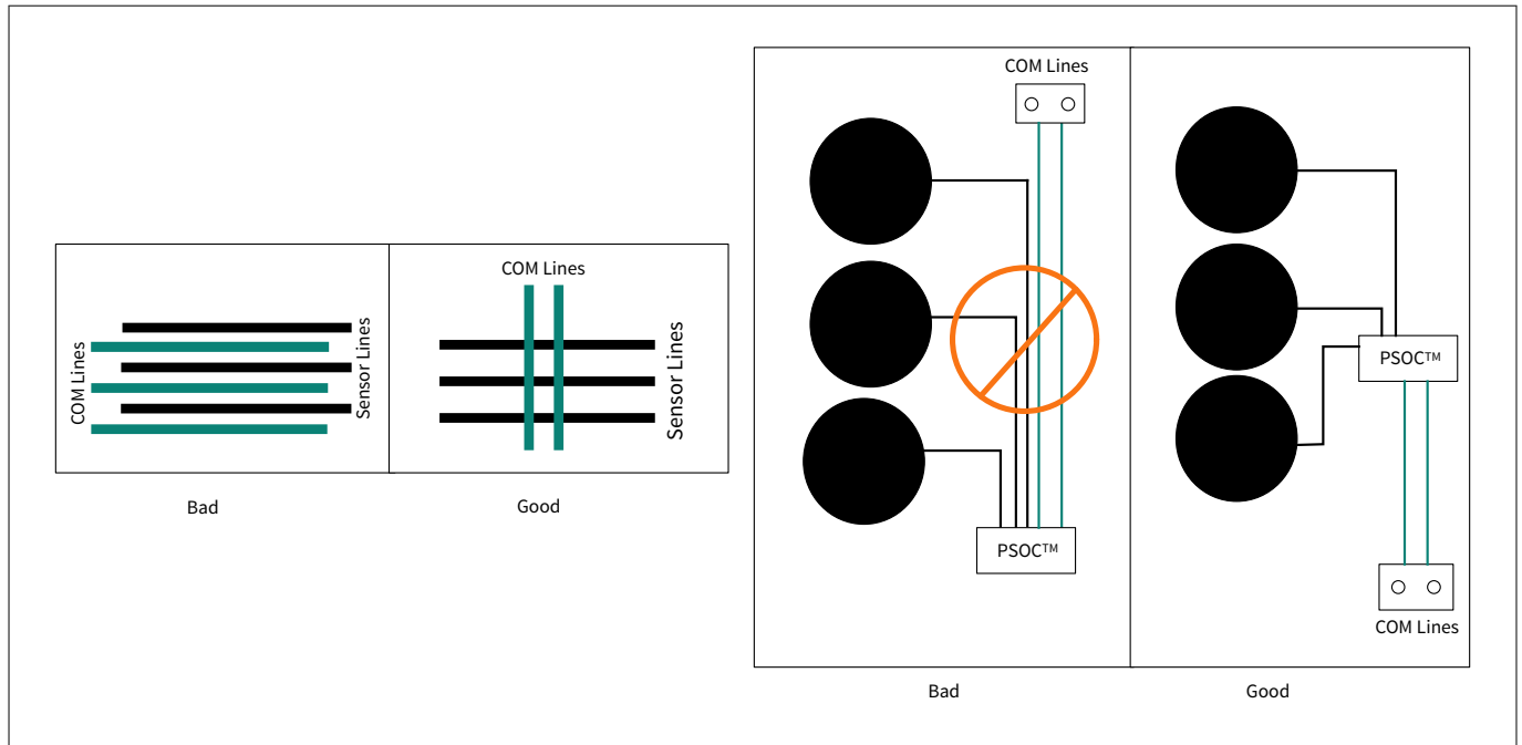
Figure 34 Routing of the sensor and communication lines
