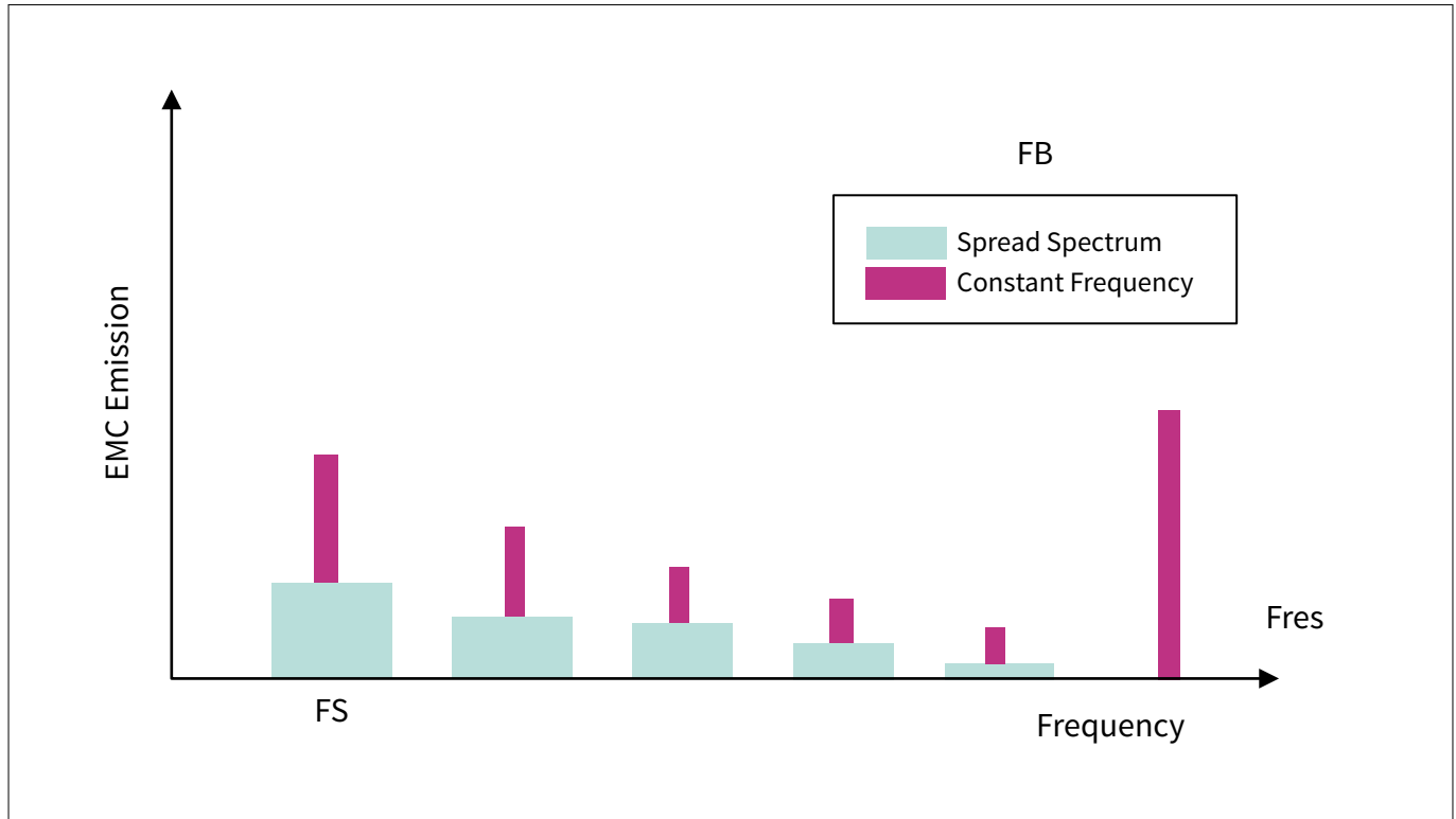
Figure 51 EMI for typical inductive sensor with constant and SS frequency
