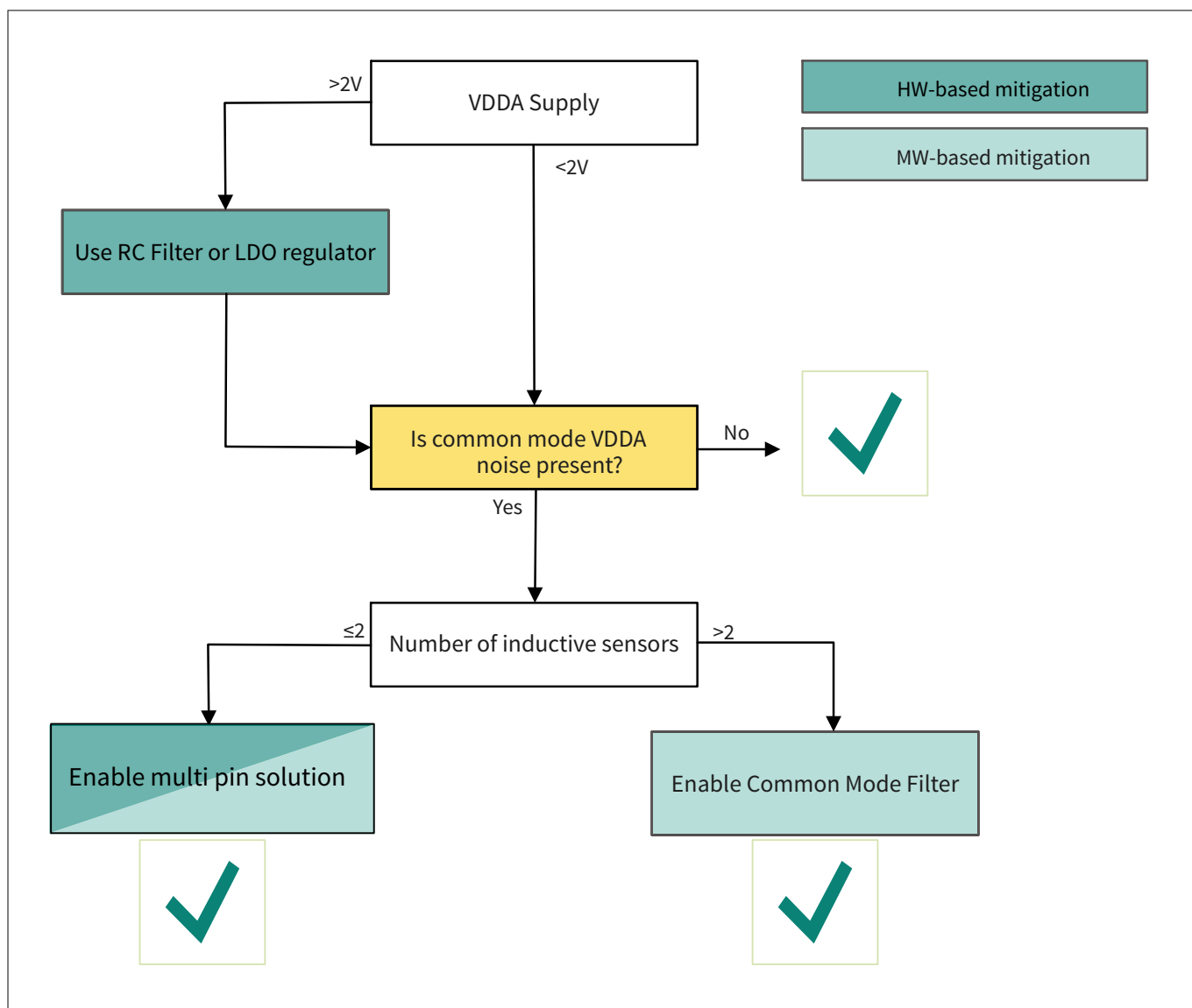
Figure 72 Power supply noise mitigation decision tree
