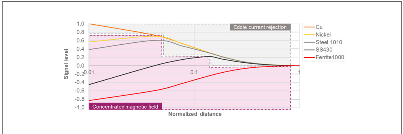
Figure 47 Properties of ferromagnetic materials as function of signal level and distance
