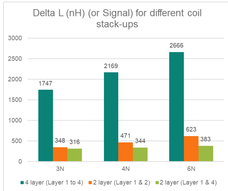
Figure 30 Signal (in terms of dL) for three different coil stack-ups
