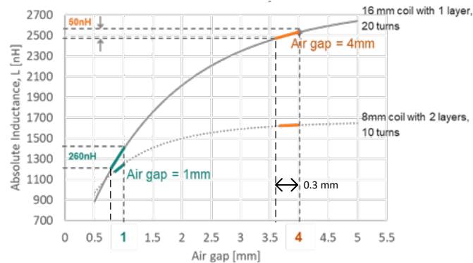
Figure 28 Absolute inductance response for 1-layer and 2-layers sensor coils
