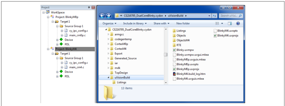
Figure 28 Resultant µVision project window and project files
