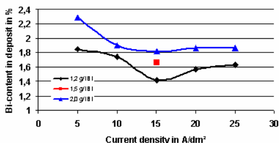
Figure 1 – The Bi content decreases by a maximum of 0,4 % in a range of 20 A / dm 2
