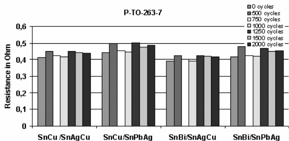
Figure 10 – Resistance of daisy chains for TO263 in various material combinations up to 2000 temperature cycles (slow ramp rate)
