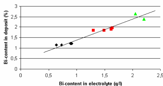
Figure 3 – An increases by 1 g/l Bi in the electrolyte corresponds with an increase of nearly 1 % Bi in the deposit
