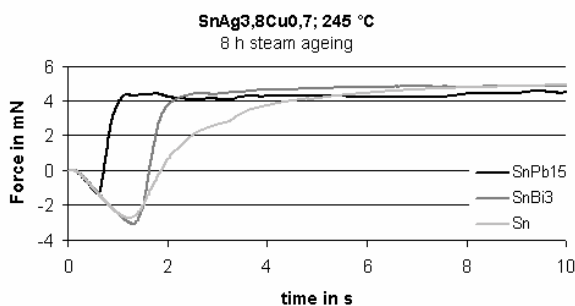
Figure 7 – Wetting of SnPb15, SnBi3 and Sn plated on copper after 8 ha steam ageing with SnAgCu solder
