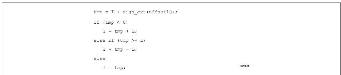
Figure 2-5 Circular Addressing Index Algorithm
