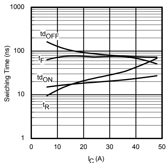
Fig. 15 - Typ. Switching Time vs. I_C T_J = 175^\circ\text{C} ; L = 0.40\text{mH} ; V_{CE} = 400\text{V} , R_G = 10\Omega ; V_{GE} = 15\text{V}
