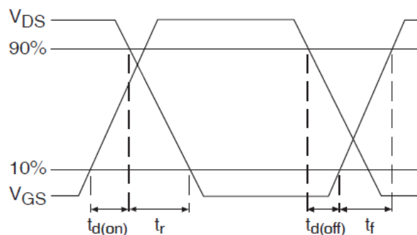
Fig 15b. Switching Time Waveforms
