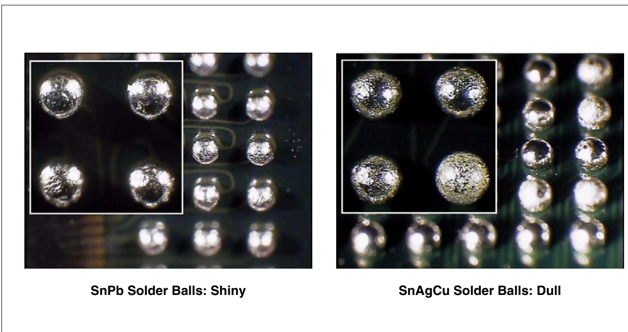
Figure 9 Comparison of Solder Ball Appearance
