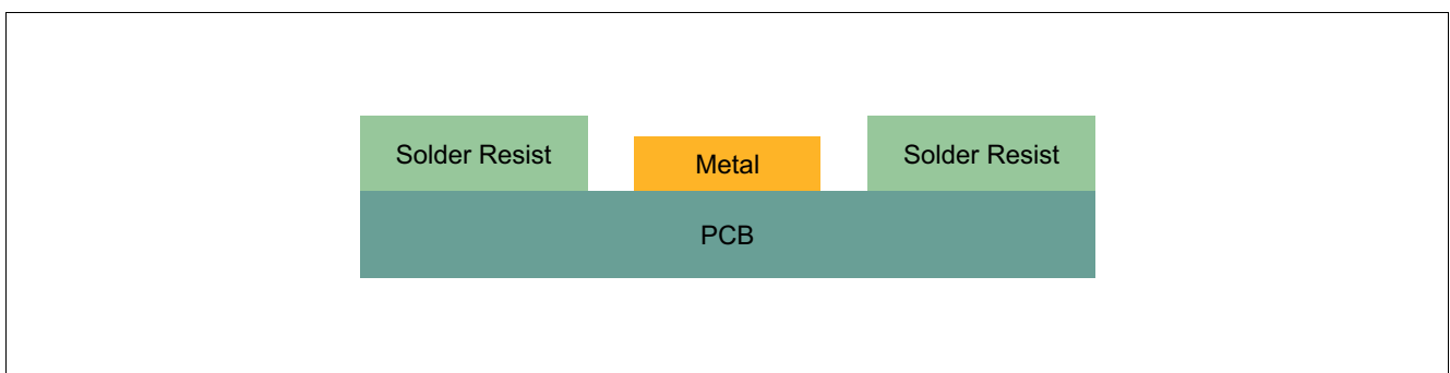
Figure 4 NSMD Pad
