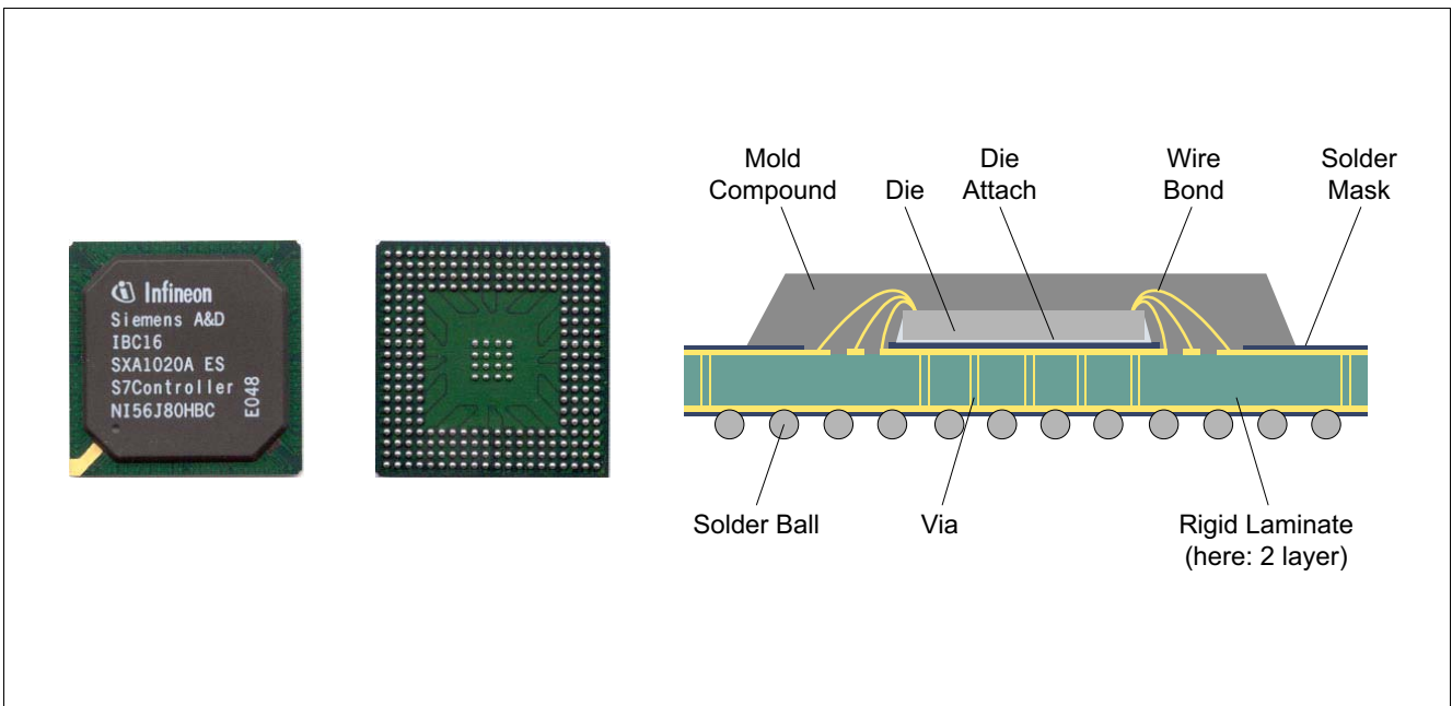
Figure 1 P(G)-BGA Top View, Bottom View and Cross Section
