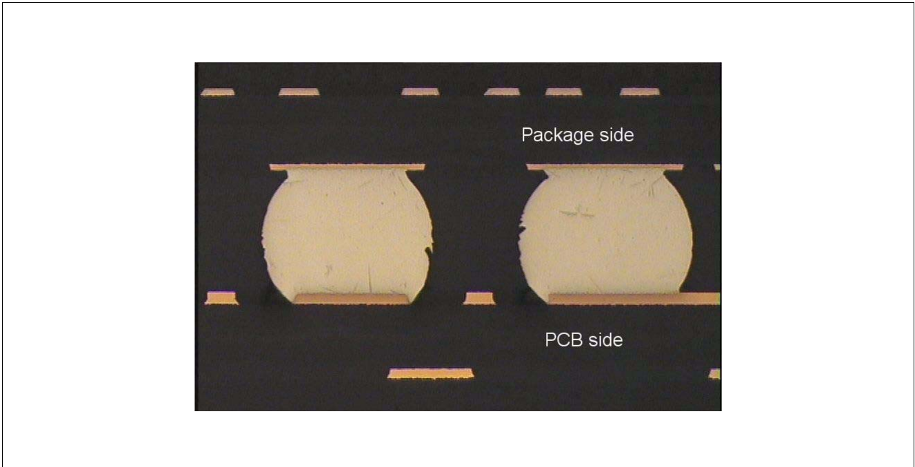
Figure 8 Sample Cross Section of BGA Solder Balls
