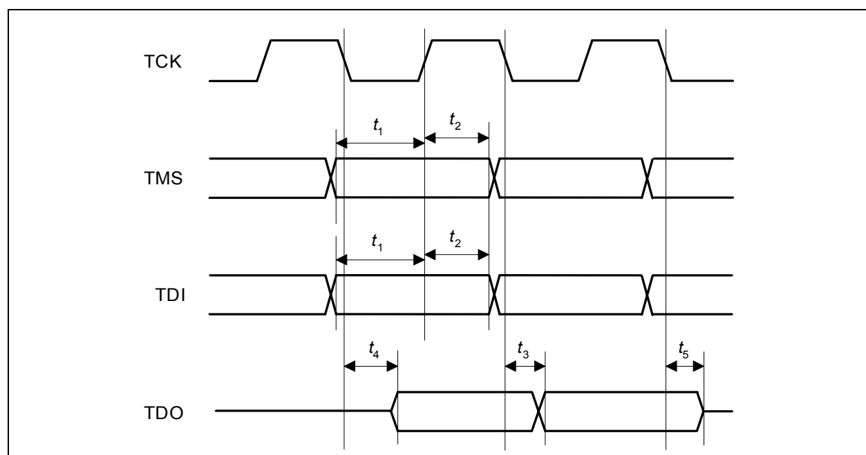
Figure 43 JTAG Timing
