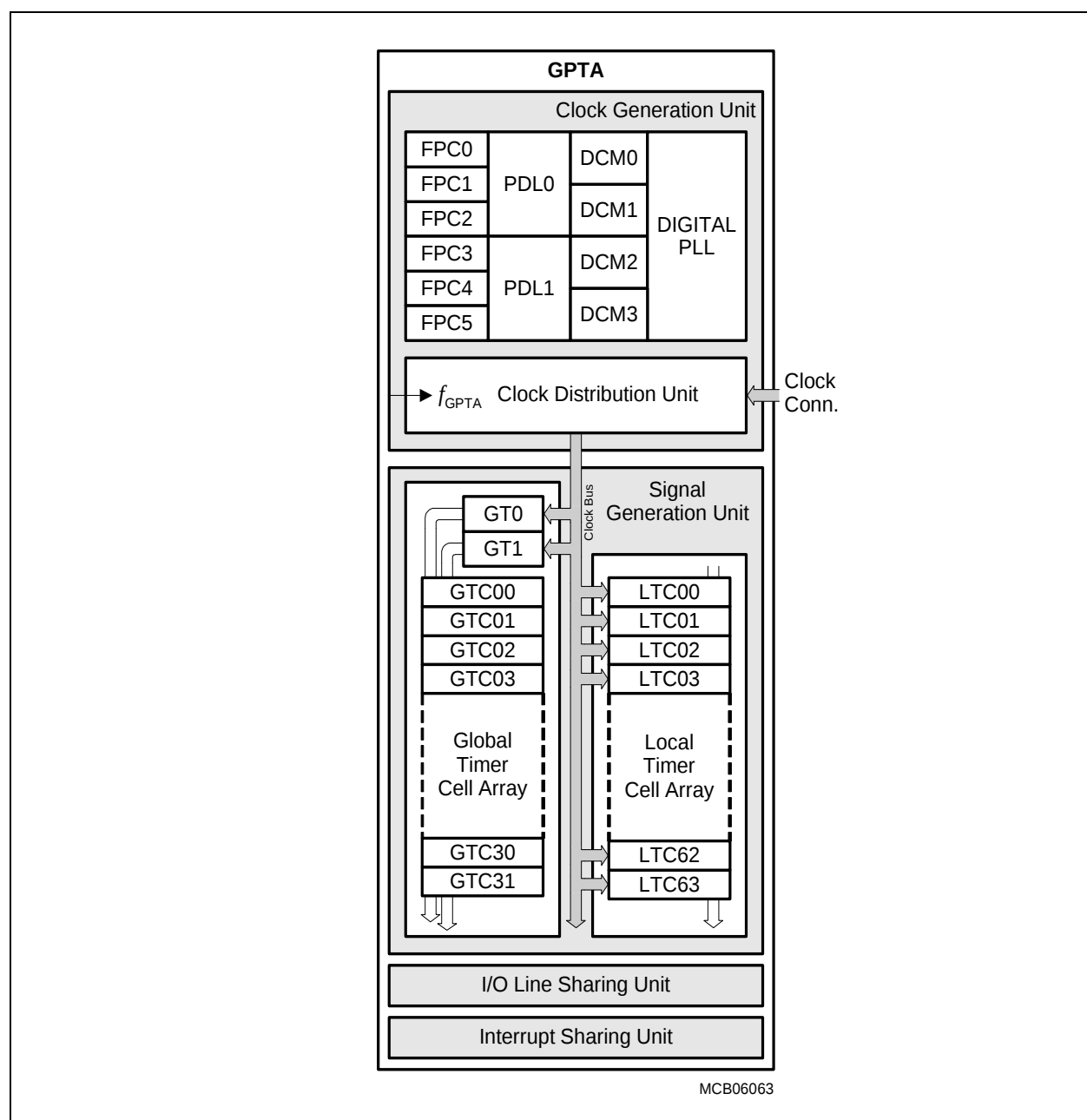
Figure 3-9 Block Diagram of the GPTA Module
