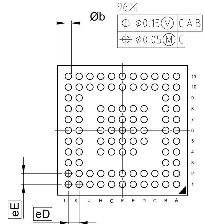
Bottom view
