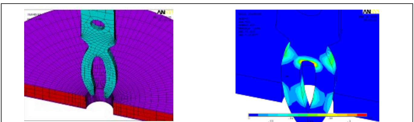
Figure 1 Opened PressFIT Pin
