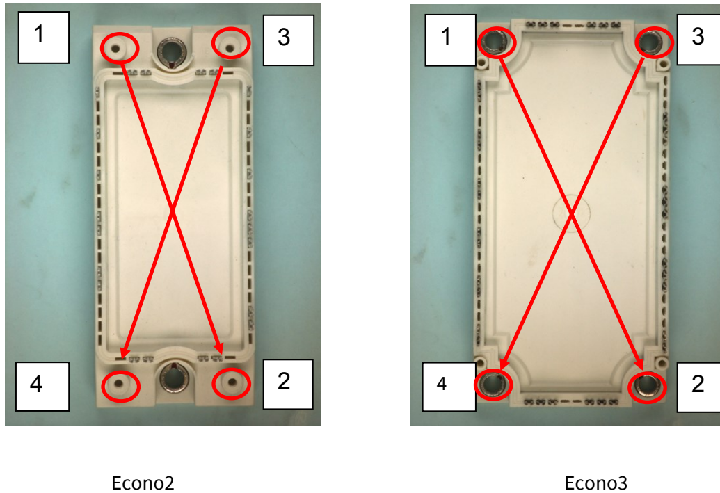
Figure 8 Figure 14 PCB mounting stand-offs of an EconoPACK™ module
