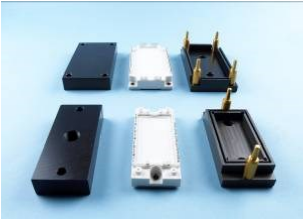
Figure 7 Press-in tools of Econo 2/3
