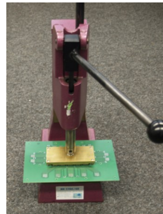
Pressing-out the module
