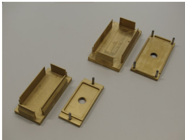
Press-out tools of Econo2/3 module
