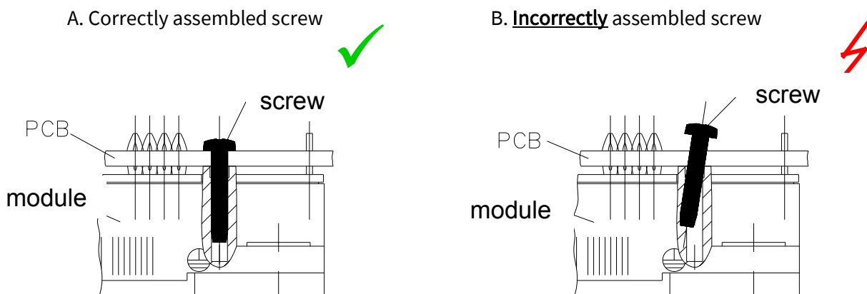
Figure 9 (Left) Correctly assembled screw into the mounting stand-off. (Right) Incorrectly positioned screw in the mounting stand-off
