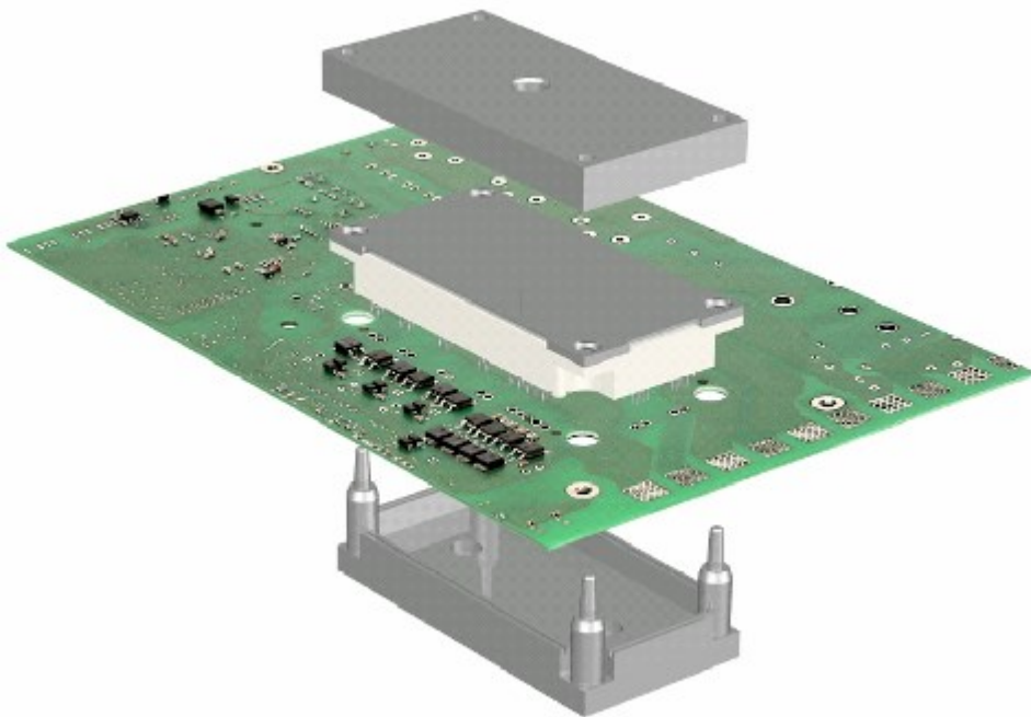
Figure 3 Mounting of a PCB onto an Econo module
