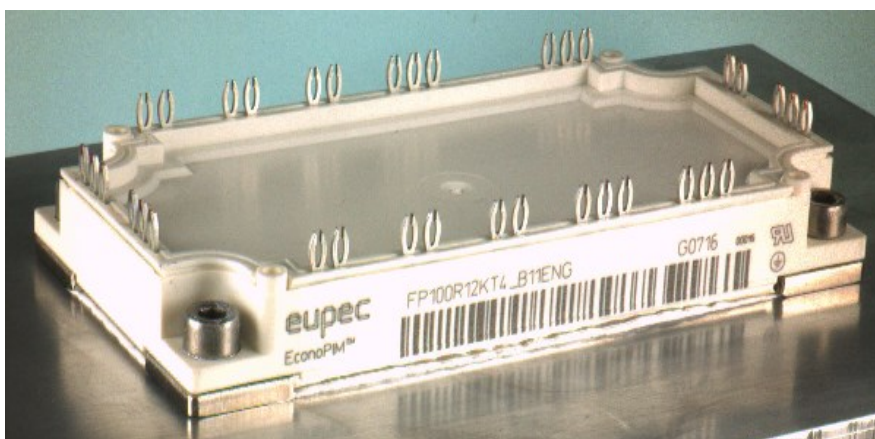
Figure 10 Mounted EconoPIM™ module with thermal compound oozing out on the side
