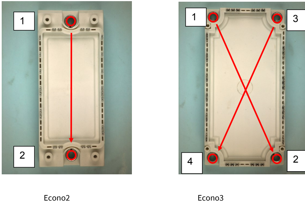
Figure 13 Tightening sequence to mount the module
