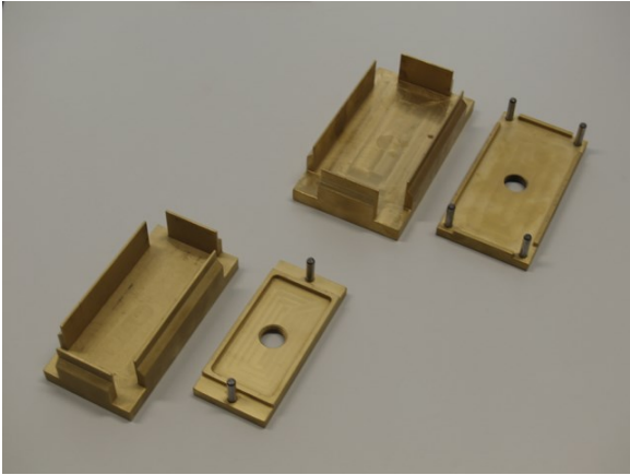
Press-out tools of Econo 2/3
