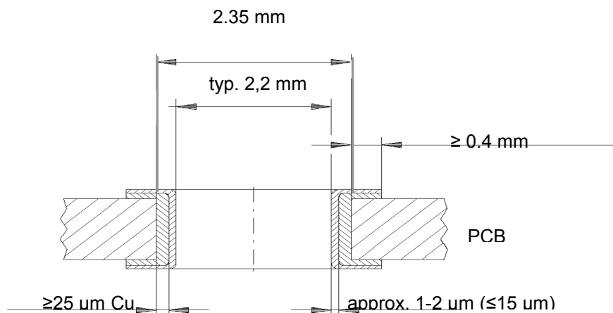
Figure 2 Construction of the PCB
