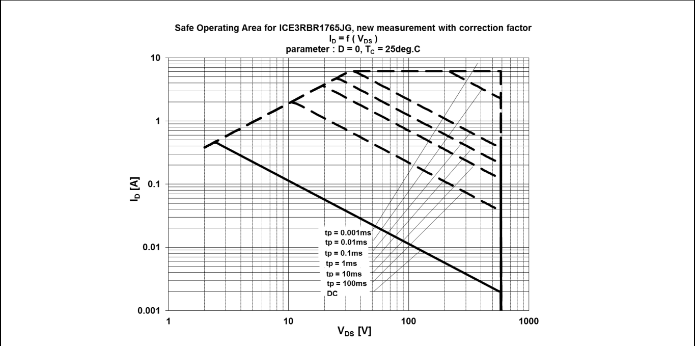
Figure 28 Safe Operating Area (SOA) curve for ICE3RBR1765JG
