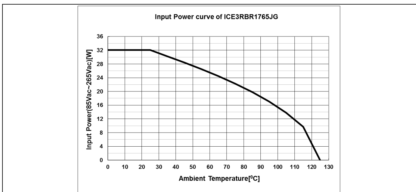
Figure 32 Input power curve V_{IN}=85 \sim 265 V_{AC} ; P_{in}=f(T_a)
