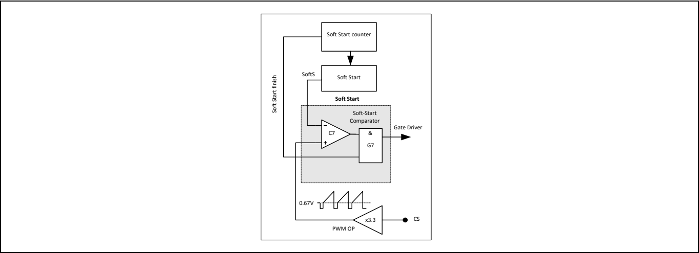
Figure 10 Soft Start
