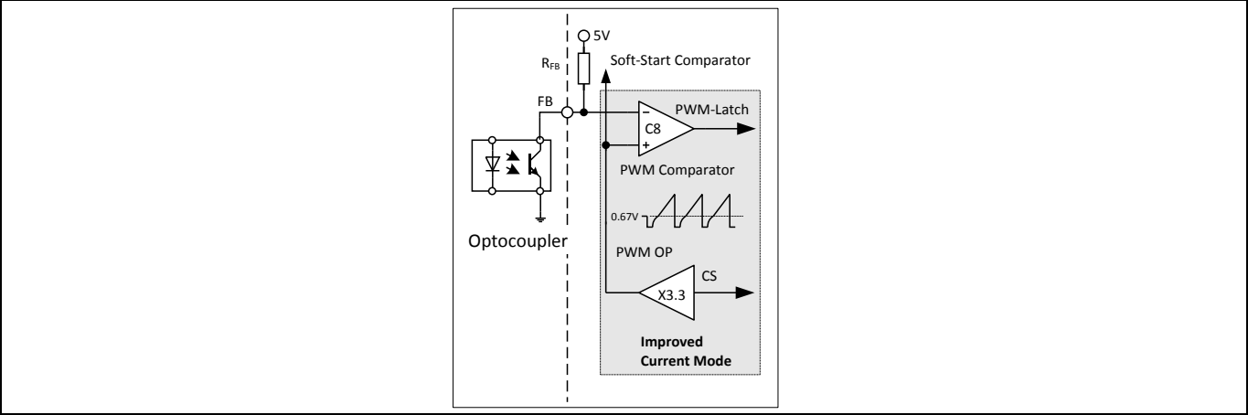
Figure 9 PWM Controlling
