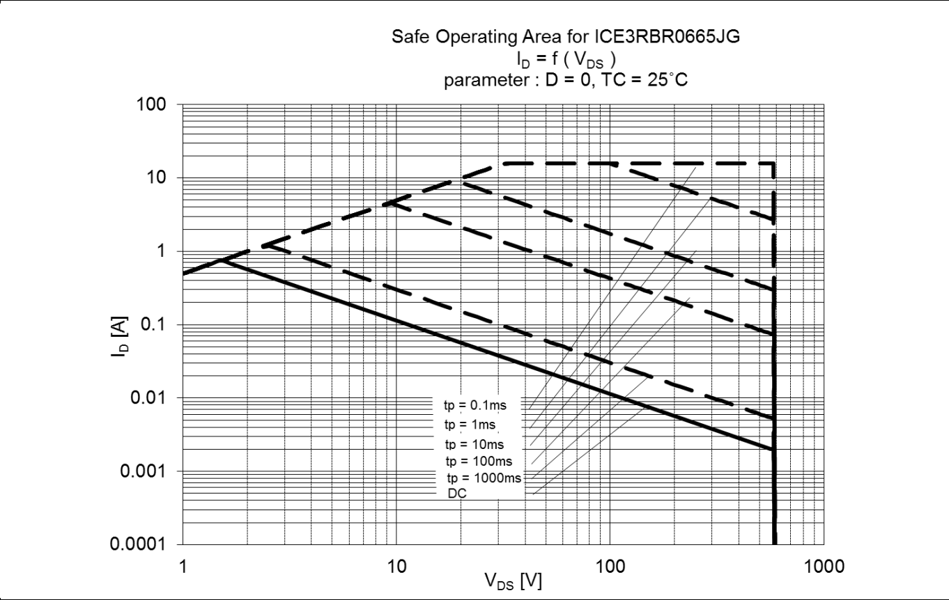
Figure 28 Safe Operating Area (SOA) curve for ICE3RBR0665JG
