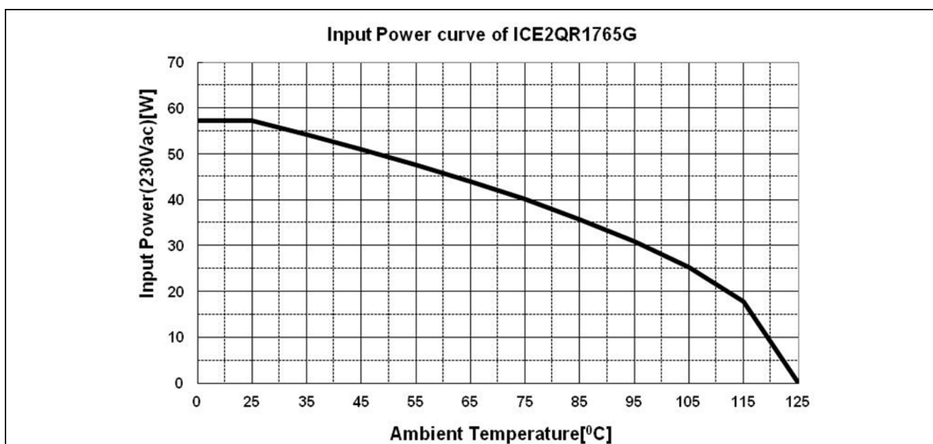
Figure 14 Input power curve V_{in}=230\text{ V}_{AC} ; P_{in}=f(T_a)
