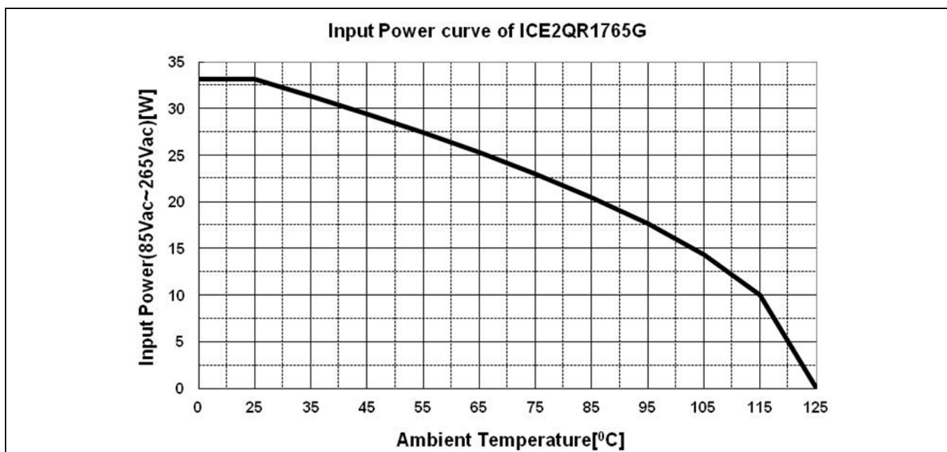
Figure 13 Input power curve V_{in}=85\sim 265\text{ V}_{AC} ; P_{in}=f(T_a)
