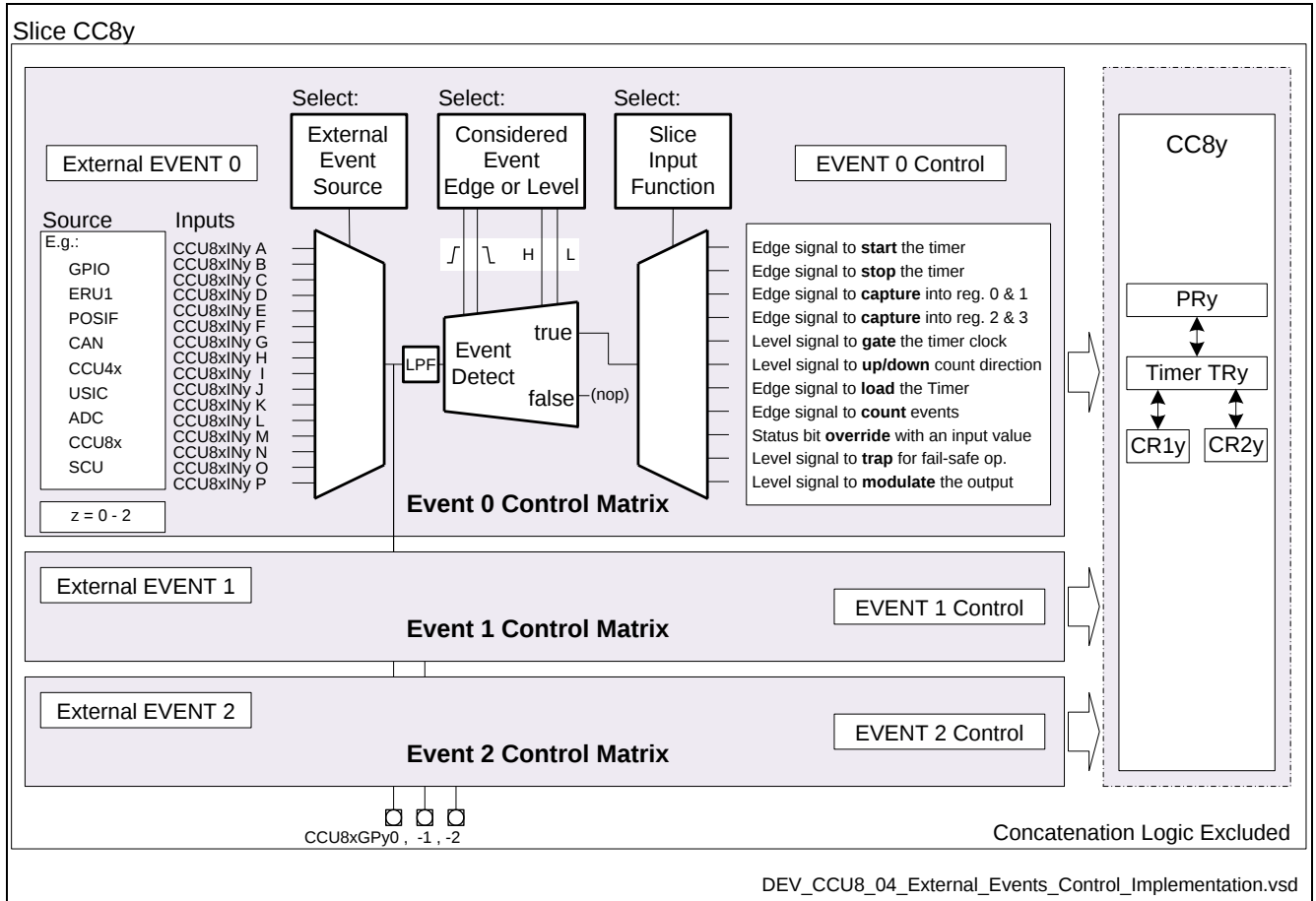
Figure 14 Block diagram of the external event control implementation
