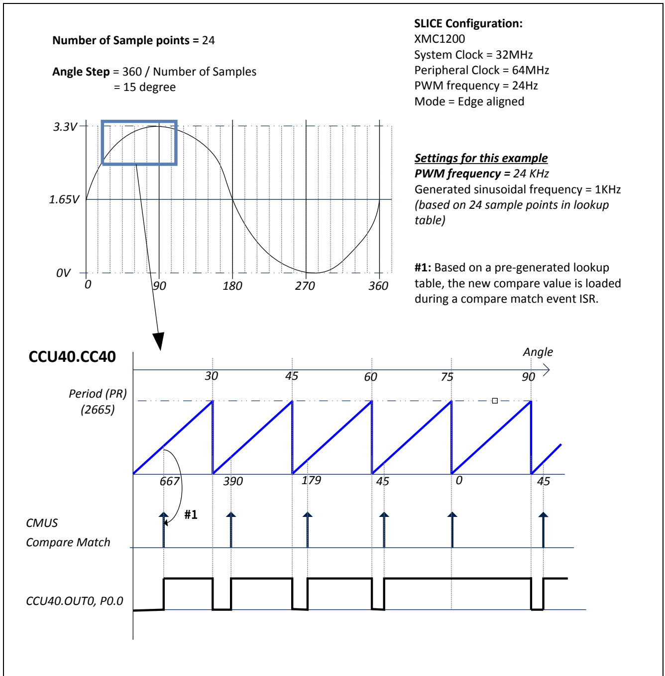
Figure 21 Example: generating a sinusoidal waveform
