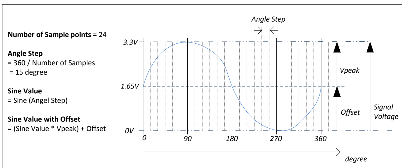
Figure 24 Deriving the sine value with reference to signal voltage
