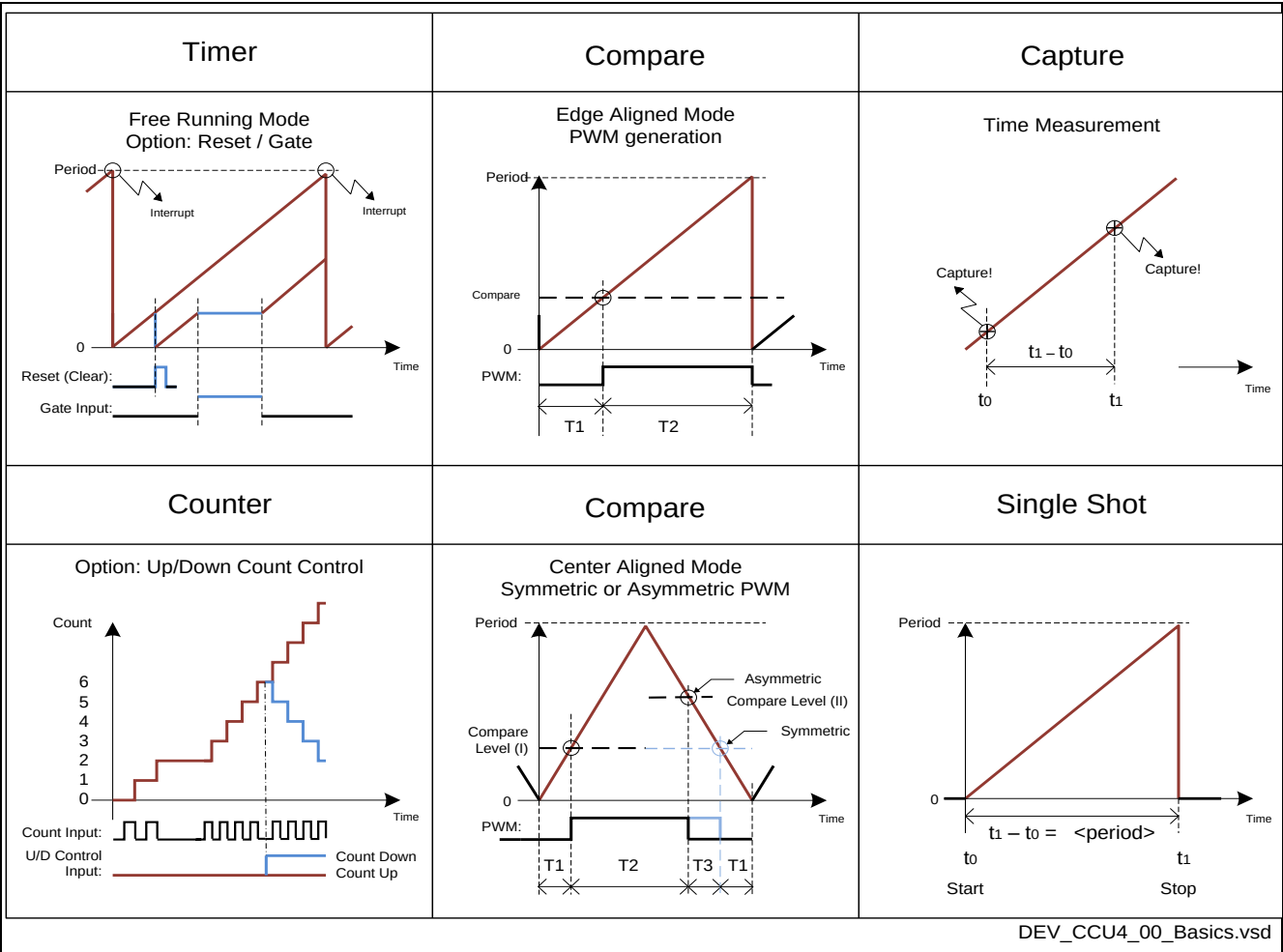
Figure 2 Basic functions of each timer slice
