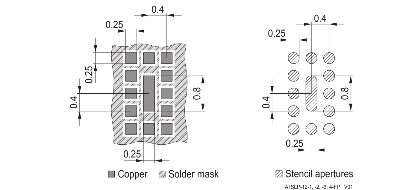
Figure 11: Footprint Recommendation
