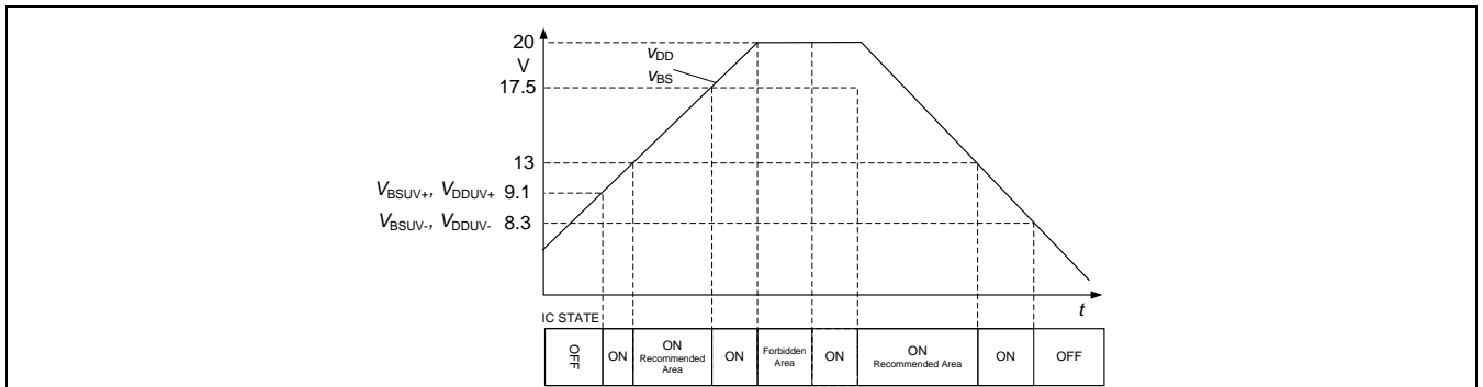
Figure 7 Typical areas of operation for MOSFET types
