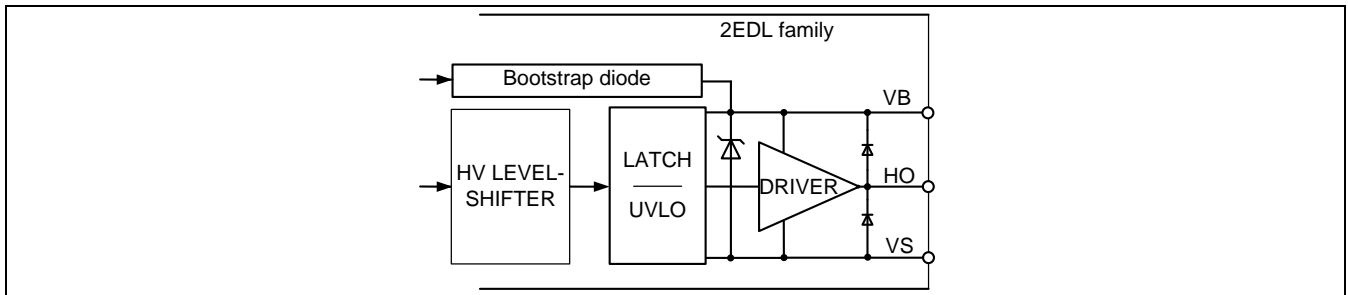
Figure 9 Structure of the low side gate drive section
