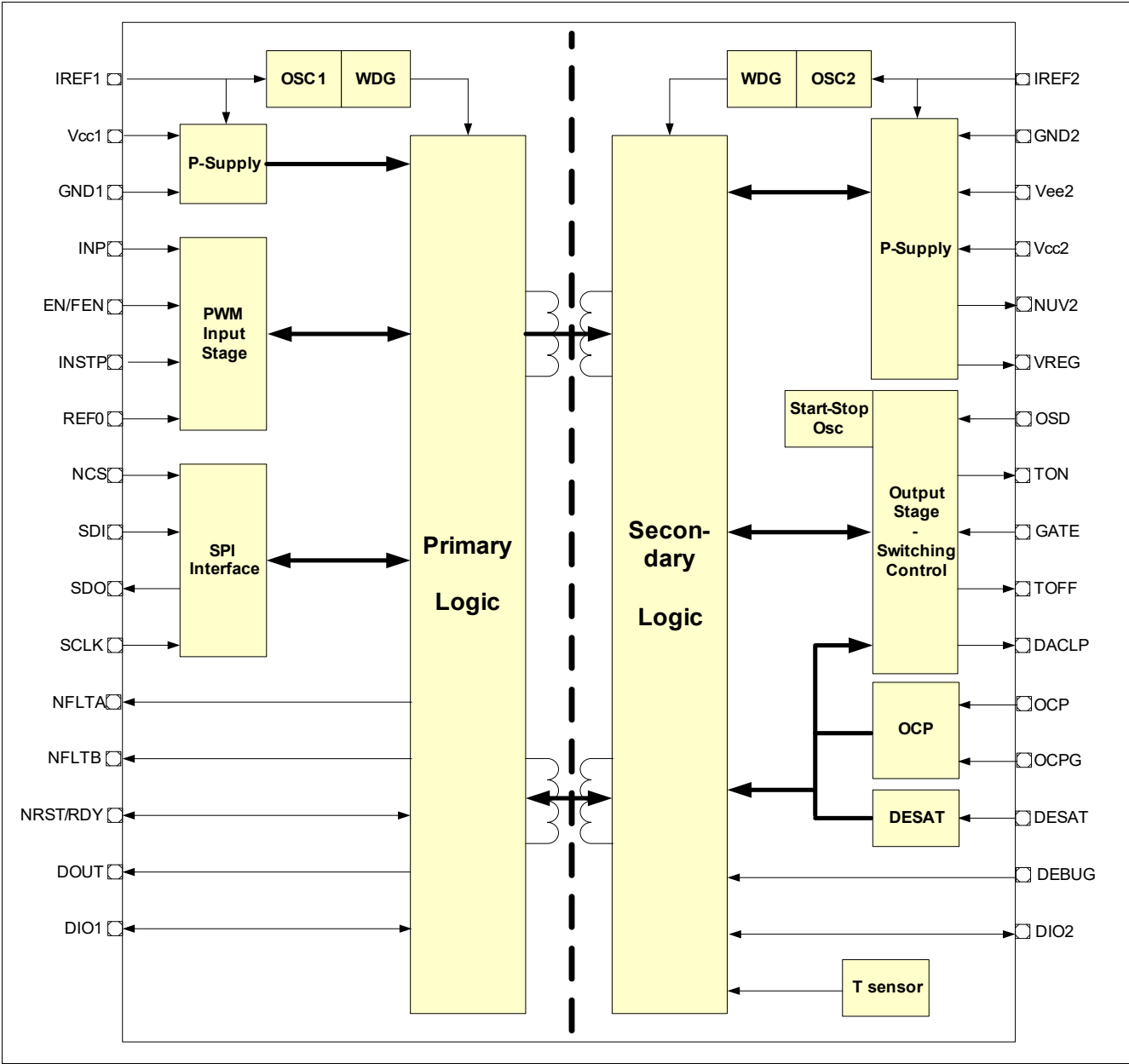
Figure 2 Block Diagram
