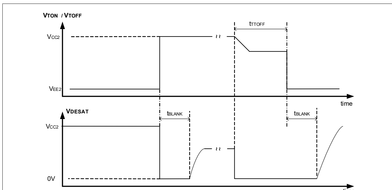
Figure 20 DESAT Operation
