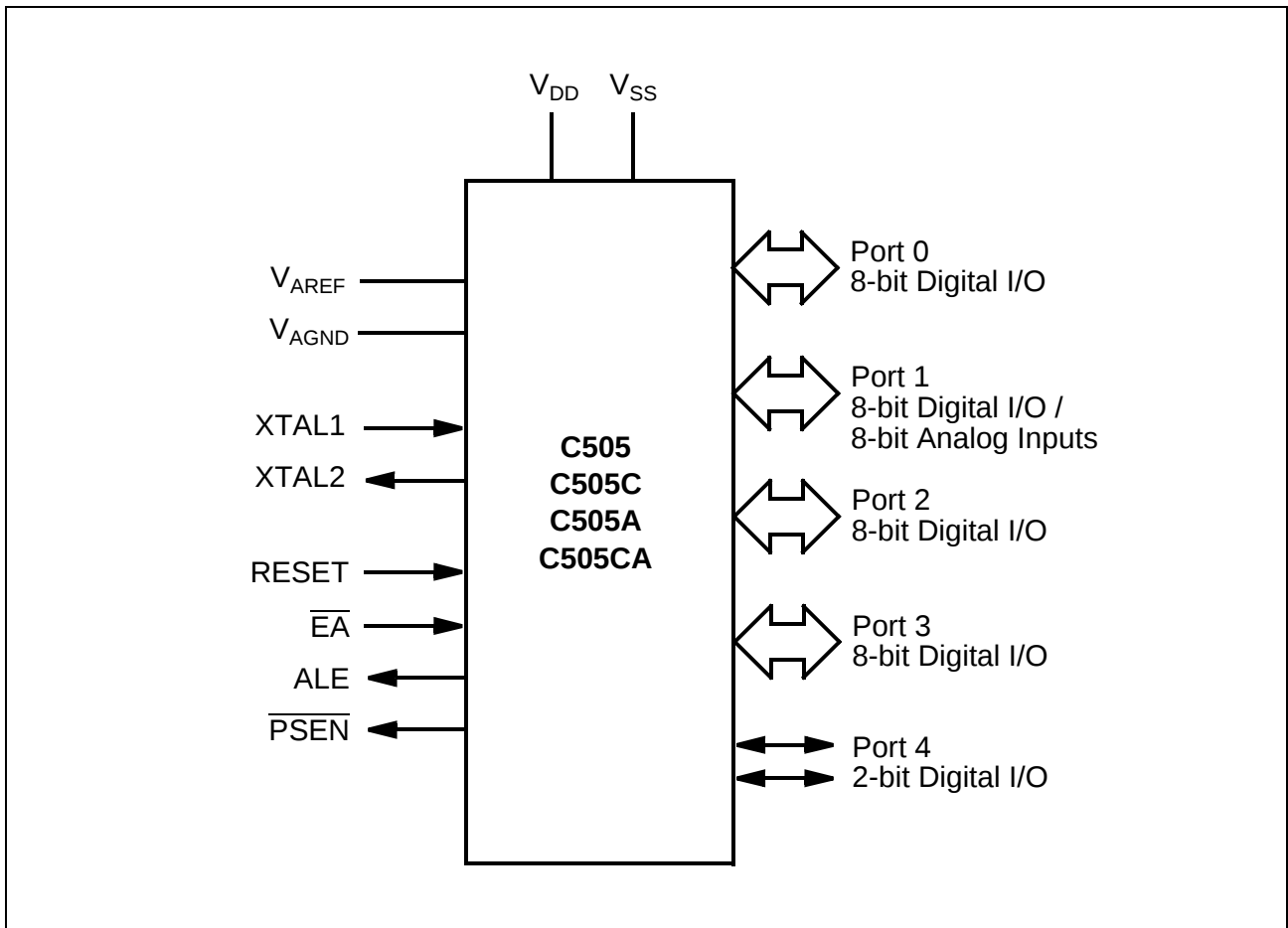
Figure 2 Logic Symbol
