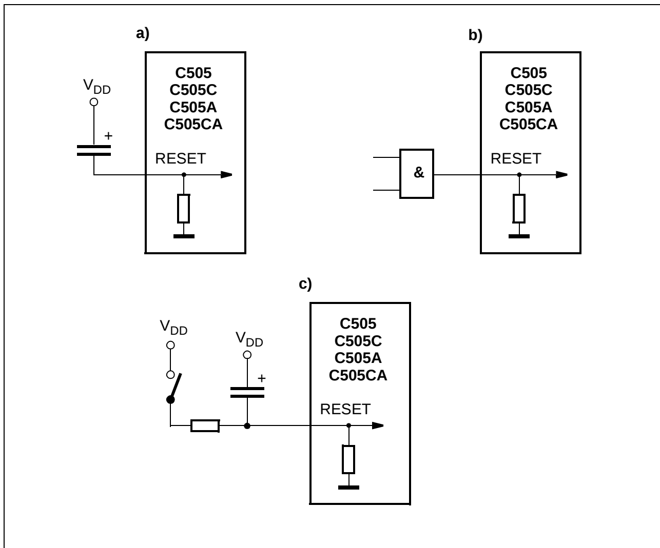
Figure 6 Reset Circuitries
