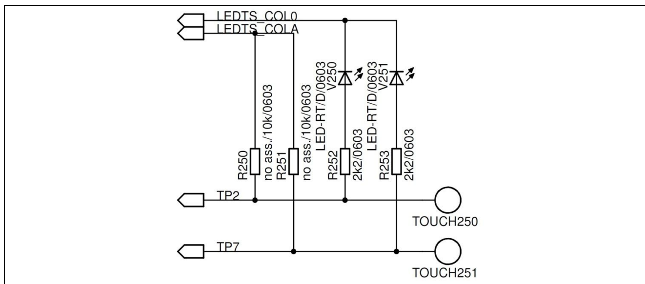
Figure 4 Touch Buttons
